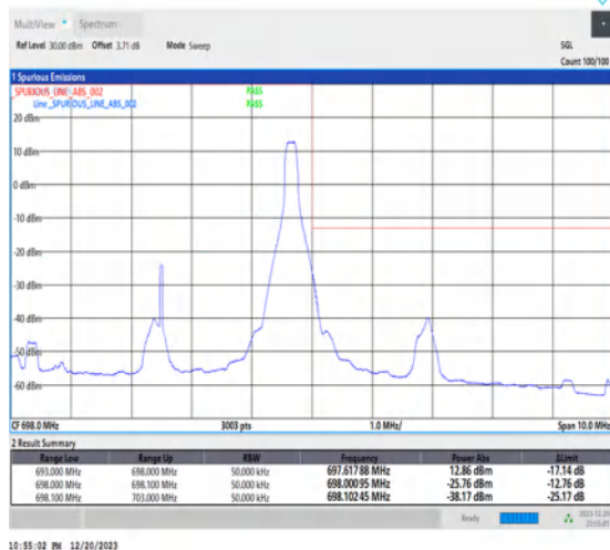
1-N71-15-5-H-5-CP-QPSK-Edge_1RB_Right-1@24-Ant7-1--PASS-see graph
