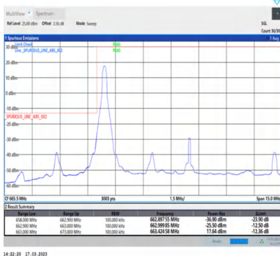
1-N71-PC3-15-10-L-4-CP-QPSK-Edge_1RB_Left-1@0-Ant7-1--PASS-see graph
