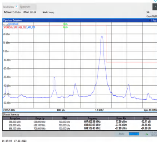
1-N71-PC3-15-10-H-5-CP-QPSK-Edge_1RB_Right-1@51-Ant7-1--PASS-see graph
