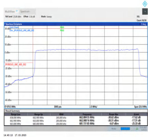
1-N71-PC3-15-20-L-3-DFT-PI2BPSK-Outer_Full-100@0-Ant7-1--PASS-see graph
