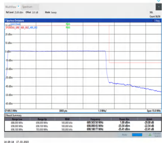
1-N71-PC3-15-10-H-6-CP-QPSK-Outer_Full-52@0-Ant7-1--PASS-see graph
