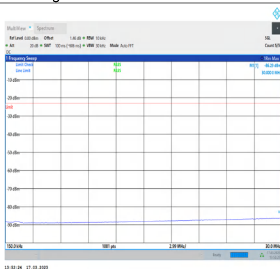
1-N71-PC3-15-20-H-1-DFT-PI2BPSK- Inner_1RB_Left-1@1-0.15-30-Ant7-30.00--86.29--23- PASS
