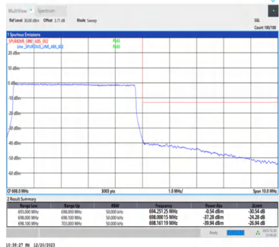
1-N71-15-5-H-6-CP-QPSK-Outer_Full-25@0-Ant7-1--PASS-see graph
