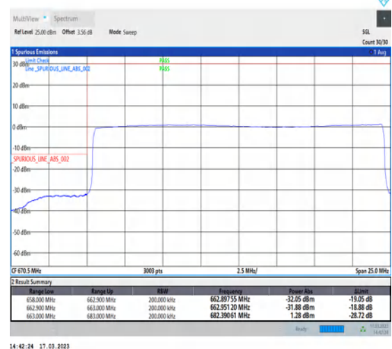
1-N71-PC3-15-20-L-6-CP-QPSK-Outer_Full-106@0-Ant7-1--PASS-see graph
