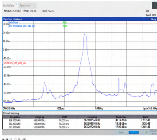
1-N71-PC3-15-5-L-1-DFT-PI2BPSK-Edge_1RB_Left-1@0-Ant7-1--PASS-see graph
