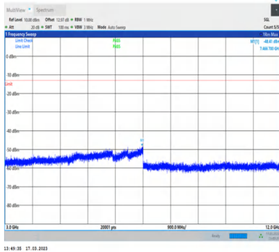
1-N71-PC3-15-20-L-1-DFT-PI2BPSK- Inner_1RB_Left-1@1-3000-12000-Ant7-7466.70-- 48.41--13-PASS
