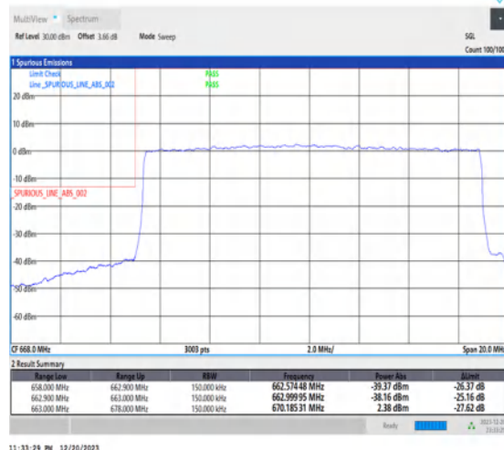
1-N71-15-15-L-3-DFT-PI2BPSK-Outer_Full-75@0-Ant7-1--PASS-see graph
