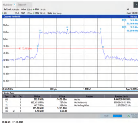
1-N71-PC3-15-5-L-1-DFT-QPSK-Outer_Full-25@0- Ant7-4.467-4.790-≤5-PASS
