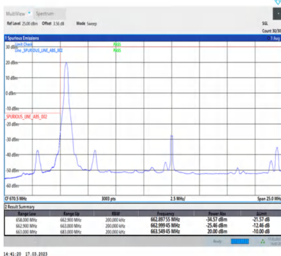
1-N71-PC3-15-20-L-4-CP-QPSK-Edge_1RB_Left-1@0-Ant7-1--PASS-see graph
