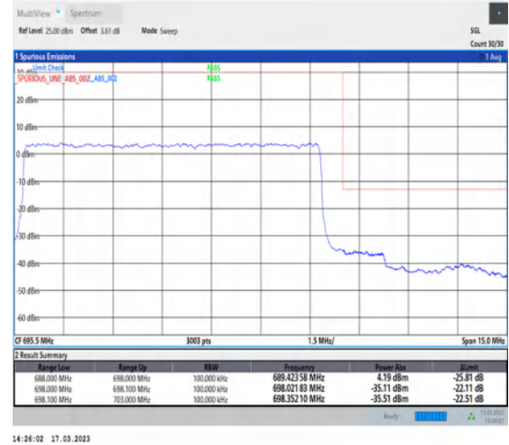
1-N71-PC3-15-10-H-3-DFT-PI2BPSK-Outer_Full-50@0-Ant7-1--PASS-see graph
