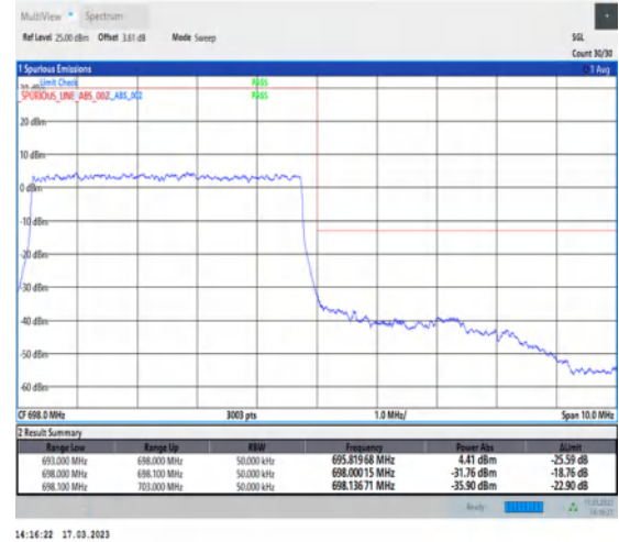
1-N71-PC3-15-5-H-3-DFT-PI2BPSK-Outer_Full-25@0-Ant7-1--PASS-see graph
