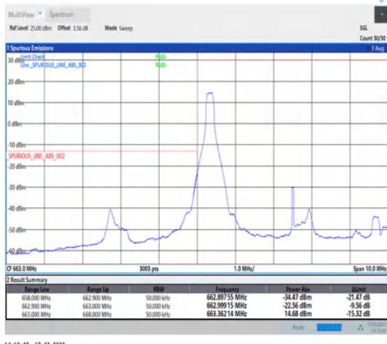
1-N71-PC3-15-5-L-4-CP-QPSK-Edge_1RB_Left-1@0-Ant7-1--PASS-see graph
