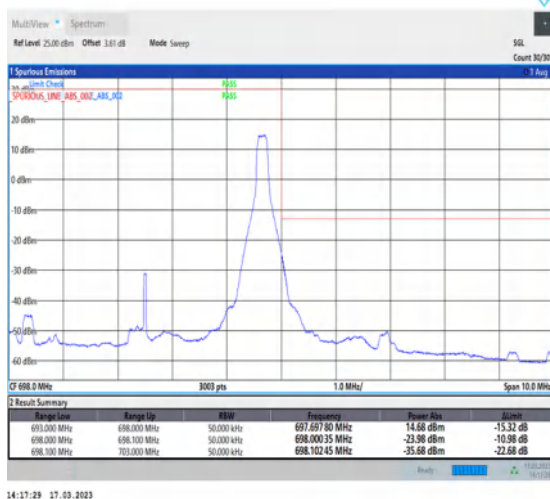
1-N71-PC3-15-5-H-5-CP-QPSK-Edge_1RB_Right-1@24-Ant7-1--PASS-see graph
