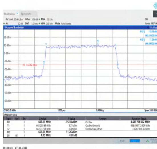
1-N71-PC3-15-5-L-4-DFT-64QAM-Outer_Full-25@0- Ant7-4.462-4.750-≤5-PASS
