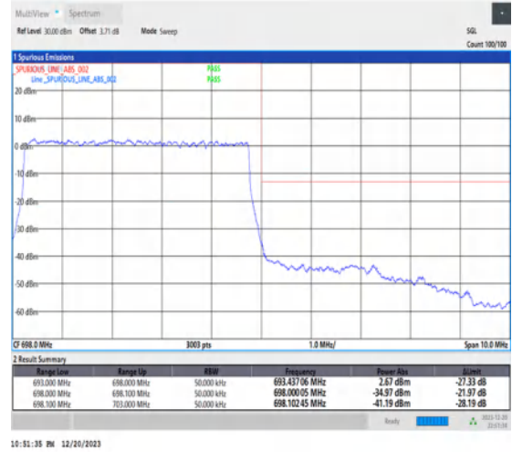
1-N71-15-5-H-3-DFT-PI2BPSK-Outer_Full-25@0-Ant7-1--PASS-see graph
