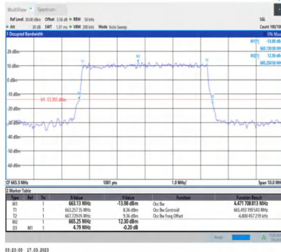
1-N71-PC3-15-5-L-2-DFT-PI2BPSK-Outer_Full- 25@0-Ant7-4.472-4.790-≤5-PASS
