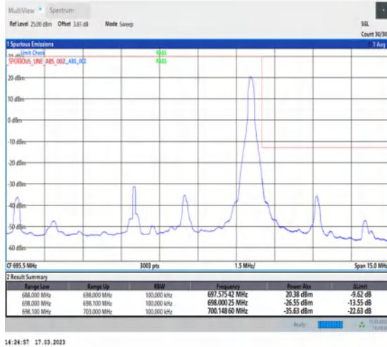
1-N71-PC3-15-10-H-2-DFT-PI2BPSK-Edge_1RB_Right-1@51-Ant7-1--PASS-see graph
