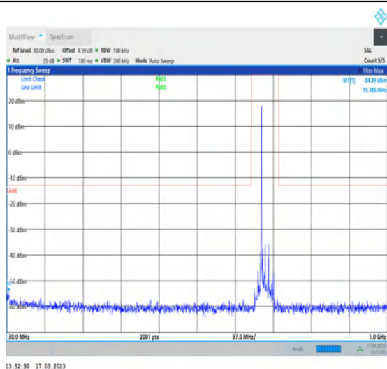
1-N71-PC3-15-20-H-1-DFT-PI2BPSK- Inner_1RB_Left-1@1-30-1000-Ant7-35.34--54.39-- 13-PASS
