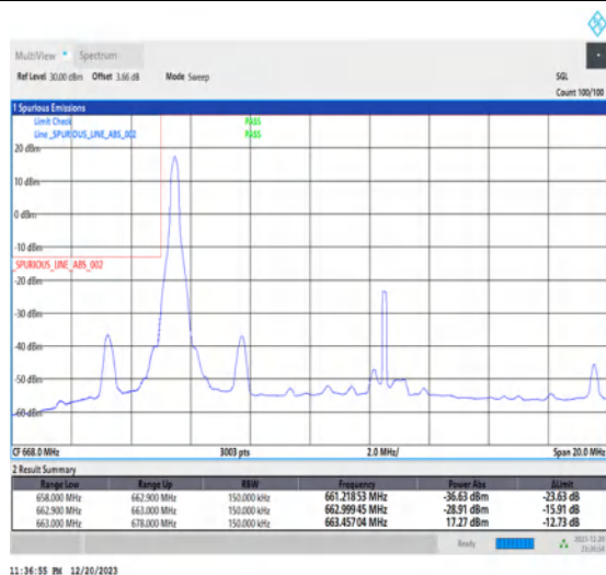
1-N71-15-15-L-4-CP-QPSK-Edge_1RB_Left-1@0-Ant7-1--PASS-see graph
