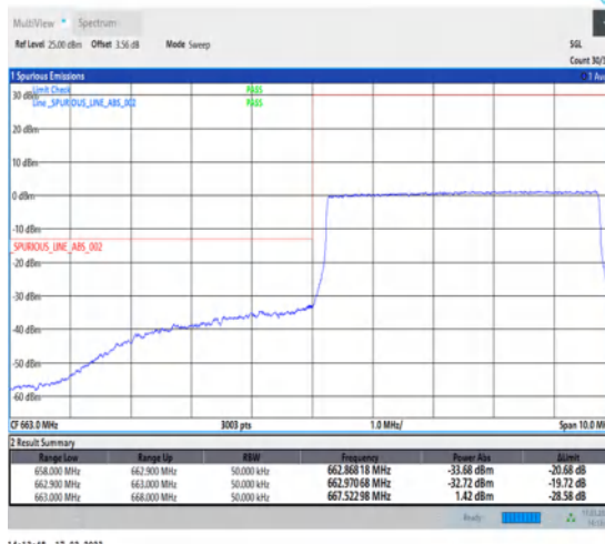
1-N71-PC3-15-5-L-6-CP-QPSK-Outer_Full-25@0-Ant7-1--PASS-see graph
