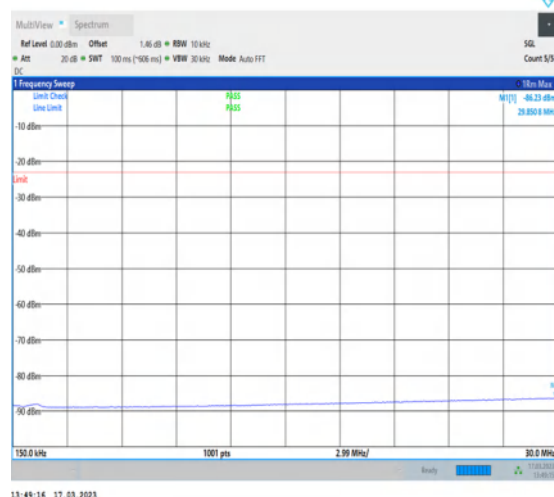
1-N71-PC3-15-20-L-1-DFT-PI2BPSK- Inner_1RB_Left-1@1-0.15-30-Ant7-29.85--86.23--23- PASS
