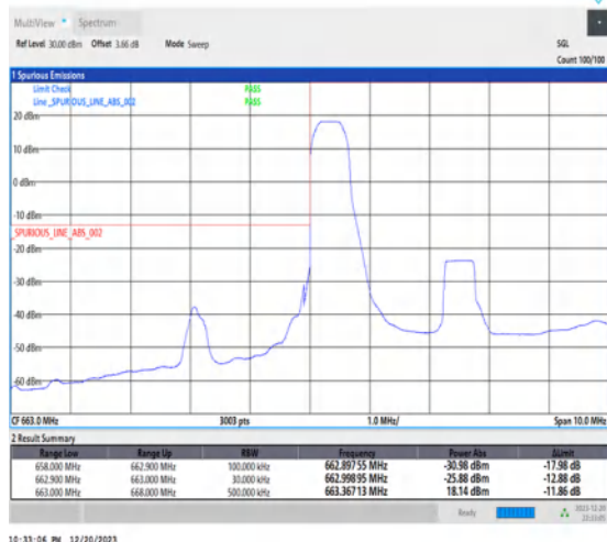
1-N71-15-5-L-4-CP-QPSK-Edge_1RB_Left-1@0-Ant7-1--PASS-see graph
