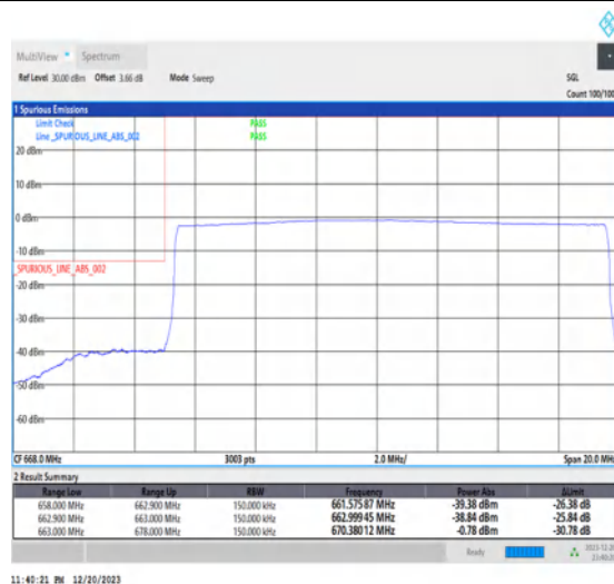
1-N71-15-15-L-6-CP-QPSK-Outer_Full-79@0-Ant7-1--PASS-see graph
