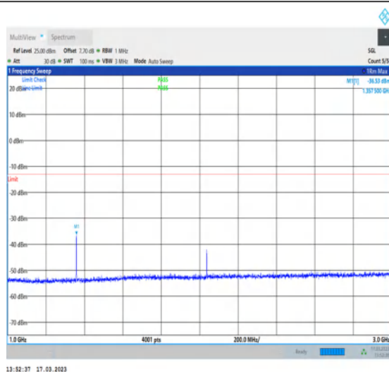
1-N71-PC3-15-20-H-1-DFT-PI2BPSK- Inner_1RB_Left-1@1-1000-3000-Ant7-1357.50-- 36.53--13-PASS
