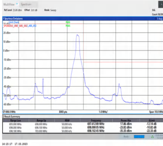
1-N71-PC3-15-5-H-2-DFT-PI2BPSK-Edge_1RB_Right-1@24-Ant7-1--PASS-see graph
