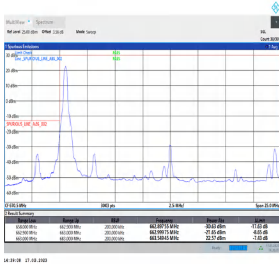
1-N71-PC3-15-20-L-1-DFT-PI2BPSK-Edge_1RB_Left-1@0-Ant7-1--PASS-see graph
