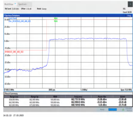
1-N71-PC3-15-10-L-3-DFT-PI2BPSK-Outer_Full-50@0-Ant7-1--PASS-see graph
