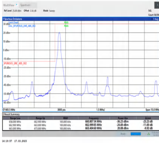
1-N71-PC3-15-10-L-1-DFT-PI2BPSK-Edge_1RB_Left-1@0-Ant7-1--PASS-see graph
