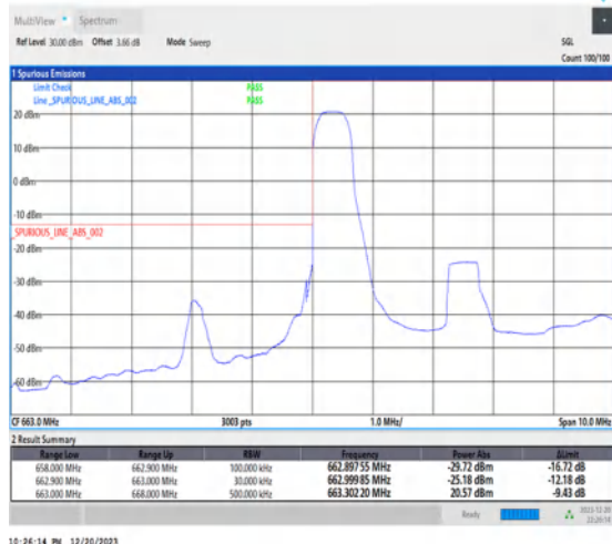
1-N71-15-5-L-1-DFT-PI2BPSK-Edge_1RB_Left-1@0-Ant7-1--PASS-see graph
