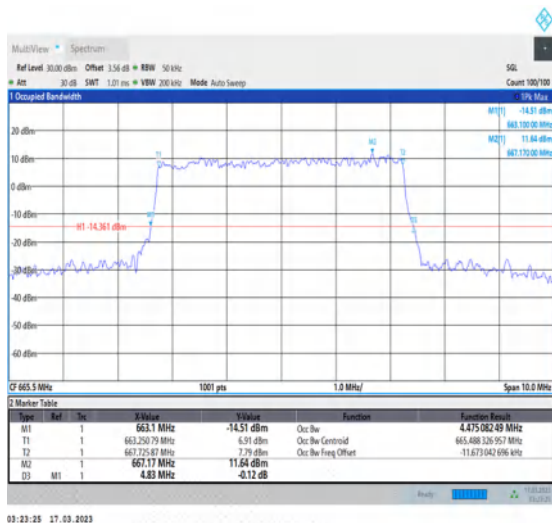
1-N71-PC3-15-5-L-3-DFT-16QAM-Outer_Full-25@0- Ant7-4.475-4.830-≤5-PASS
