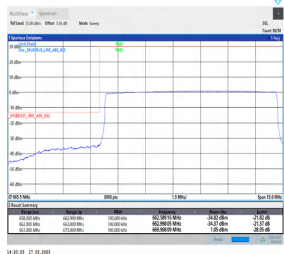
1-N71-PC3-15-10-L-6-CP-QPSK-Outer_Full-52@0-Ant7-1--PASS-see graph
