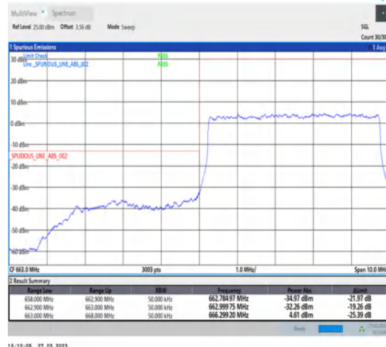
1-N71-PC3-15-5-L-3-DFT-PI2BPSK-Outer_Full-25@0-Ant7-1--PASS-see graph
