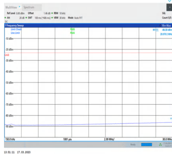
1-N71-PC3-15-20-M-1-DFT-PI2BPSK- Inner_1RB_Left-1@1-0.15-30-Ant7-29.97--86.30--23- PASS
