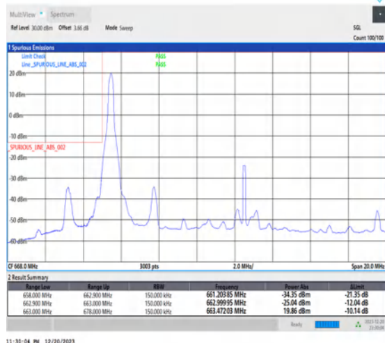
1-N71-15-15-L-1-DFT-PI2BPSK-Edge_1RB_Left-1@0-Ant7-1--PASS-see graph
