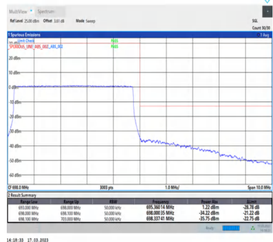
1-N71-PC3-15-5-H-6-CP-QPSK-Outer_Full-25@0-Ant7-1--PASS-see graph
