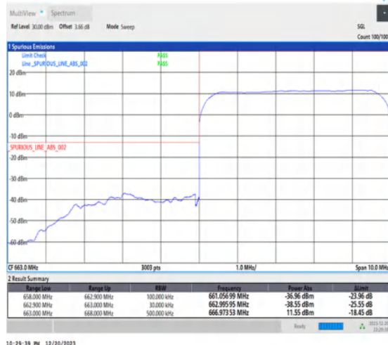
1-N71-15-5-L-3-DFT-PI2BPSK-Outer_Full-25@0-Ant7-1--PASS-see graph
