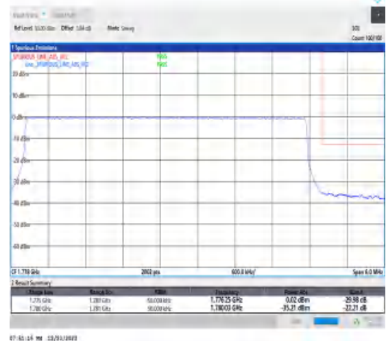
1-N66-15-5-H-6-CP-QPSK-Outer_Full-25@0-Ant1-1-seegraph-PASS-see graph
