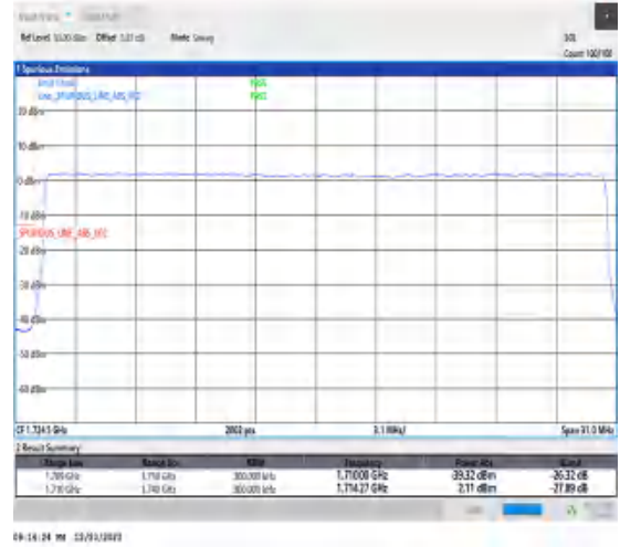
1-N66-15-30-L-3-DFT-PI2BPSK-Outer_Full-160@0-Ant1-1-seegraph-PASS-see graph
