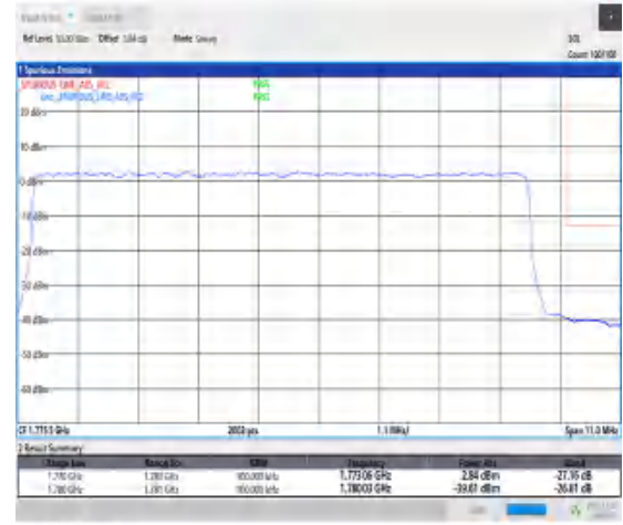
1-N66-15-10-H-3-DFT-PI2BPSK-Outer_Full-50@0-Ant1-1-seegraph-PASS-see graph
