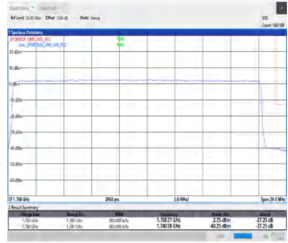
1-N66-15-25-H-3-DFT-PI2BPSK-Outer_Full-128@0-Ant1-1-seegraph-PASS-see graph
