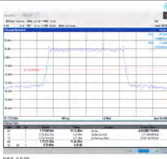
1-N66-PC3-15-5-L-4-DFT-64QAM-Outer_Full-25@0- Ant1-4.454-4.790≤5-PASS
