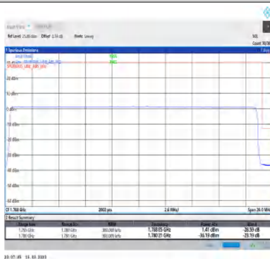
1-N66-PC3-15-25-H-6-CP-QPSK-Outer_Full-133@0-Ant1-1-seegraph-PASS-see graph
