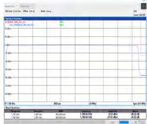
1-N66-15-25-H-6-CP-QPSK-Outer_Full-133@0-Ant1-1-seegraph-PASS-see graph
