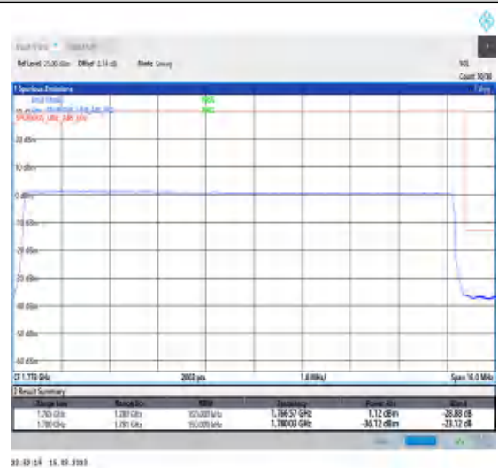
1-N66-PC3-15-15-H-6-CP-QPSK-Outer_Full-79@0-Ant1-1-seegraph-PASS-see graph
