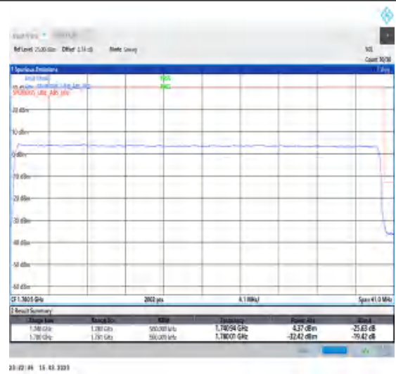
1-N66-PC3-15-40-H-3-DFT-PI2BPSK-Outer_Full-216@0-Ant1-1-seegraph-PASS-see graph
