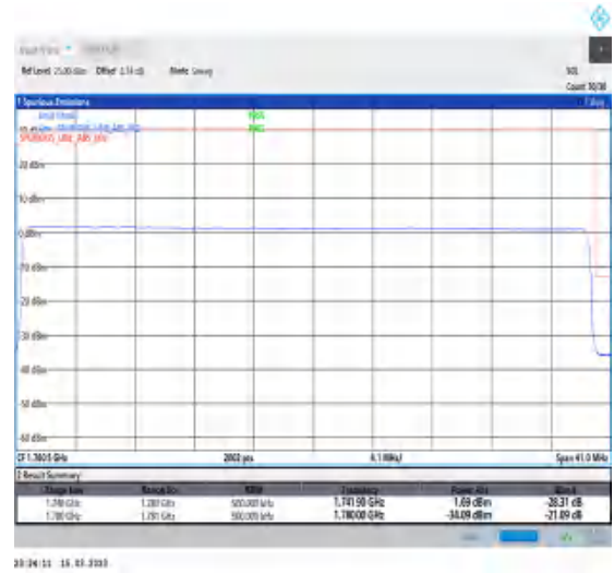
1-N66-PC3-15-40-H-6-CP-QPSK-Outer_Full-216@0-Ant1-1-seegraph-PASS-see graph
