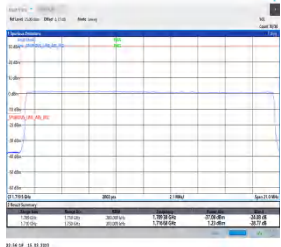
1-N66-PC3-15-20-L-6-CP-QPSK-Outer_Full-106@0-Ant1-1-seegraph-PASS-see graph
