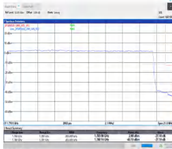
1-N66-15-20-H-3-DFT-PI2BPSK-Outer_Full-100@0-Ant1-1-seegraph-PASS-see graph
