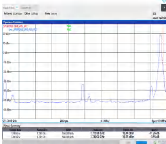
1-N66-15-40-H-5-CP-QPSK-Edge_1RB_Right-1@215-Ant1-1-seegraph-PASS-see graph
