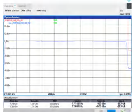
1-N66-15-40-H-6-CP-QPSK-Outer_Full-216@0-Ant1-1-seegraph-PASS-see graph
