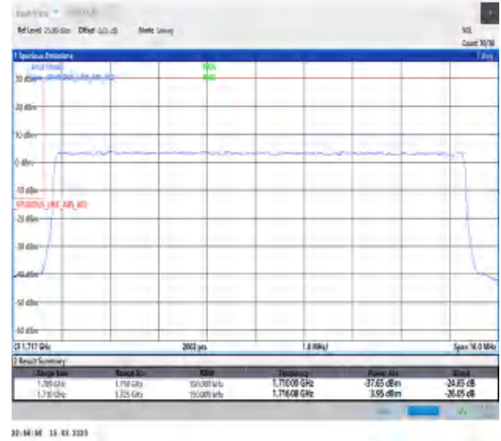
1-N66-PC3-15-15-L-3-DFT-PI2BPSK-Outer_Full-75@0-Ant1-1-seegraph-PASS-see graph
