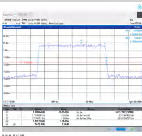
1-N66-PC3-15-15-L-9-CP-256QAM-Outer_Full- 79@0-Ant1-14.118-14.760-≤15-PASS
