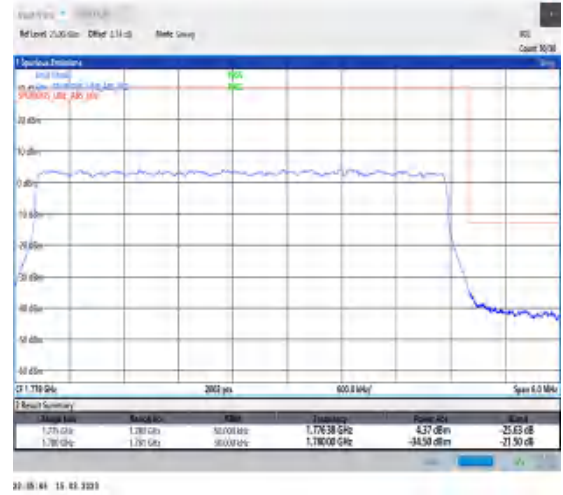
1-N66-PC3-15-5-H-3-DFT-PI2BPSK-Outer_Full-25@0-Ant1-1-seegraph-PASS-see graph
