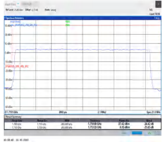
1-N66-PC3-15-20-L-3-DFT-PI2BPSK-Outer_Full-100@0-Ant1-1-seegraph-PASS-see graph
