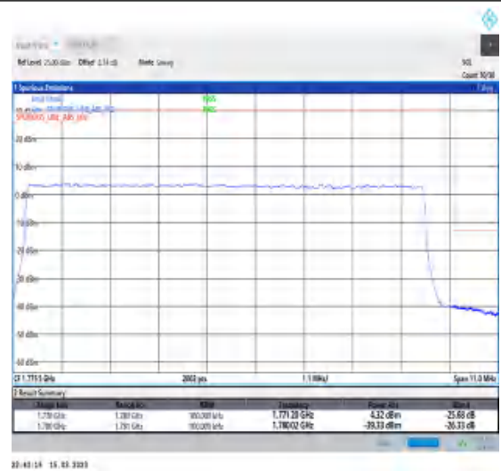
1-N66-PC3-15-10-H-3-DFT-PI2BPSK-Outer_Full-50@0-Ant1-1-seegraph-PASS-see graph
