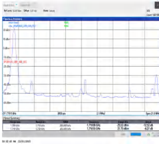
1-N66-15-20-L-1-DFT-PI2BPSK-Edge_1RB_Left-1@0-Ant1-1-seegraph-PASS-see graph
