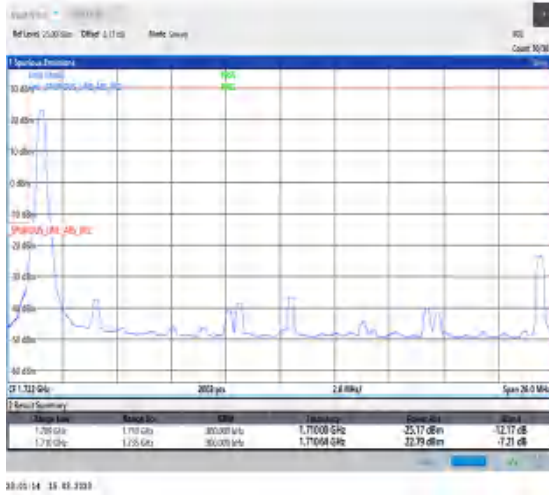
1-N66-PC3-15-25-L-1-DFT-PI2BPSK-Edge_1RB_Left-1@0-Ant1-1-seegraph-PASS-see graph
