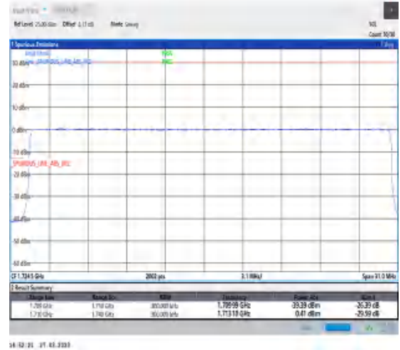
1-N66-PC3-15-30-L-3-DFT-PI2BPSK-Outer_Full-160@0-Ant1-1-seegraph-PASS-see graph
