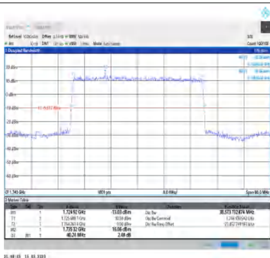
1-N66-PC3-15-40-M-2-DFT-PI2BPSK-Outer_Full- 216@0-Ant1-38.574-40.240-≤40-PASS
