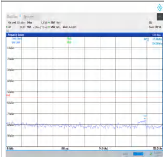
1-N41-30-100-M-1-DFT-PI2BPSK- Inner_1RB_Left-1@1-0.009-0.15-Ant1-0.13-- 75.68--55-PASS
