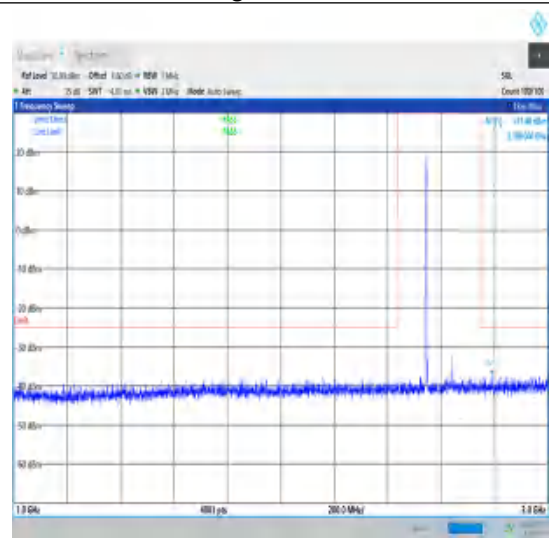
1-N41-30-100-M-1-DFT-PI2BPSK- Inner_1RB_Left-1@1-1000-3000-Ant1- 2959.50--37.48--25-PASS
