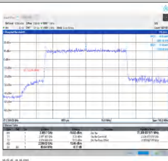
1-N41-30-80-L-6-CP-QPSK-Outer_Full-217@0- Ant1-77.3-80.640-≤80-PASS
