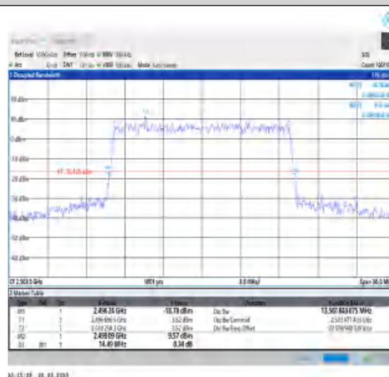
1-N41-30-15-L-9-CP-256QAM-Outer_Full-38@0- Ant1-13.562-14.490≤15-PASS
