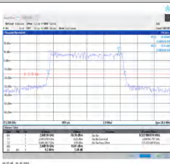
1-N41-30-10-H-5-DFT-256QAM-Outer_Full-24@0- Ant1-8.528-9.200-≤10-PASS
