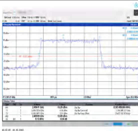
1-N41-30-10-L-3-DFT-16QAM-Outer_Full-24@0- Ant1-8.565-9.140≤10-PASS
