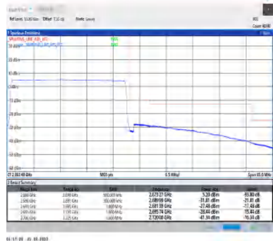
1-N41-30-30-H-6-CP-QPSK-Outer_Full-78@0-Ant1-1--PASS-see graph
