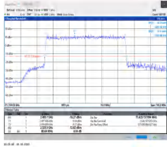
1-N41-30-80-L-9-CP-256QAM-Outer_Full-217@0-Ant1-77.424-80.640-≤80-PASS
