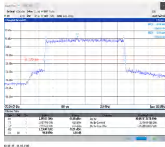
1-N41-30-100-L-5-DFT-256QAM-Outer_Full-270@0-Ant1-96.093-99.800-≤100-PASS
