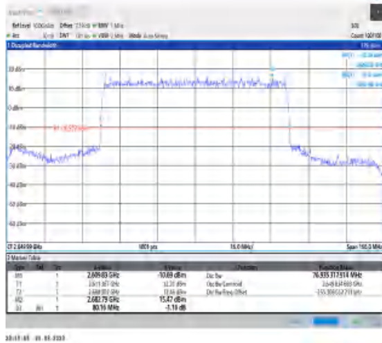
1-N41-30-80-H-2-DFT-PI2BPSK-Outer_Full-216@0-Ant1-76.935-80.160-≤80-PASS
