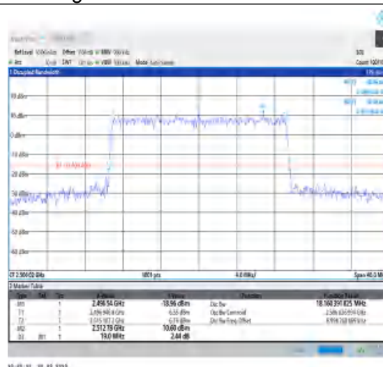
1-N41-30-20-L-8-CP-64QAM-Outer_Full-51@0-Ant1- 18.16-19.000-≤20-PASS
