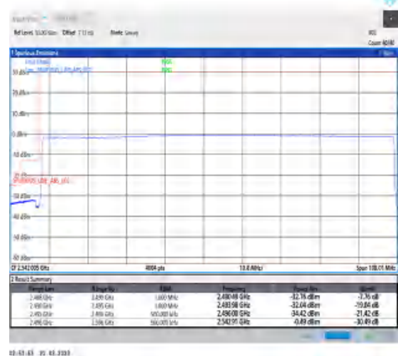
1-N41-30-100-L-6-CP-QPSK-Outer_Full-273@0-Ant1-1--PASS-see graph
