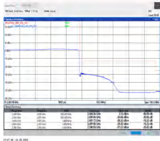
1-N41-30-90-H-6-CP-QPSK-Outer_Full-245@0-Ant1-1--PASS-see graph
