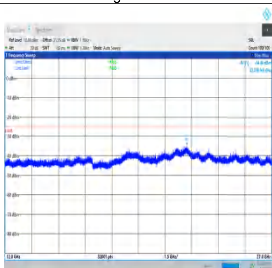
1-N41-30-100-L-1-DFT-PI2BPSK- Inner_1RB_Left-1@1-12000-27000-Ant1- 21680.00--34.86--25-PASS
