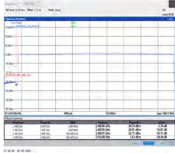
1-N41-30-100-L-6-CP-QPSK-Outer_Full-273@0-Ant1-1--PASS-see graph
