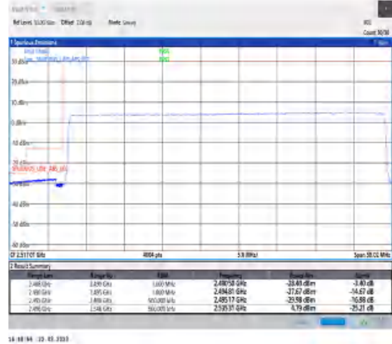
1-N41-30-50-L-6-CP-QPSK-Outer_Full-133@0-Ant1-1--PASS-see graph
