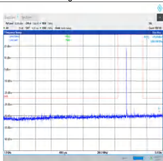
1-N41-30-100-M-1-DFT-PI2BPSK- Inner_1RB_Left-1@1-1000-3000-Ant1- 2959.50--37.08--25-PASS
