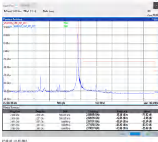
1-N41-30-90-H-5-CP-QPSK-Edge_1RB_Right-1@244-Ant1-1--PASS-see graph
