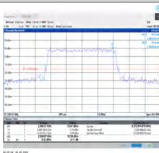
1-N41-30-10-L-8-CP-64QAM-Outer_Full-24@0-Ant1- 8.572-9.320≤10-PASS
