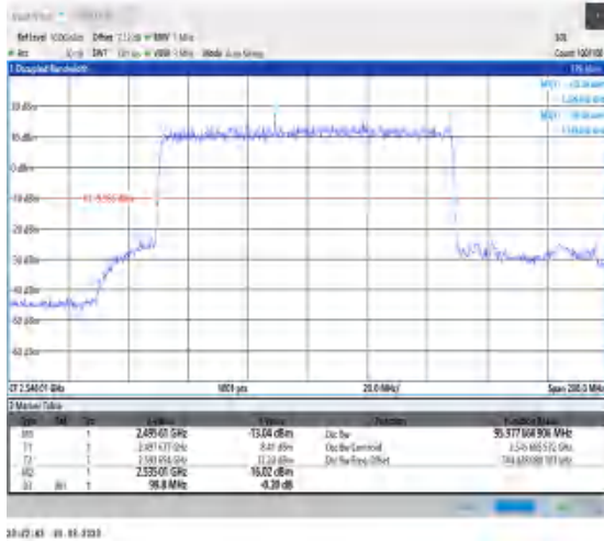
1-N41-30-100-L-2-DFT-PI2BPSK-Outer_Full-270@0-Ant1-95.978-99.800-≤100-PASS
