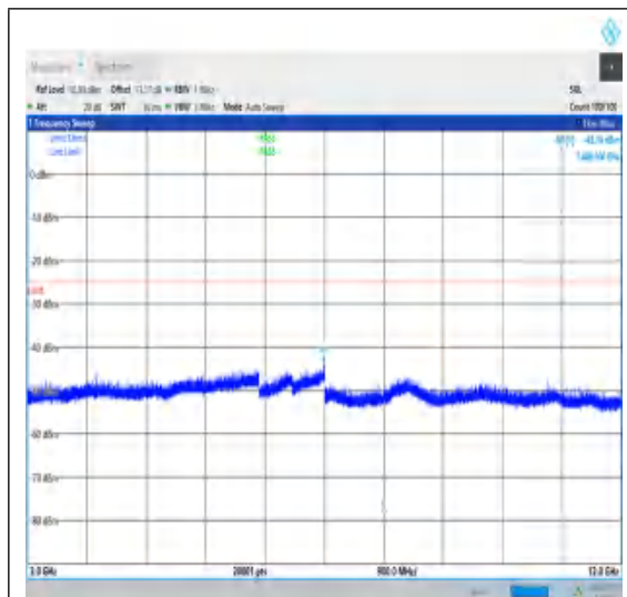
1-N41-30-100-L-1-DFT-PI2BPSK- Inner_1RB_Left-1@1-3000-12000-Ant1- 7493.25--43.76--25-PASS
