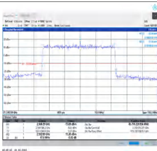
1-N41-30-50-M-1-DFT-QPSK-Outer_Full-128@0- Ant1-45.776-47.600-≤50-PASS
