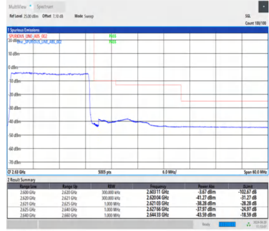
1-N38-30-20-H-3-DFT-PI2BPSK-Outer_Full-50@0-Ant1-1--PASS-see graph
