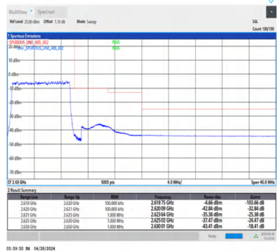
1-N38-30-10-H-3-DFT-PI2BPSK-Outer_Full-24@0-Ant1-1--PASS-see graph
