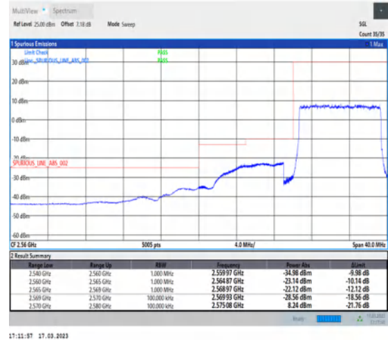
1-N38-30-10-L-3-DFT-PI2BPSK-Outer_Full-24@0-Ant1-1--PASS-see graph
