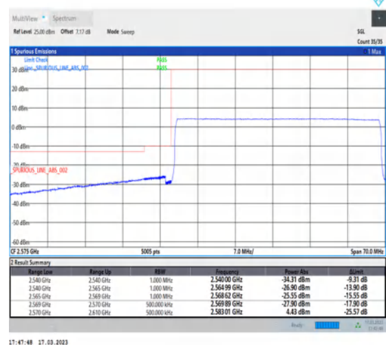
1-N38-30-40-L-6-CP-QPSK-Outer_Full-106@0-Ant1-1--PASS-see graph
