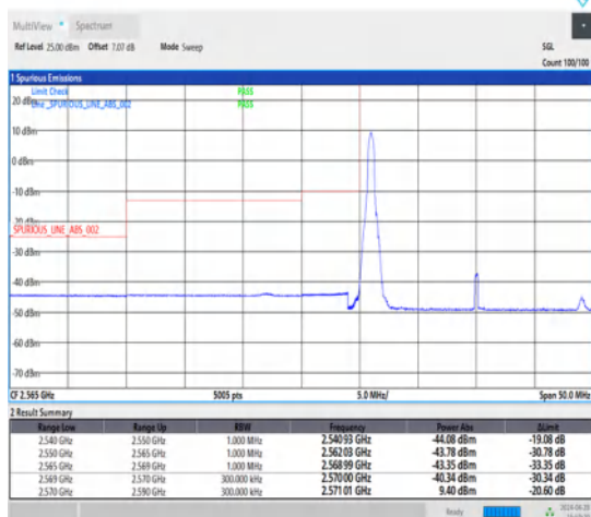
1-N38-30-20-L-4-CP-QPSK-Edge_1RB_Left-1@0-Ant1-1--PASS-see graph
