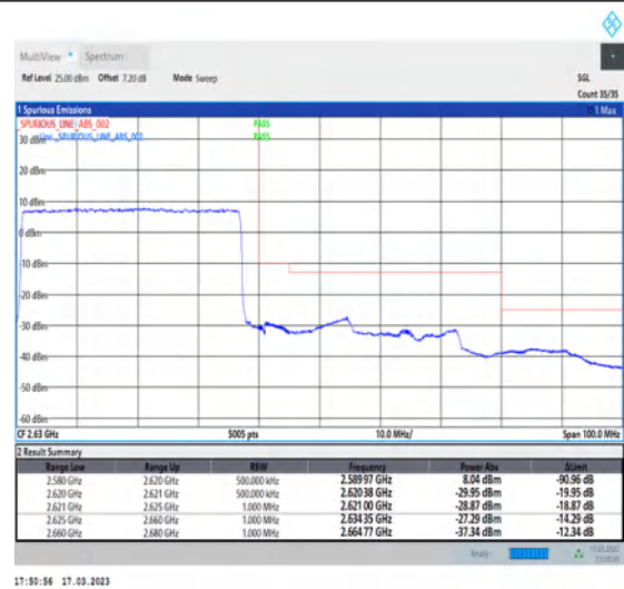
1-N38-30-40-H-3-DFT-PI2BPSK-Outer_Full-100@0-Ant1-1--PASS-see graph
