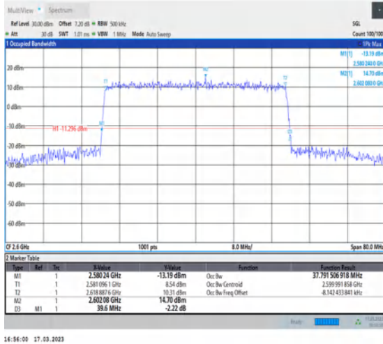
1-N38-30-40-H-6-CP-QPSK-Outer_Full-106@0-Ant1-37.792-39.600-≤40-PASS
