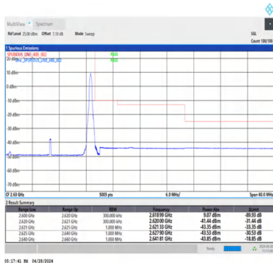
1-N38-30-20-H-5-CP-QPSK-Edge_1RB_Right-1@50-Ant1-1--PASS-see graph
