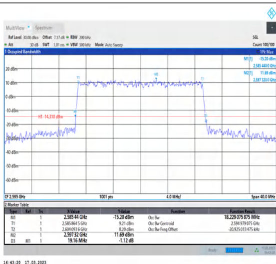
1-N38-30-20-M-6-CP-QPSK-Outer_Full-51@0-Ant1-18.229-19.160-≤20-PASS
