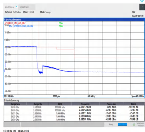
1-N38-30-10-H-6-CP-QPSK-Outer_Full-24@0-Ant1-1--PASS-see graph
