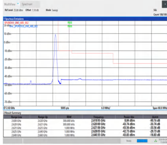
1-N38-30-20-H-2-DFT-PI2BPSK-Edge_1RB_Right-1@50-Ant1-1--PASS-see graph
