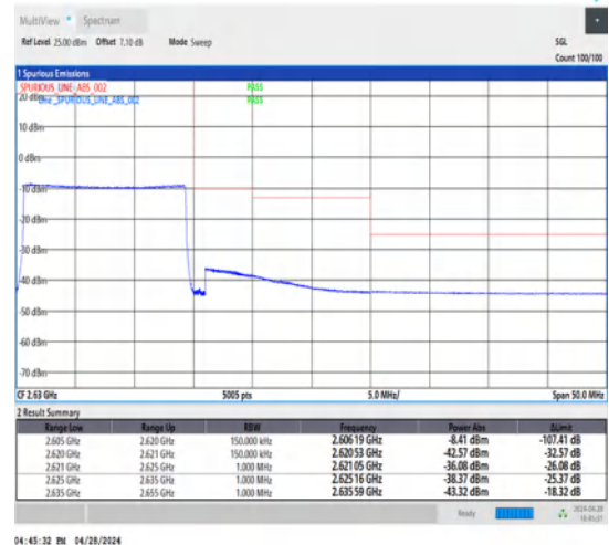
1-N38-30-15-H-6-CP-QPSK-Outer_Full-38@0-Ant1-1--PASS-see graph
