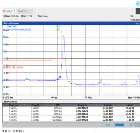
1-N38-30-40-L-1-DFT-PI2BPSK-Edge_1RB_Left-1@0-Ant1-1--PASS-see graph
