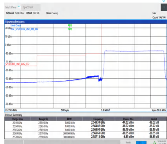
1-N38-30-20-L-6-CP-QPSK-Outer_Full-51@0-Ant1-1--PASS-see graph
