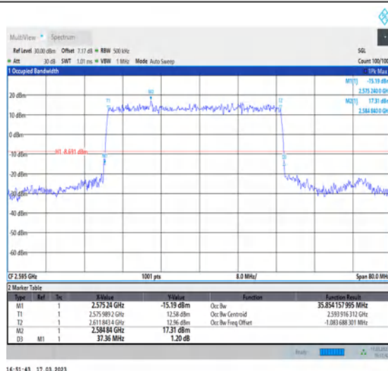
1-N38-30-40-M-2-DFT-PI2BPSK-Outer_Full-100@0-Ant1-35.854-37.360-≤40-PASS
