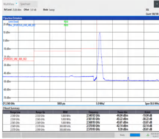
1-N38-30-20-L-1-DFT-PI2BPSK-Edge_1RB_Left-1@0-Ant1-1--PASS-see graph
