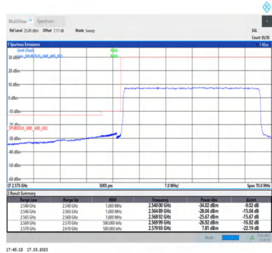
1-N38-30-40-L-3-DFT-PI2BPSK-Outer_Full-100@0-Ant1-1--PASS-see graph
