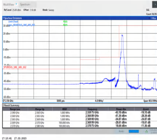
1-N38-30-10-L-1-DFT-PI2BPSK-Edge_1RB_Left-1@0-Ant1-1--PASS-see graph
