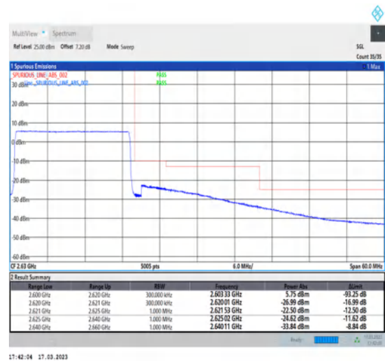
1-N38-30-20-H-6-CP-QPSK-Outer_Full-51@0-Ant1-1--PASS-see graph
