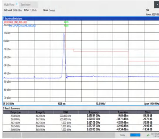
1-N38-30-40-H-2-DFT-PI2BPSK-Edge_1RB_Right-1@105-Ant1-1--PASS-see graph
