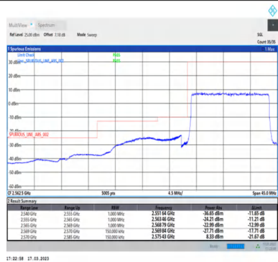
1-N38-30-15-L-3-DFT-PI2BPSK-Outer_Full-36@0-Ant1-1--PASS-see graph
