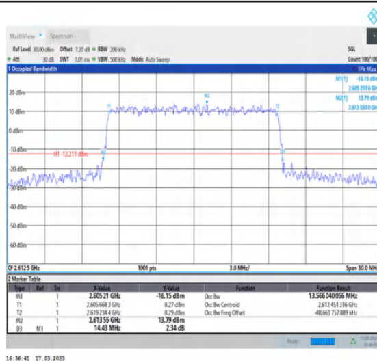
1-N38-30-15-H-7-CP-16QAM-Outer_Full-38@0-Ant1-13.566-14.430-≤15-PASS
