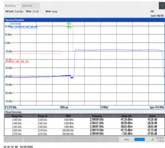
1-N38-30-40-L-6-CP-QPSK-Outer_Full-106@0-Ant1-1--PASS-see graph
