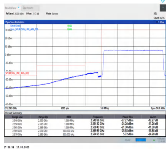
1-N38-30-20-L-6-CP-QPSK-Outer_Full-51@0-Ant1-1--PASS-see graph
