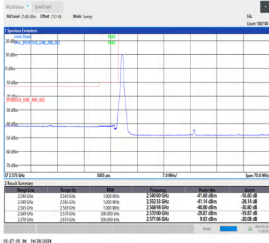
1-N38-30-40-L-1-DFT-PI2BPSK-Edge_1RB_Left-1@0-Ant1-1--PASS-see graph
