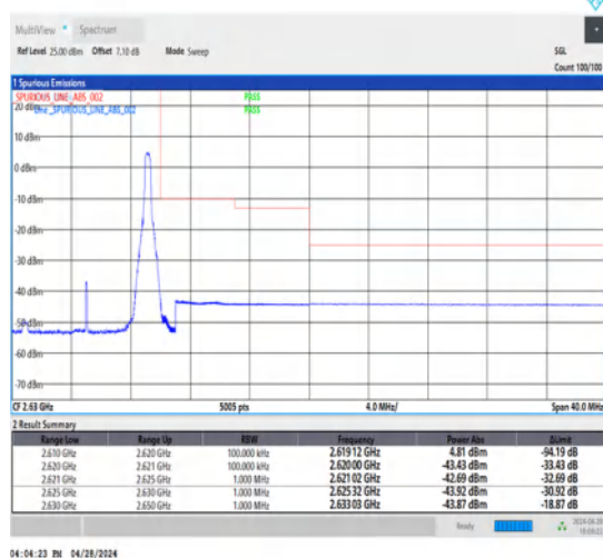
1-N38-30-10-H-5-CP-QPSK-Edge_1RB_Right-1@23-Ant1-1--PASS-see graph
