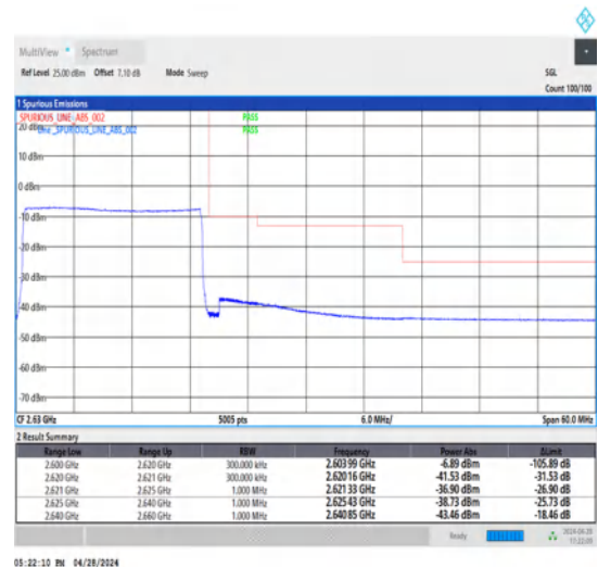
1-N38-30-20-H-6-CP-QPSK-Outer_Full-51@0-Ant1-1--PASS-see graph
