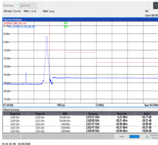
1-N38-30-15-H-5-CP-QPSK-Edge_1RB_Right-1@37-Ant1-1--PASS-see graph
