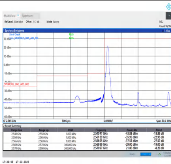
1-N38-30-20-L-1-DFT-PI2BPSK-Edge_1RB_Left-1@0-Ant1-1--PASS-see graph
