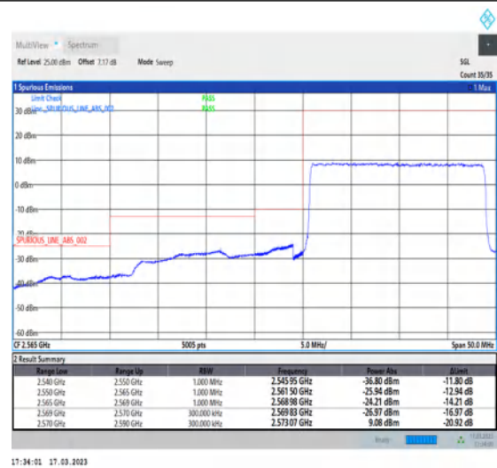
1-N38-30-20-L-3-DFT-PI2BPSK-Outer_Full-50@0-Ant1-1--PASS-see graph
