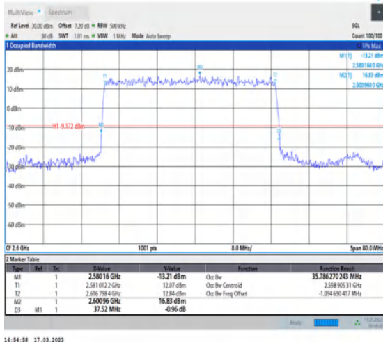
1-N38-30-40-H-2-DFT-PI2BPSK-Outer_Full-100@0-Ant1-35.786-37.520-≤40-PASS
