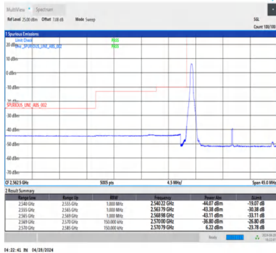
1-N38-30-15-L-4-CP-QPSK-Edge_1RB_Left-1@0-Ant1-1--PASS-see graph
