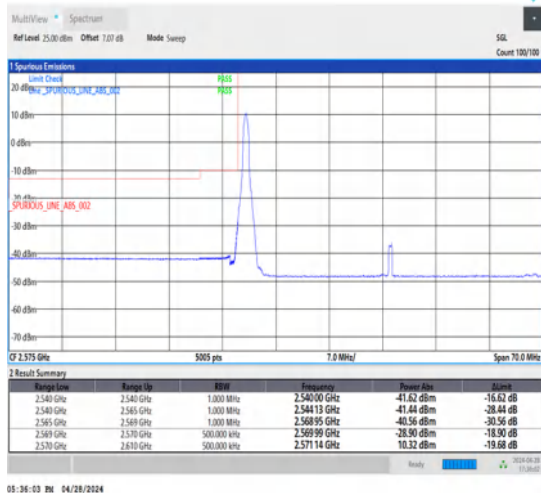
1-N38-30-40-L-4-CP-QPSK-Edge_1RB_Left-1@0-Ant1-1--PASS-see graph
