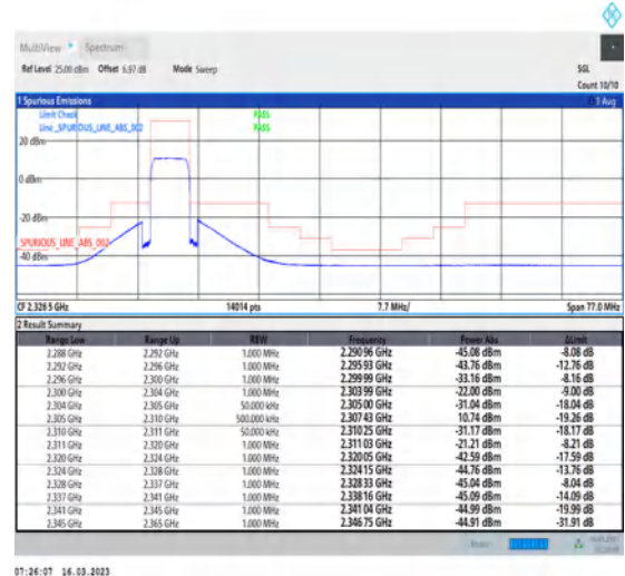
1-N30-PC3-15-5-L-6-CP-QPSK-Outer_Full-25@0-Ant1-1--PASS-see graph
