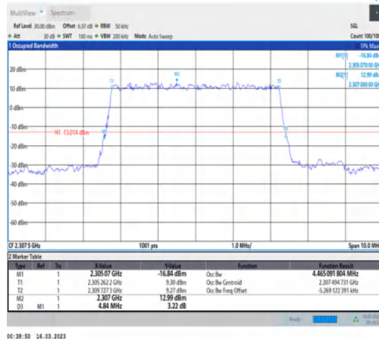
1-N30-PC3-15-5-L-2-DFT-PI2BPSK-Outer_Full- 25@0-Ant1-4.465-4.840-≤5-PASS
