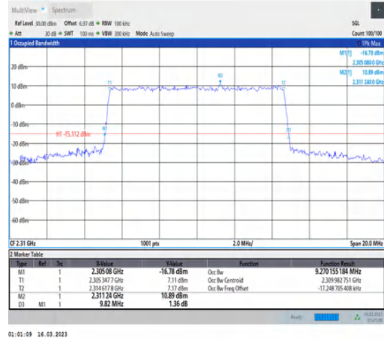
1-N30-PC3-15-10-L-7-CP-16QAM-Outer_Full-52@0-Ant1-9.27-9.820-≤10-PASS
