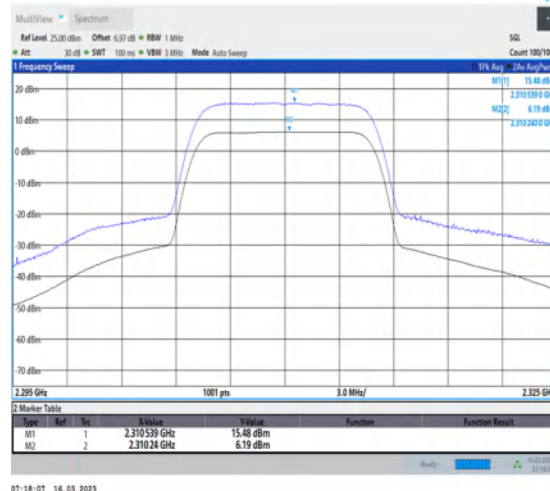
1-N30-PC3-15-10-M-2-CP-256QAM-Outer_Full-52@0-Ant1-9.29-100%-0.00-9.29-PASS-≤13
