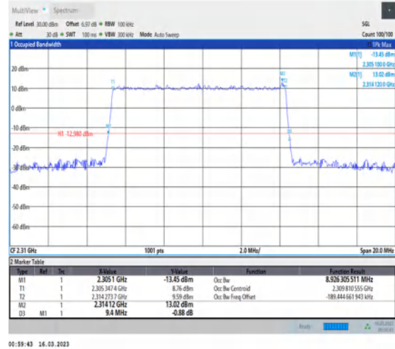
1-N30-PC3-15-10-L-3-DFT-16QAM-Outer_Full-50@0-Ant1-8.926-9.400-≤10-PASS
