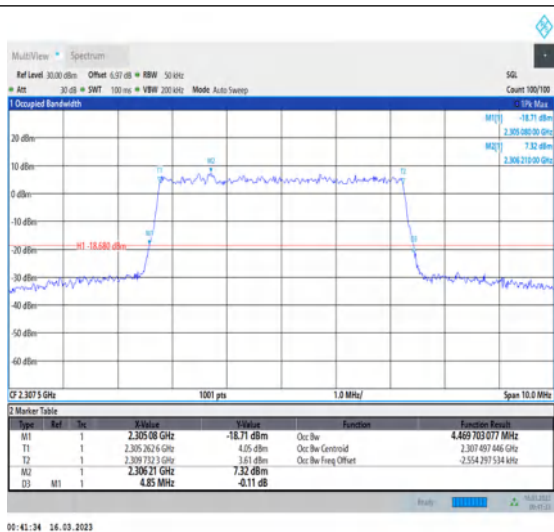
1-N30-PC3-15-5-L-9-CP-256QAM-Outer_Full-25@0-Ant1-4.47-4.850-≤5-PASS
