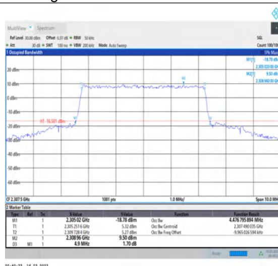
1-N30-PC3-15-5-L-6-CP-QPSK-Outer_Full-25@0-Ant1-4.477-4.900-≤5-PASS
