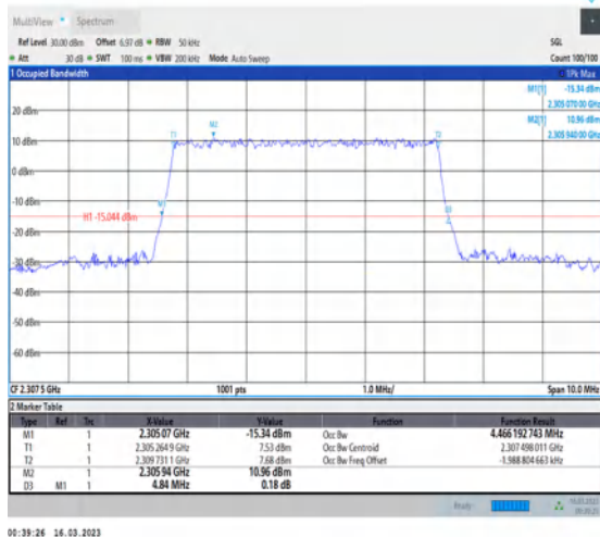
1-N30-PC3-15-5-L-3-DFT-16QAM-Outer_Full-25@0- Ant1-4.466-4.840-≤5-PASS
