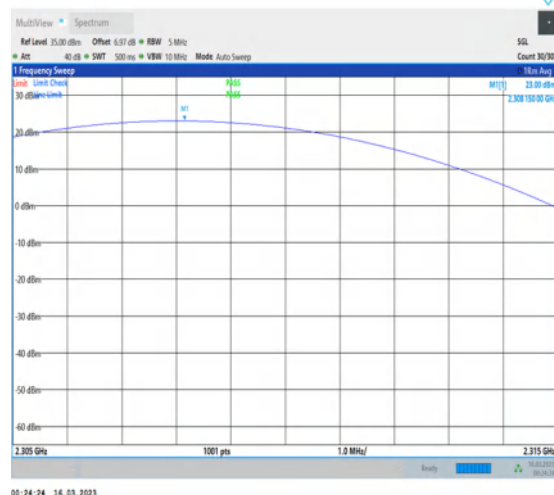
1-N30-PC3-15-5-M-1-DFT-PI2BPSK- Inner_1RB_Left-1@1-2305-2315-Ant1-2308.15- 23.00-99-PASS
