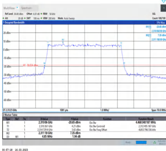
1-N30-PC3-15-5-H-9-CP-256QAM-Outer_Full-25@0-Ant1-4.468-4.850-≤5-PASS
