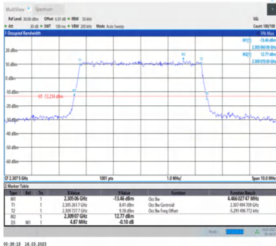
1-N30-PC3-15-5-L-1-DFT-QPSK-Outer_Full-25@0- Ant1-4.466-4.870-≤5-PASS
