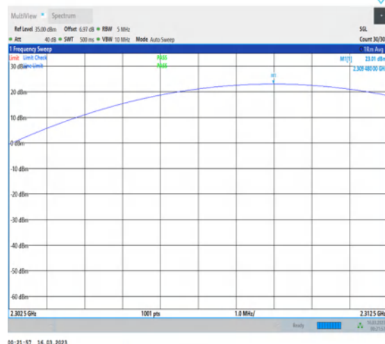
1-N30-PC3-15-5-L-2-DFT-PI2BPSK- Inner_1RB_Right-1@23-2302.5-2312.5-Ant1-2309.48-23.01-99-PASS
