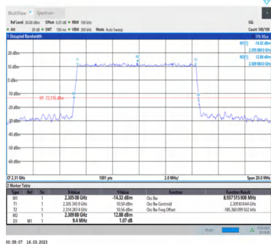
1-N30-PC3-15-10-L-1-DFT-QPSK-Outer_Full-50@0-Ant1-8.938-9.400-≤10-PASS
