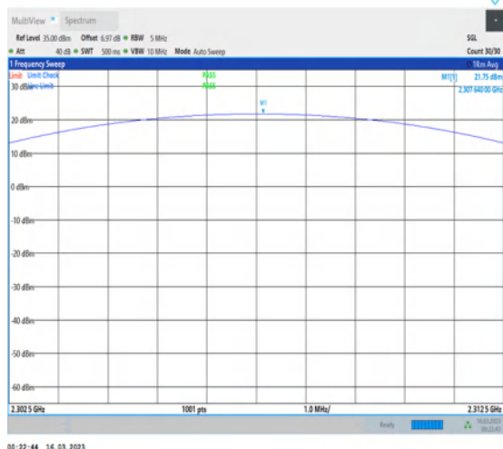
1-N30-PC3-15-5-L-3-DFT-PI2BPSK-Outer_Full- 25@0-2302.5-2312.5-Ant1-2307.64-21.75-99-PASS
