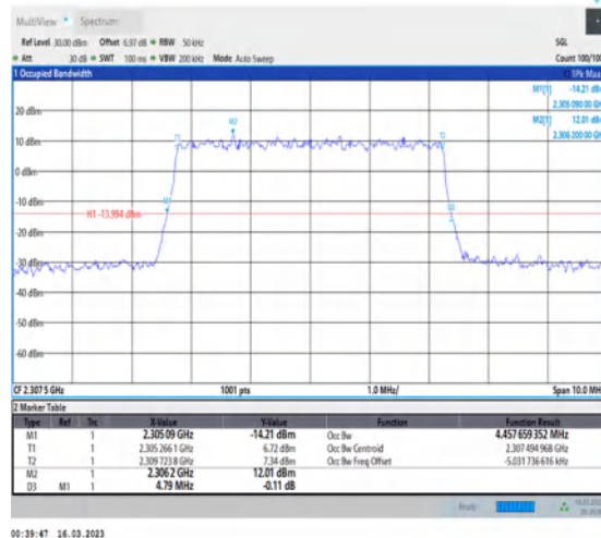
1-N30-PC3-15-5-L-4-DFT-64QAM-Outer_Full-25@0- Ant1-4.458-4.790-≤5-PASS
