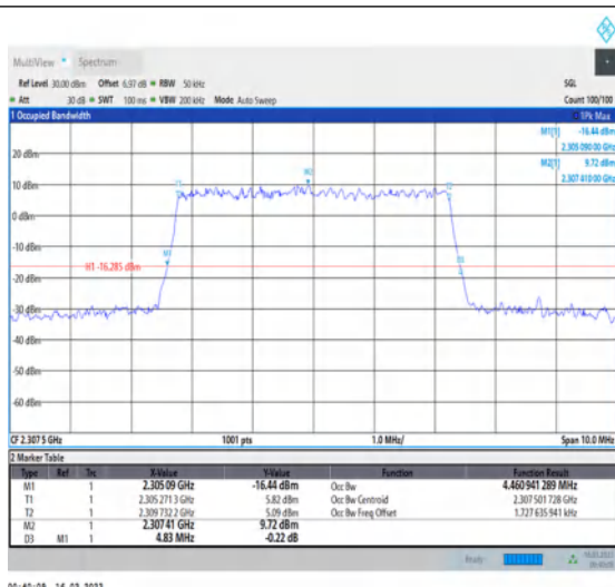
1-N30-PC3-15-5-L-5-DFT-256QAM-Outer_Full-25@0-Ant1-4.461-4.830-≤5-PASS
