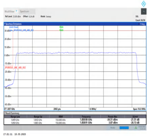
1-N25-PC3-15-15-L-3-DFT-PI2BPSK-Outer_Full-75@0-Ant1-1-seegraph-PASS-see graph
