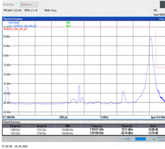
1-N25-PC3-15-15-H-2-DFT-PI2BPSK-Edge_1RB_Right-1@78-Ant1-1-seegraph-PASS-see graph
