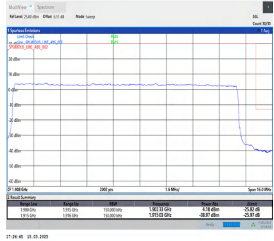
1-N25-PC3-15-15-H-3-DFT-PI2BPSK-Outer_Full-75@0-Ant1-1-seegraph-PASS-see graph
