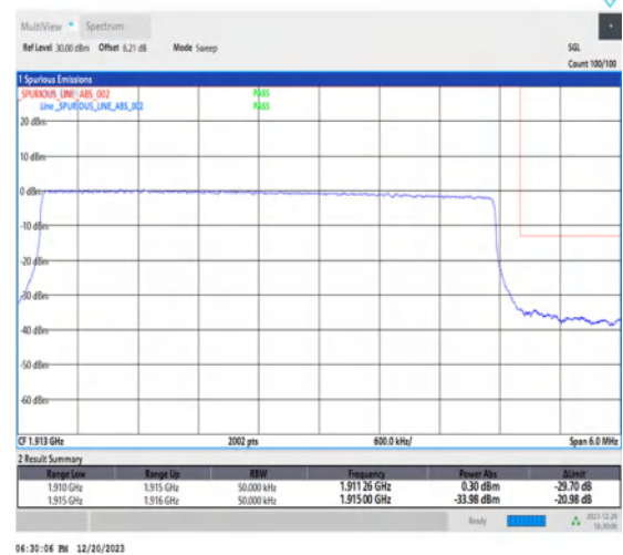
1-N25-15-5-H-6-CP-QPSK-Outer_Full-25@0-Ant1-1-seegraph-PASS-see graph
