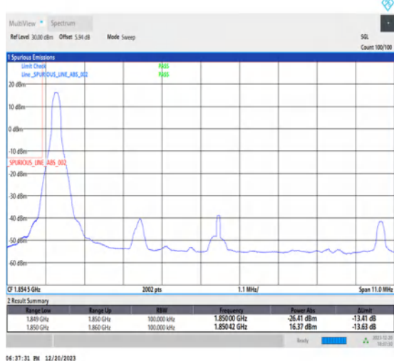
1-N25-15-10-L-4-CP-QPSK-Edge_1RB_Left-1@0-Ant1-1-seegraph-PASS-see graph
