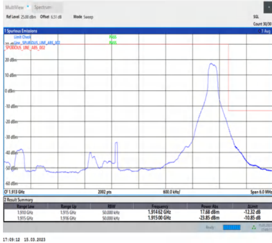
1-N25-PC3-15-5-H-2-DFT-PI2BPSK-Edge_1RB_Right-1@24-Ant1-1-seegraph-PASS-see graph
