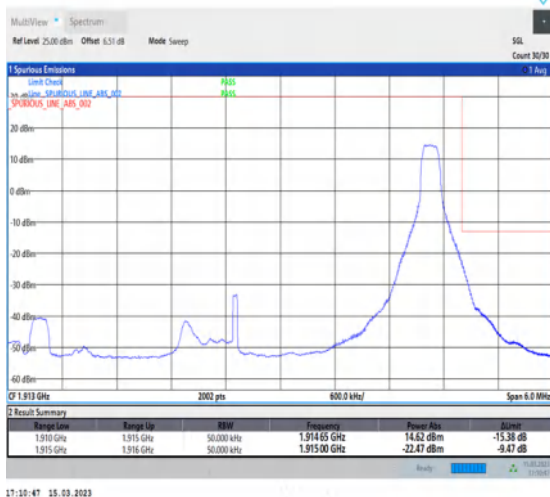
1-N25-PC3-15-5-H-5-CP-QPSK-Edge_1RB_Right-1@24-Ant1-1-seegraph-PASS-see graph
