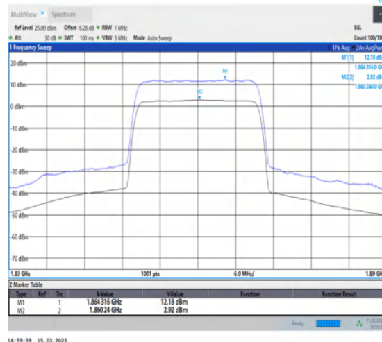
1-N25-PC3-15-20-L-2-CP-256QAM-Outer_Full-106@0-Ant1-9.26-100%-0.00-9.26-PASS-≤13
