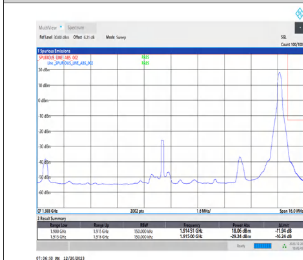
1-N25-15-15-H-5-CP-QPSK-Edge_1RB_Right-1@78-Ant1-1-seegraph-PASS-see graph
