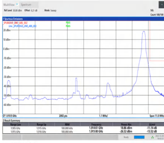
1-N25-15-10-H-2-DFT-PI2BPSK-Edge_1RB_Right-1@51-Ant1-1-seegraph-PASS-see graph
