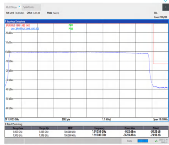
1-N25-15-10-H-6-CP-QPSK-Outer_Full-52@0-Ant1-1-seegraph-PASS-see graph
