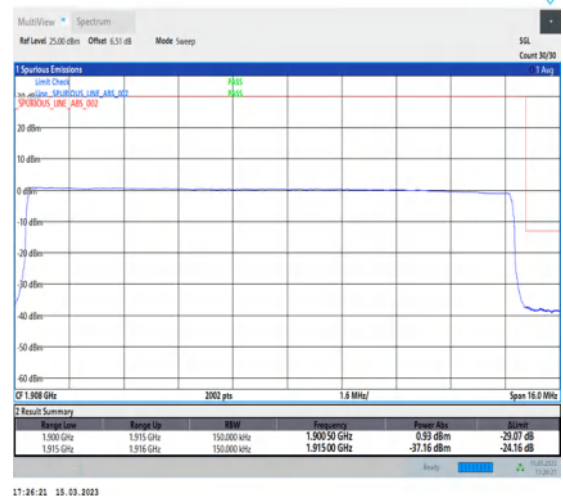
1-N25-PC3-15-15-H-6-CP-QPSK-Outer_Full-79@0-Ant1-1-seegraph-PASS-see graph
