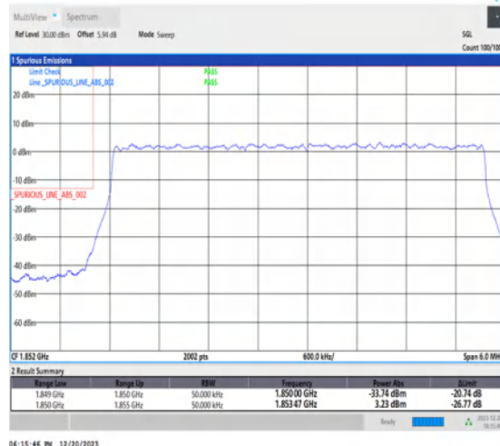
1-N25-15-5-L-3-DFT-PI2BPSK-Outer_Full-25@0-Ant1-1-seegraph-PASS-see graph
