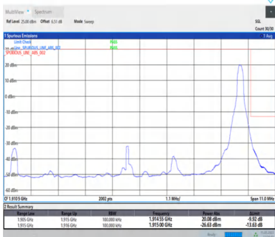
1-N25-PC3-15-10-H-2-DFT-PI2BPSK-Edge_1RB_Right-1@51-Ant1-1-seegraph-PASS-see graph
