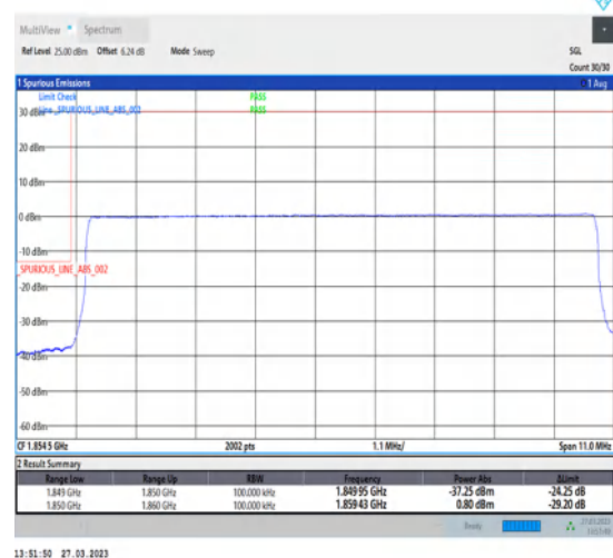
1-N25-PC3-15-10-L-6-CP-QPSK-Outer_Full-52@0-Ant1-1-seegraph-PASS-see graph
