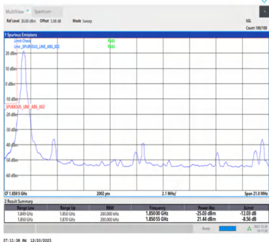
1-N25-15-20-L-1-DFT-PI2BPSK-Edge_1RB_Left-1@0-Ant1-1-seegraph-PASS-see graph
