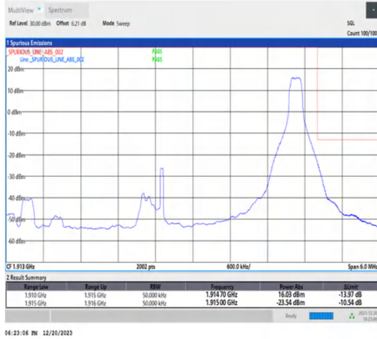
1-N25-15-5-H-2-DFT-PI2BPSK-Edge_1RB_Right-1@24-Ant1-1-seegraph-PASS-see graph
