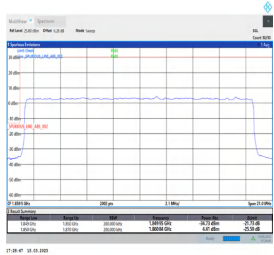
1-N25-PC3-15-20-L-3-DFT-PI2BPSK-Outer_Full-100@0-Ant1-1-seegraph-PASS-see graph
