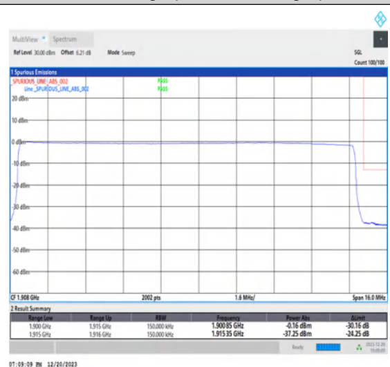
1-N25-15-15-H-6-CP-QPSK-Outer_Full-79@0-Ant1-1-seegraph-PASS-see graph
