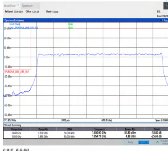
1-N25-PC3-15-5-L-3-DFT-PI2BPSK-Outer_Full-25@0-Ant1-1-seegraph-PASS-see graph
