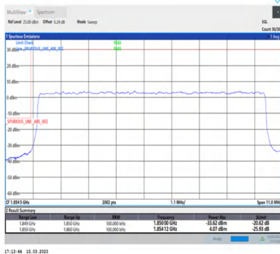
1-N25-PC3-15-10-L-3-DFT-PI2BPSK-Outer_Full-50@0-Ant1-1-seegraph-PASS-see graph
