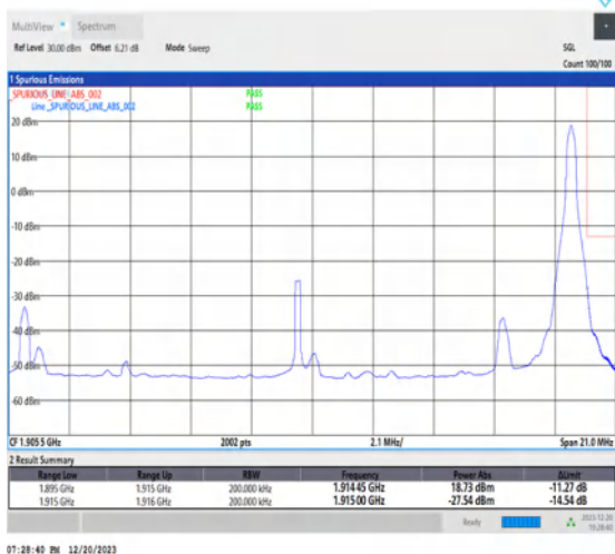
1-N25-15-20-H-5-CP-QPSK-Edge_1RB_Right-1@105-Ant1-1-seegraph-PASS-see graph
