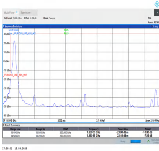
1-N25-PC3-15-20-L-1-DFT-PI2BPSK-Edge_1RB_Left-1@0-Ant1-1-seegraph-PASS-see graph
