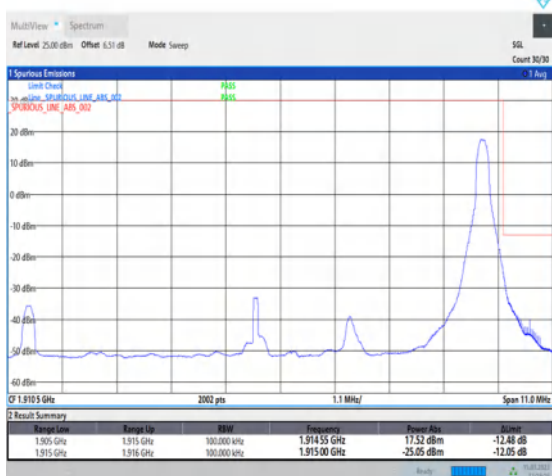
1-N25-PC3-15-10-H-5-CP-QPSK-Edge_1RB_Right-1@51-Ant1-1-seegraph-PASS-see graph
