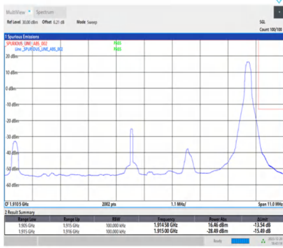
1-N25-15-10-H-5-CP-QPSK-Edge_1RB_Right-1@51-Ant1-1-seegraph-PASS-see graph
