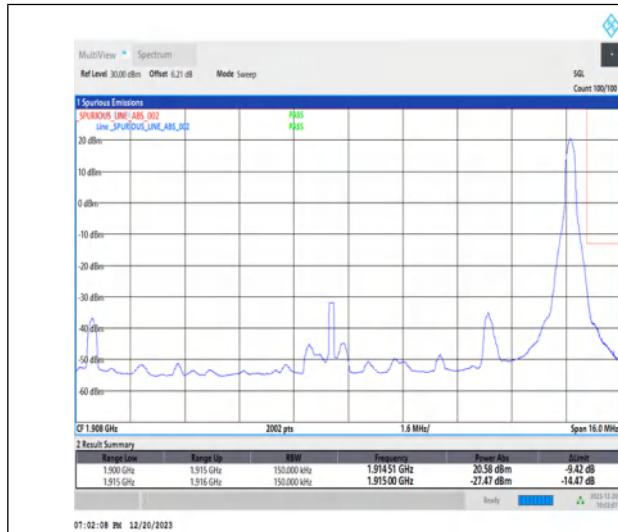
1-N25-15-15-H-2-DFT-PI2BPSK-Edge_1RB_Right-1@78-Ant1-1-seegraph-PASS-see graph
