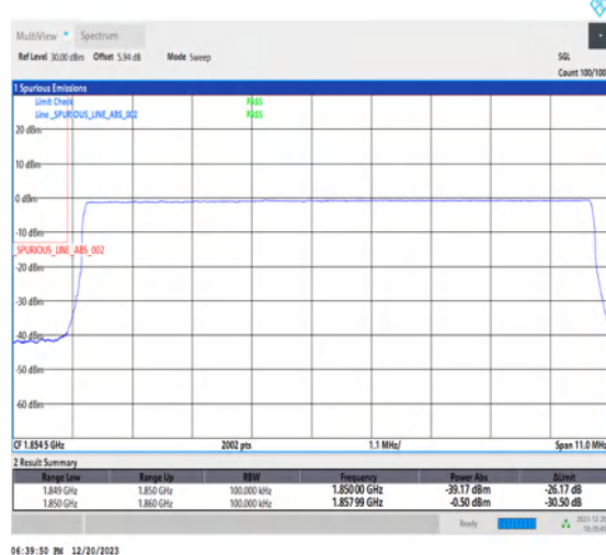
1-N25-15-10-L-6-CP-QPSK-Outer_Full-52@0-Ant1-1-seegraph-PASS-see graph
