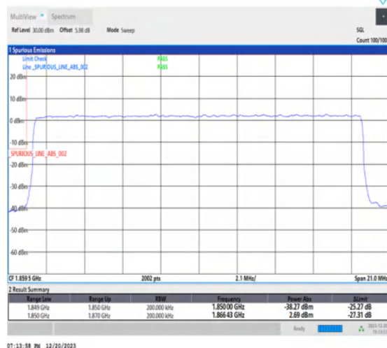
1-N25-15-20-L-3-DFT-PI2BPSK-Outer_Full-100@0-Ant1-1-seegraph-PASS-see graph
