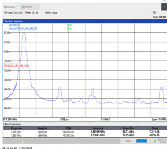
1-N25-15-10-L-1-DFT-PI2BPSK-Edge_1RB_Left-1@0-Ant1-1-seegraph-PASS-see graph
