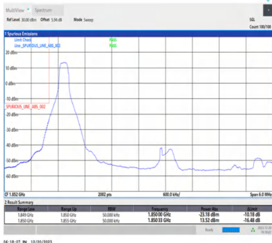
1-N25-15-5-L-4-CP-QPSK-Edge_1RB_Left-1@0-Ant1-1-seegraph-PASS-see graph
