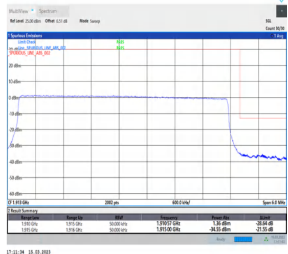
1-N25-PC3-15-5-H-6-CP-QPSK-Outer_Full-25@0-Ant1-1-seegraph-PASS-see graph
