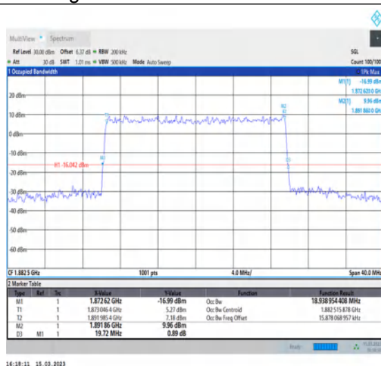
1-N25-PC3-15-20-M-8-CP-64QAM-Outer_Full-106@0-Ant1-18.939-19.720-≤20-PASS
