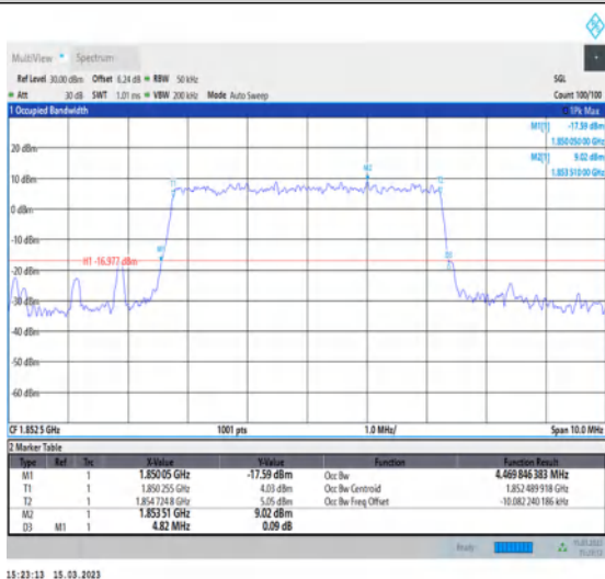
1-N25-PC3-15-5-L-7-CP-16QAM-Outer_Full-25@0-Ant1-4.474-4.820-≤5-PASS
