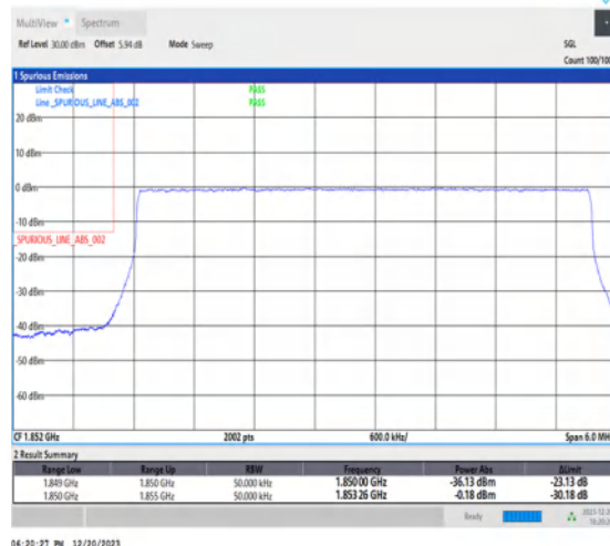
1-N25-15-5-L-6-CP-QPSK-Outer_Full-25@0-Ant1-1-seegraph-PASS-see graph
