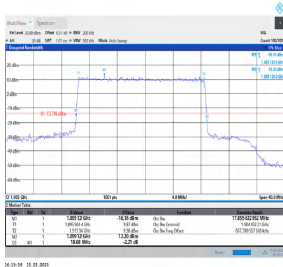
1-N25-PC3-15-20-H-1-DFT-QPSK-Outer_Full-100@0-Ant1-17.856-18.680-≤20-PASS
