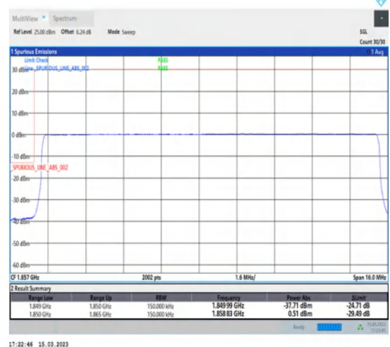
1-N25-PC3-15-15-L-6-CP-QPSK-Outer_Full-79@0-Ant1-1-seegraph-PASS-see graph
