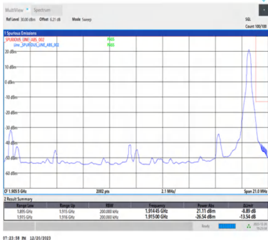
1-N25-15-20-H-2-DFT-PI2BPSK-Edge_1RB_Right-1@105-Ant1-1-seegraph-PASS-see graph
