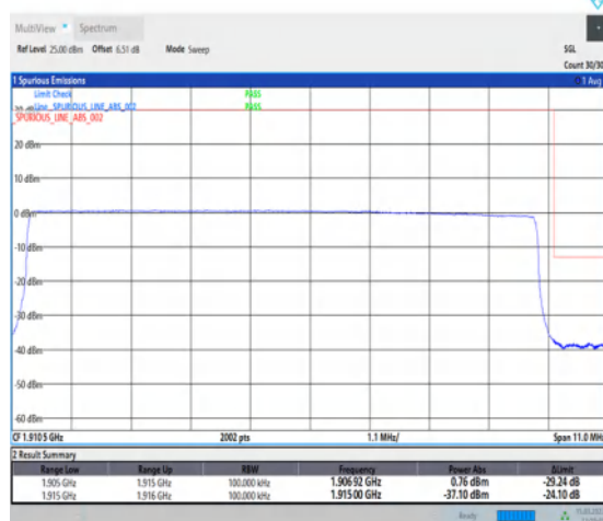
1-N25-PC3-15-10-H-6-CP-QPSK-Outer_Full-52@0-Ant1-1-seegraph-PASS-see graph
