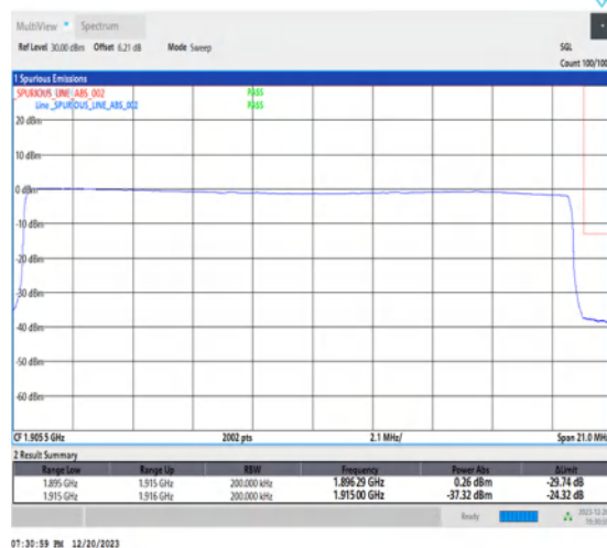
1-N25-15-20-H-6-CP-QPSK-Outer_Full-106@0-Ant1-1-seegraph-PASS-see graph
