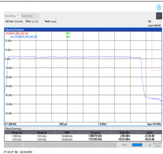
1-N25-15-15-H-3-DFT-PI2BPSK-Outer_Full-75@0-Ant1-1-seegraph-PASS-see graph
