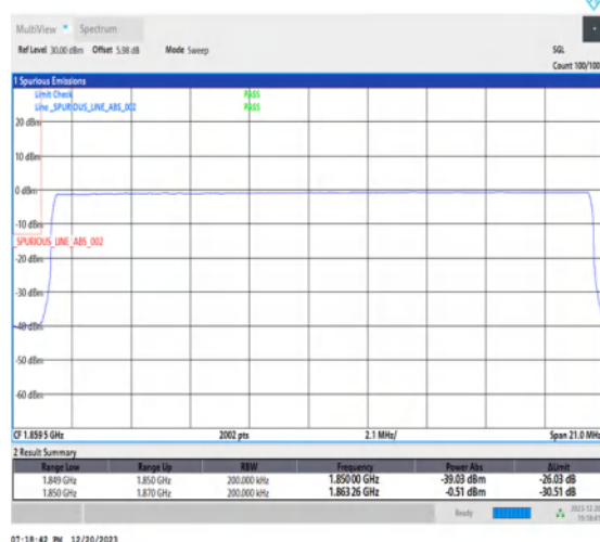
1-N25-15-20-L-6-CP-QPSK-Outer_Full-106@0-Ant1-1-seegraph-PASS-see graph
