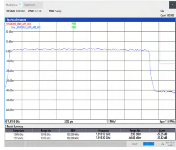
1-N25-15-10-H-3-DFT-PI2BPSK-Outer_Full-50@0-Ant1-1-seegraph-PASS-see graph
