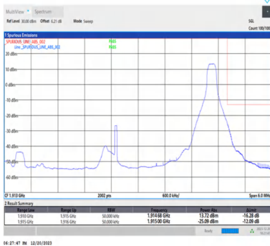
1-N25-15-5-H-5-CP-QPSK-Edge_1RB_Right-1@24-Ant1-1-seegraph-PASS-see graph
