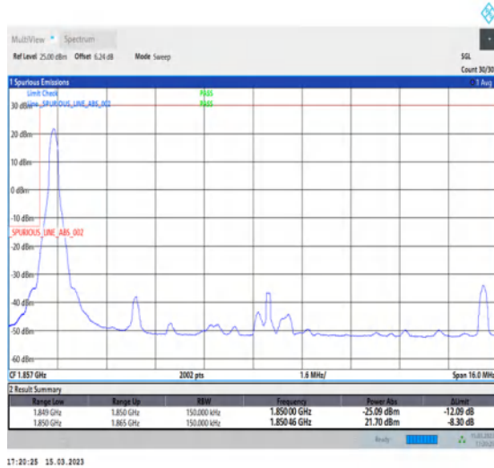
1-N25-PC3-15-15-L-1-DFT-PI2BPSK-Edge_1RB_Left-1@0-Ant1-1-seegraph-PASS-see graph
