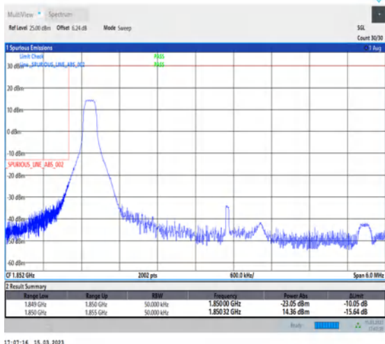
1-N25-PC3-15-5-L-4-CP-QPSK-Edge_1RB_Left-1@0-Ant1-1-seegraph-PASS-see graph
