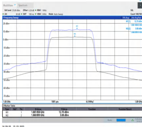
1-N25-PC3-15-20-L-1-DFT-256QAM-Outer_Full-100@0-Ant1-9.62-100%-0.00-9.62-PASS-≤13
