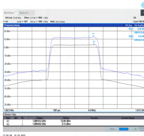
1-N25-PC3-15-20-M-2-CP-256QAM-Outer_Full-106@0-Ant1-9.71-100%-0.00-9.71-PASS-≤13
