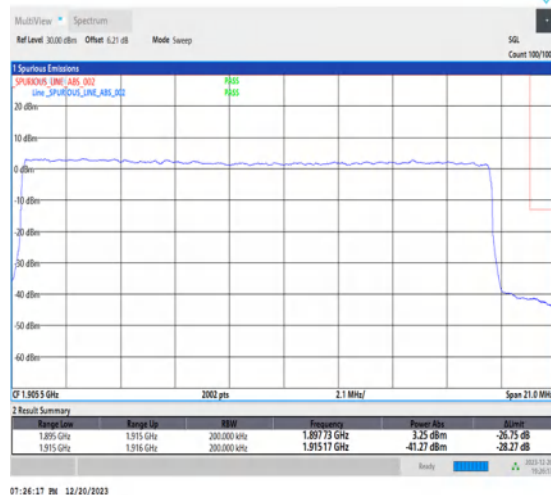
1-N25-15-20-H-3-DFT-PI2BPSK-Outer_Full-100@0-Ant1-1-seegraph-PASS-see graph
