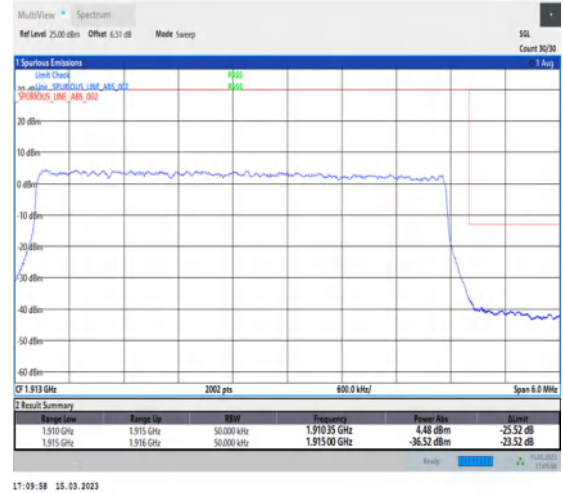
1-N25-PC3-15-5-H-3-DFT-PI2BPSK-Outer_Full-25@0-Ant1-1-seegraph-PASS-see graph
