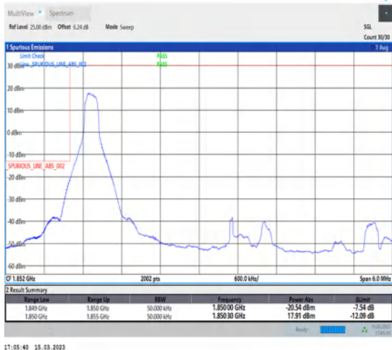
1-N25-PC3-15-5-L-1-DFT-PI2BPSK-Edge_1RB_Left-1@0-Ant1-1-seegraph-PASS-see graph
