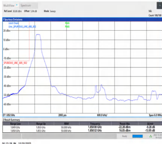
1-N25-15-5-L-1-DFT-PI2BPSK-Edge_1RB_Left-1@0-Ant1-1-seegraph-PASS-see graph
