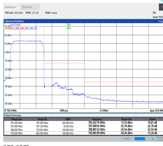
1-N13-PC3-15-5-H-3-DFT-PI2BPSK-Outer_Full-25@0-Ant7-1--PASS-see graph
