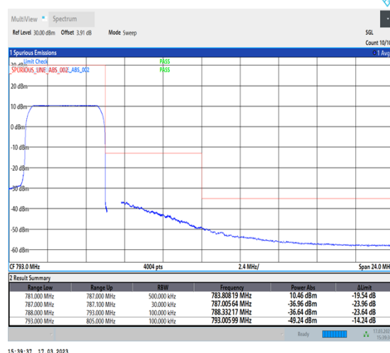
1-N13-PC3-15-5-H-6-CP-QPSK-Outer_Full-25@0-Ant7-1--PASS-see graph
