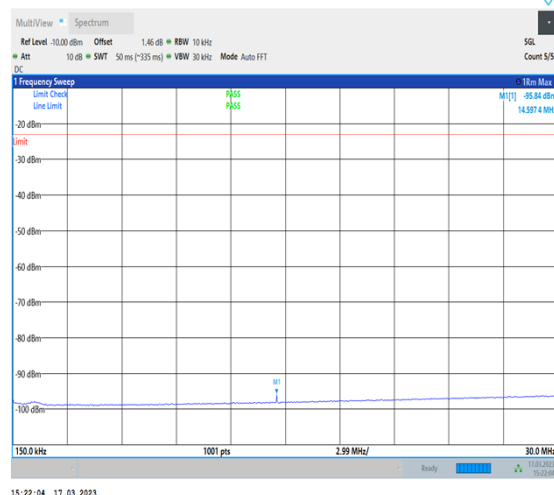
1-N13-PC3-15-10-M-1-DFT-PI2BPSK- Inner_1RB_Left-1@1-0.15-30-Ant7-14.60--95.84--23- PASS
