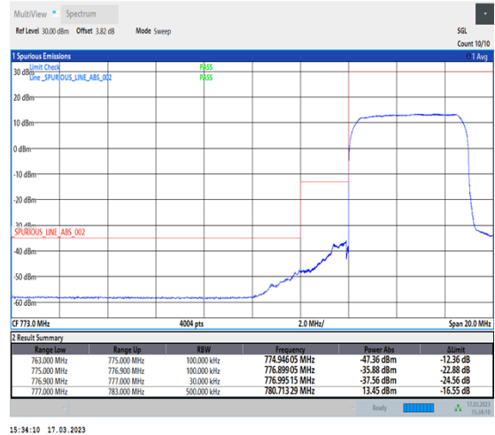
1-N13-PC3-15-5-L-3-DFT-PI2BPSK-Outer_Full-25@0-Ant7-1--PASS-see graph
