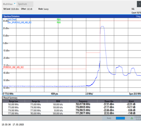
1-N13-PC3-15-5-L-1-DFT-PI2BPSK-Edge_1RB_Left-1@0-Ant7-1--PASS-see graph
