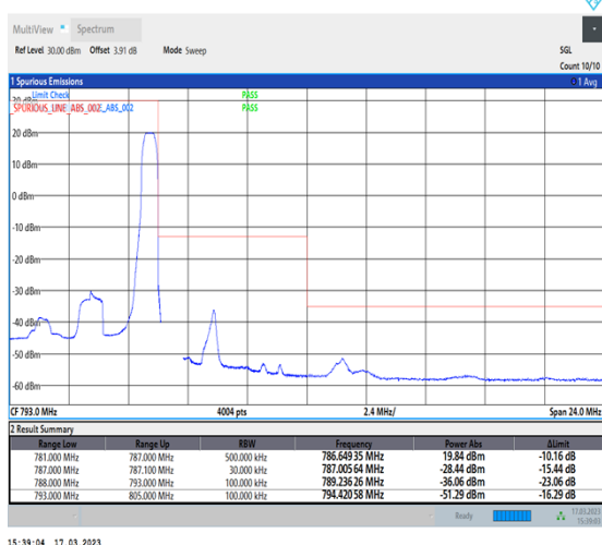
1-N13-PC3-15-5-H-5-CP-QPSK-Edge_1RB_Right-1@24-Ant7-1--PASS-see graph
