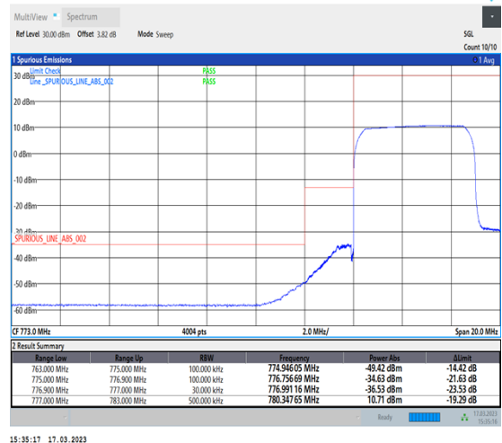
1-N13-PC3-15-5-L-6-CP-QPSK-Outer_Full-25@0-Ant7-1--PASS-see graph
