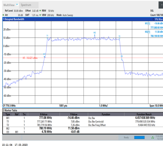
1-N13-PC3-15-5-L-3-DFT-16QAM-Outer_Full-25@0- Ant7-4.458-4.780-≤5-PASS
