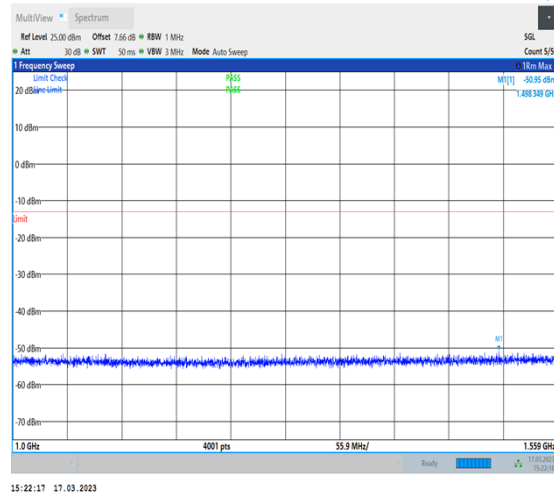
1-N13-PC3-15-10-M-1-DFT-PI2BPSK- Inner_1RB_Left-1@1-1000-1559-Ant7-1498.35-- 50.95--13-PASS
