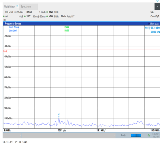
1-N13-PC3-15-10-M-1-DFT-PI2BPSK- Inner_1RB_Left-1@1-0.009-0.15-Ant7-0.06--99.78-- 33-PASS
