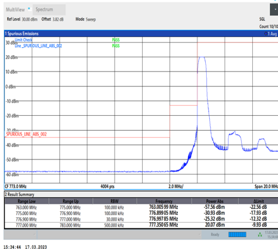
1-N13-PC3-15-5-L-4-CP-QPSK-Edge_1RB_Left-1@0-Ant7-1--PASS-see graph
