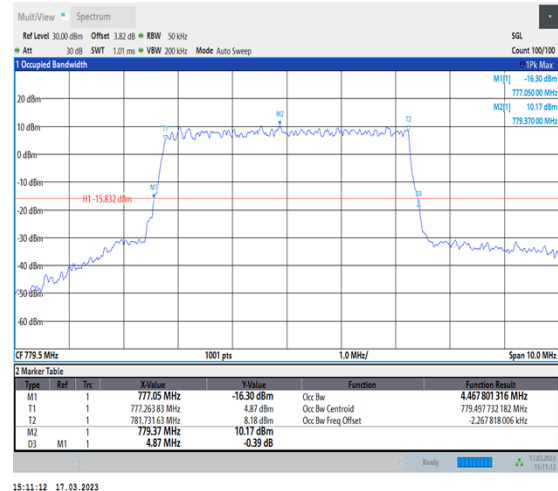
1-N13-PC3-15-5-L-4-DFT-64QAM-Outer_Full-25@0- Ant7-4.468-4.870-≤5-PASS
