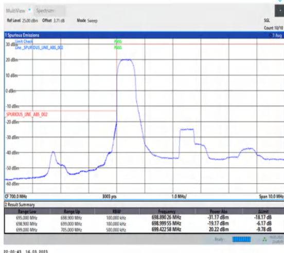
1-N12-PC3-15-5-L-4-CP-QPSK-Edge_1RB_Left-1@0-Ant7-1--PASS-see graph
