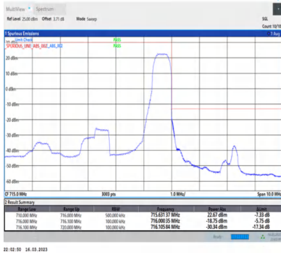
1-N12-PC3-15-5-H-2-DFT-PI2BPSK-Edge_1RB_Right-1@24-Ant7-1--PASS-see graph
