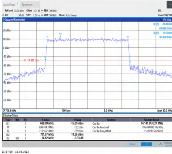
1-N12-PC3-15-15-L-7-CP-16QAM-Outer_Full-79@0-Ant7-14.141-14.820-≤15-PASS
