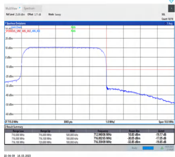
1-N12-PC3-15-5-H-6-CP-QPSK-Outer_Full-25@0-Ant7-1--PASS-see graph
