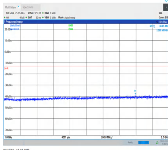
1-N12-PC3-15-15-M-1-DFT-PI2BPSK- Inner_1RB_Left-1@1-1000-3000-Ant7-2590.50-- 38.61--13-PASS
