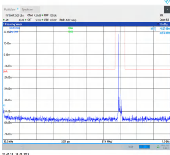
1-N12-PC3-15-15-H-1-DFT-PI2BPSK- Inner_1RB_Left-1@1-30-1000-Ant7-30.97--48.37-- 13-PASS
