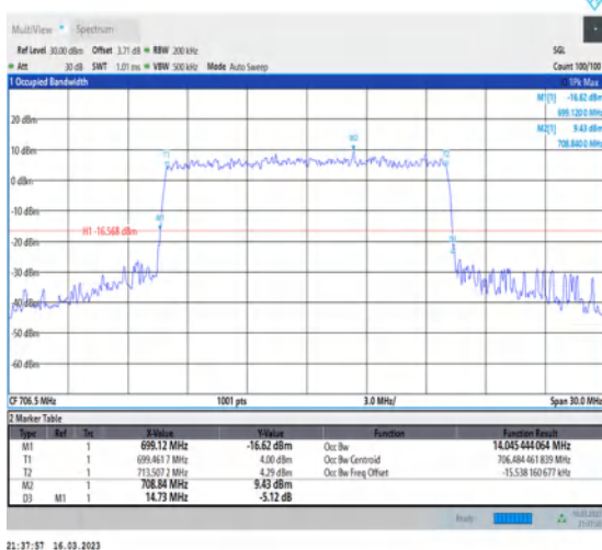
1-N12-PC3-15-15-L-9-CP-256QAM-Outer_Full-79@0-Ant7-14.045-14.730-≤15-PASS
