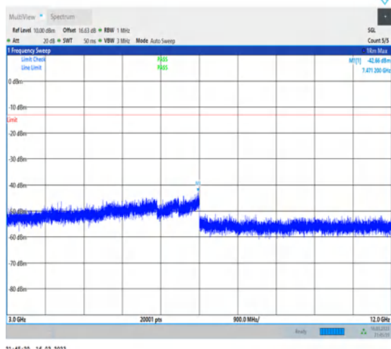
1-N12-PC3-15-15-L-1-DFT-PI2BPSK- Inner_1RB_Left-1@1-3000-12000-Ant7-7471.20-- 42.66--13-PASS
