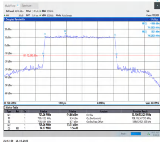
1-N12-PC3-15-15-H-4-DFT-64QAM-Outer_Full-75@0-Ant7-13.406-14.070-≤15-PASS
