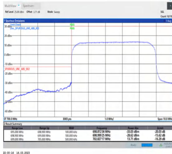
1-N12-PC3-15-5-L-3-DFT-PI2BPSK-Outer_Full-25@0-Ant7-1--PASS-see graph
