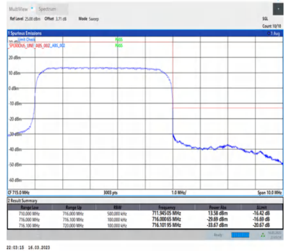
1-N12-PC3-15-5-H-3-DFT-PI2BPSK-Outer_Full-25@0-Ant7-1--PASS-see graph
