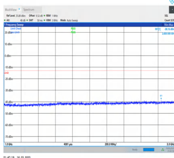
1-N12-PC3-15-15-H-1-DFT-PI2BPSK- Inner_1RB_Left-1@1-1000-3000-Ant7-2835.50-- 38.16--13-PASS
