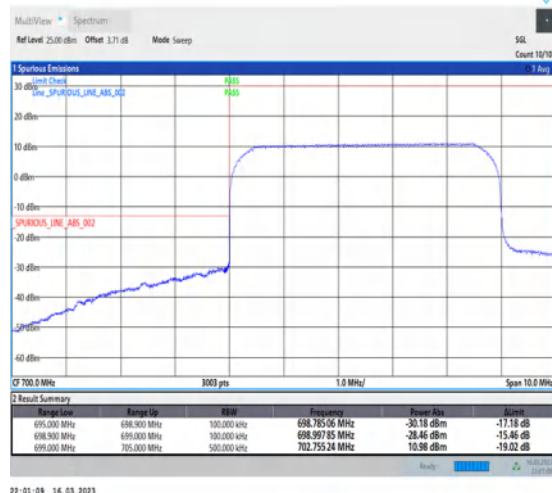
1-N12-PC3-15-5-L-6-CP-QPSK-Outer_Full-25@0-Ant7-1--PASS-see graph
