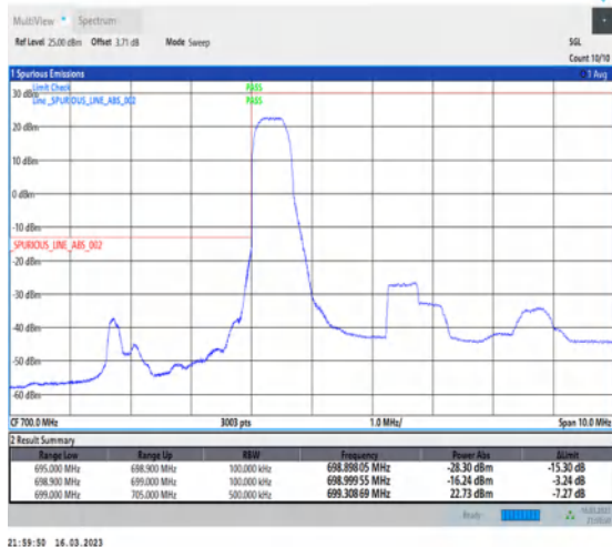
1-N12-PC3-15-5-L-1-DFT-PI2BPSK-Edge_1RB_Left-1@0-Ant7-1--PASS-see graph
