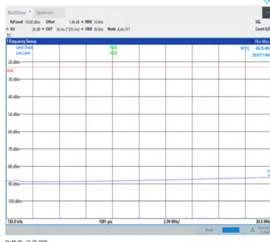
1-N12-PC3-15-15-M-1-DFT-PI2BPSK- Inner_1RB_Left-1@1-0.15-30-Ant7-29.67--86.25--23- PASS
