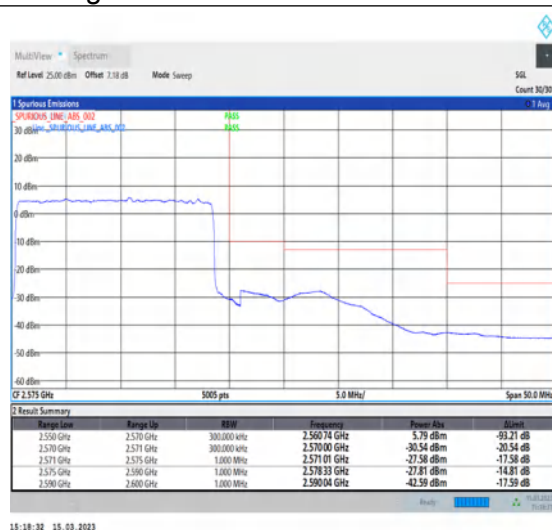
1-N7-PC3-15-20-H-3-DFT-PI2BPSK-Outer_Full-100@0-Ant1-1--PASS-see graph
