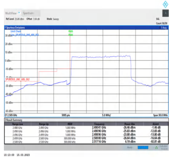
1-N7-PC3-15-20-L-3-DFT-PI2BPSK-Outer_Full-100@0-Ant1-1--PASS-see graph
