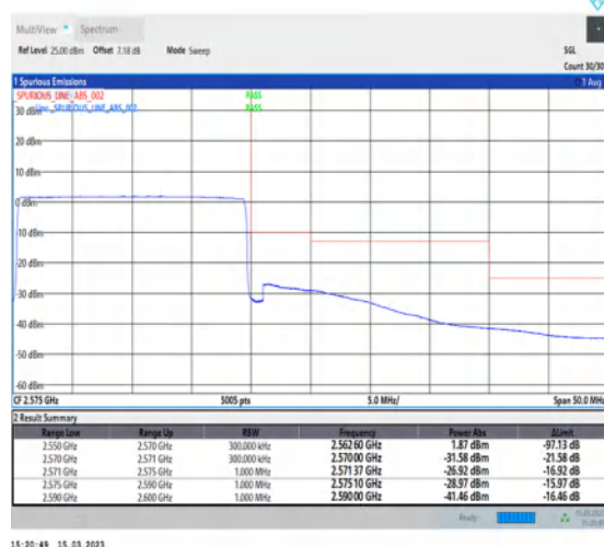
1-N7-PC3-15-20-H-6-CP-QPSK-Outer_Full-106@0-Ant1-1--PASS-see graph
