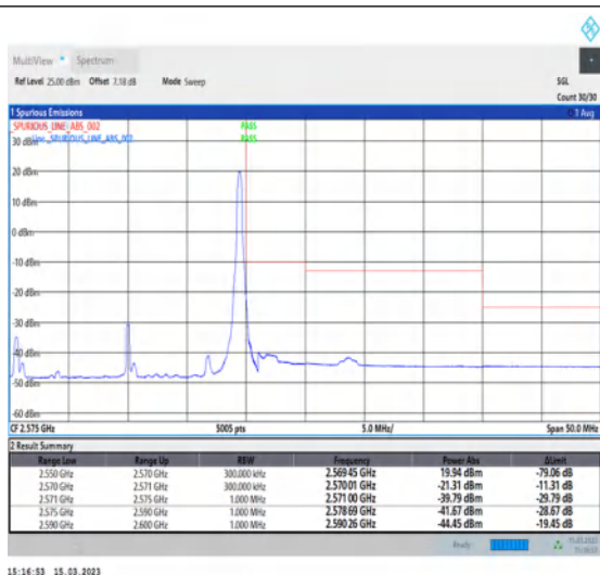
1-N7-PC3-15-20-H-2-DFT-PI2BPSK-Edge_1RB_Right-1@105-Ant1-1--PASS-see graph
