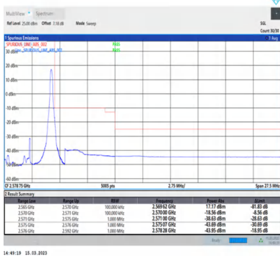
1-N7-PC3-15-5-H-5-CP-QPSK-Edge_1RB_Right-1@24-Ant1-1--PASS-see graph
