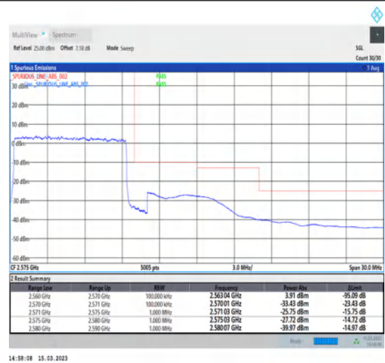
1-N7-PC3-15-10-H-3-DFT-PI2BPSK-Outer_Full-50@0-Ant1-1--PASS-see graph
