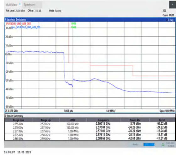
1-N7-PC3-15-15-H-3-DFT-PI2BPSK-Outer_Full-75@0-Ant1-1--PASS-see graph
