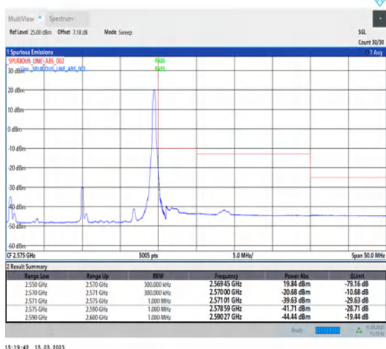
1-N7-PC3-15-20-H-5-CP-QPSK-Edge_1RB_Right-1@105-Ant1-1--PASS-see graph
