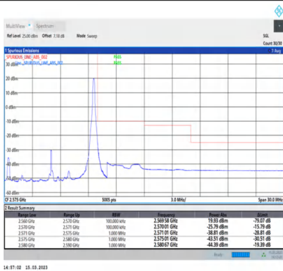
1-N7-PC3-15-10-H-2-DFT-PI2BPSK-Edge_1RB_Right-1@51-Ant1-1--PASS-see graph
