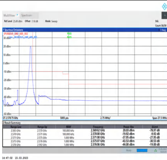
1-N7-PC3-15-5-H-2-DFT-PI2BPSK-Edge_1RB_Right-1@24-Ant1-1--PASS-see graph
