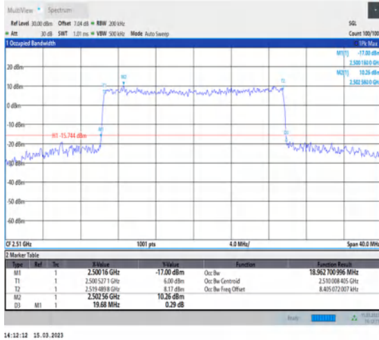
1-N7-PC3-15-20-L-8-CP-64QAM-Outer_Full-106@0-Ant1-18.963-19.680-≤20-PASS
