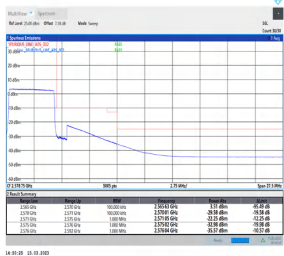
1-N7-PC3-15-5-H-6-CP-QPSK-Outer_Full-25@0-Ant1-1--PASS-see graph
