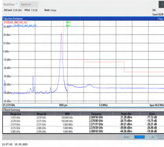
1-N7-PC3-15-15-H-2-DFT-PI2BPSK-Edge_1RB_Right-1@78-Ant1-1--PASS-see graph
