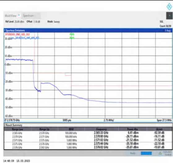
1-N7-PC3-15-5-H-3-DFT-PI2BPSK-Outer_Full-25@0-Ant1-1--PASS-see graph
