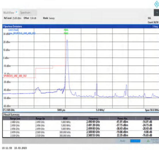
1-N7-PC3-15-20-L-1-DFT-PI2BPSK-Edge_1RB_Left-1@0-Ant1-1--PASS-see graph
