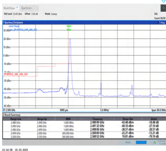
1-N7-PC3-15-20-L-4-CP-QPSK-Edge_1RB_Left-1@0-Ant1-1--PASS-see graph
