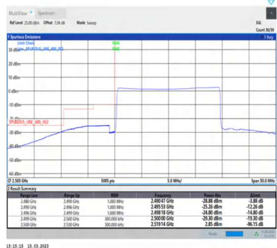
1-N7-PC3-15-20-L-6-CP-QPSK-Outer_Full-106@0-Ant1-1--PASS-see graph
