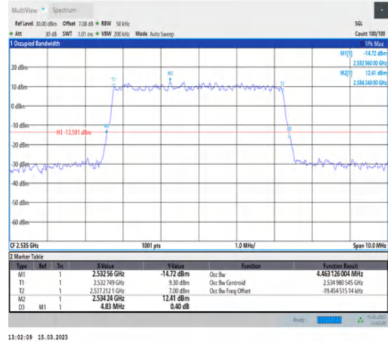
1-N7-PC3-15-5-M-1-DFT-QPSK-Outer_Full-25@0-Ant1-4.463-4.830-≤5-PASS
