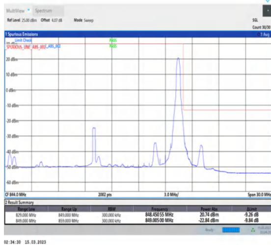
1-N5-PC3-15-20-H-5-CP-QPSK-Edge_1RB_Right-1@105-Ant1-1-seegraph-PASS-see graph
