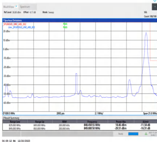
1-N515-20-H-5-CP-QPSK-Edge_1RB_Right-1@105-Ant1-1-seegraph-PASS-see graph
