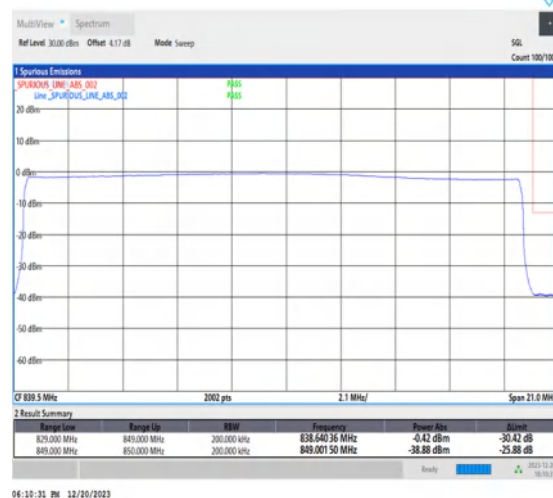
1-N515-20-H-6-CP-QPSK-Outer_Full-106@0-Ant1-1-seegraph-PASS-see graph
