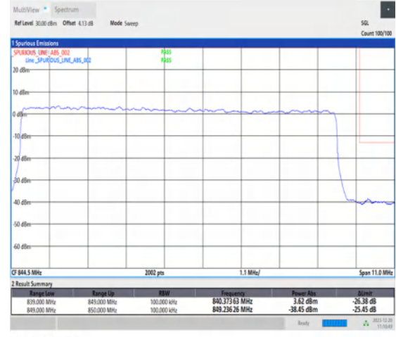
1-N515-10-H-3-DFT-PI2BPSK-Outer_Full-50@0-Ant1-1-seegraph-PASS-see graph
