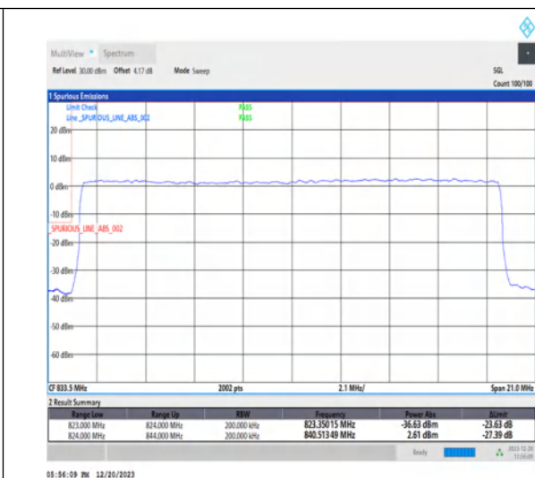
1-N515-20-L-3-DFT-PI2BPSK-Outer_Full-100@0-Ant1-1-seegraph-PASS-see graph
