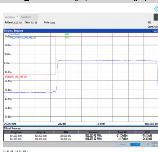
1-N5-PC3-15-20-L-6-CP-QPSK-Outer_Full-106@0-Ant1-1-seegraph-PASS-see graph
