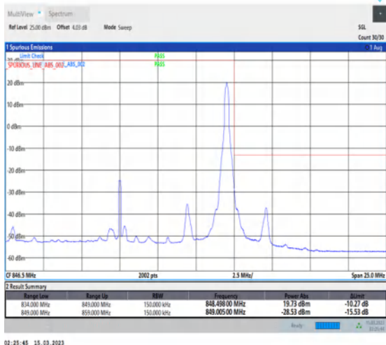
1-N5-PC3-15-15-H-2-DFT-PI2BPSK-Edge_1RB_Right-1@78-Ant1-1-seegraph-PASS-see graph
