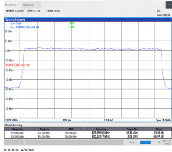
1-N515-10-L-3-DFT-PI2BPSK-Outer_Full-50@0-Ant1-1-seegraph-PASS-see graph
