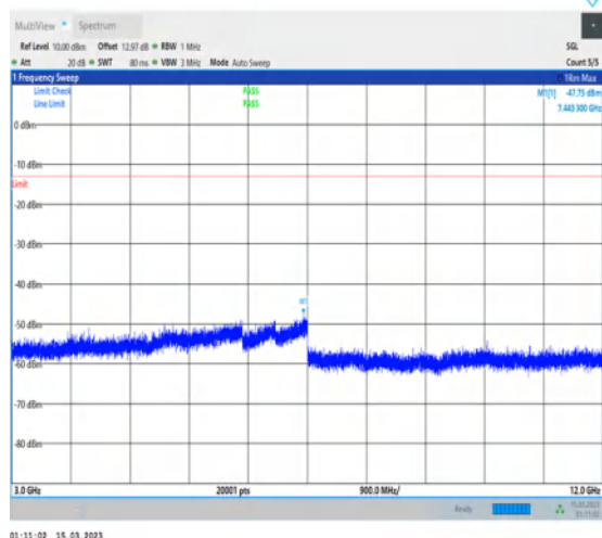
1-N5-PC3-15-20-H-1-DFT-PI2BPSK- Inner_1RB_Left-1@1-3000-12000-Ant1-7443.30-- 47.75--13-PASS
