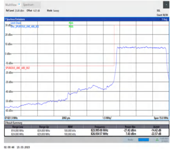
1-N5-PC3-15-5-L-3-DFT-PI2BPSK-Outer_Full-25@0-Ant1-1-seegraph-PASS-see graph
