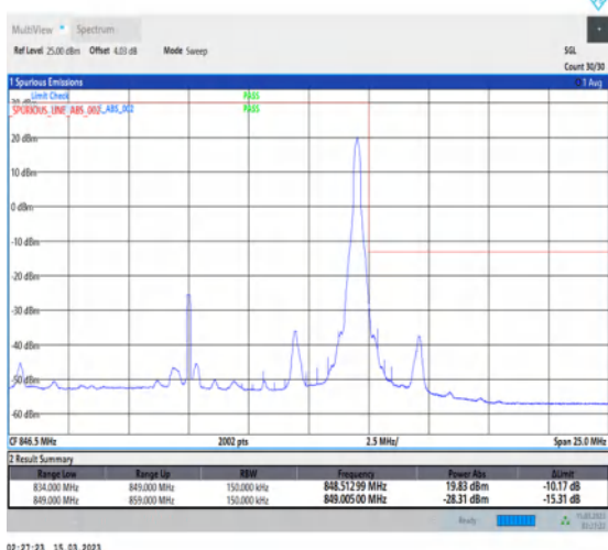
1-N5-PC3-15-15-H-5-CP-QPSK-Edge_1RB_Right-1@78-Ant1-1-seegraph-PASS-see graph
