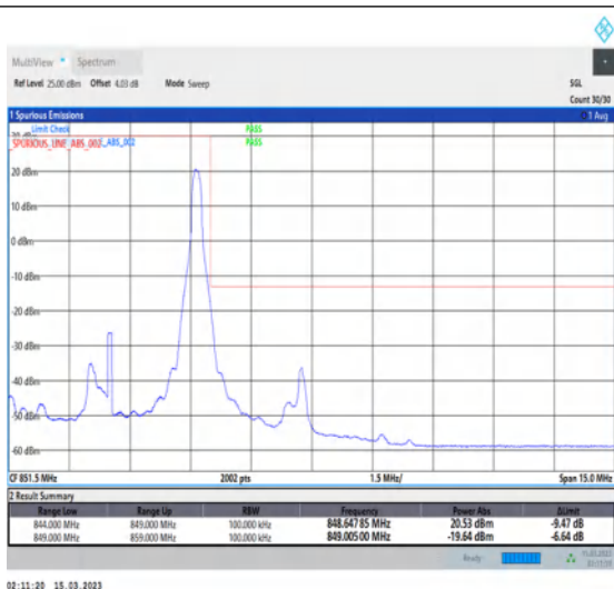
1-N5-PC3-15-5-H-2-DFT-PI2BPSK-Edge_1RB_Right-1@24-Ant1-1-seegraph-PASS-see graph
