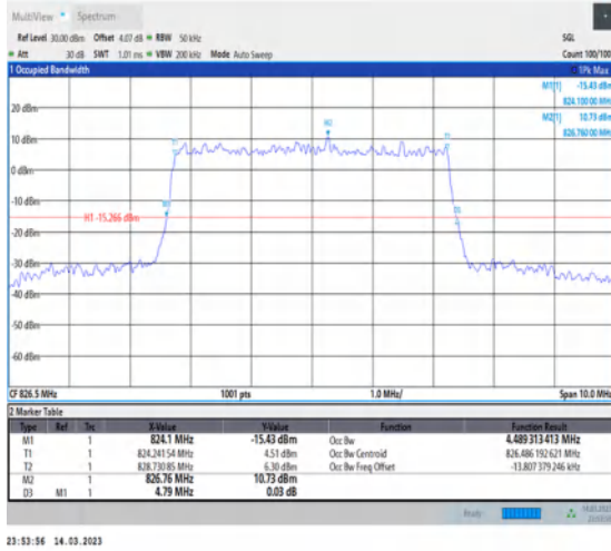
1-N5-PC3-15-5-L-5-DFT-256QAM-Outer_Full-25@0-Ant1-4.489-4.790-≤5-PASS
