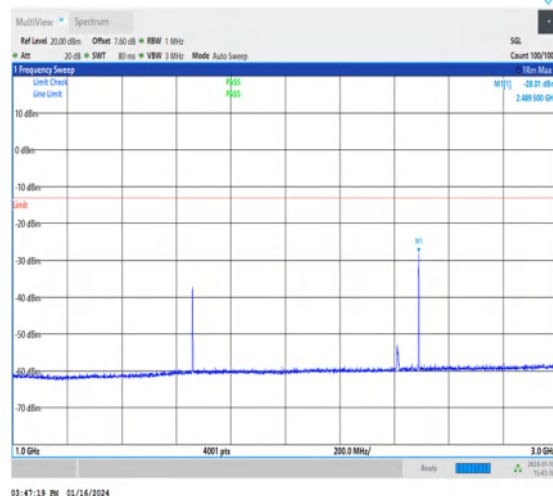
1-N5-15-20-H-1-DFT-PI2BPSK-Inner_1RB_Left- 1@1-1000-3000-Ant1-2886.00--28.01--13-PASS
