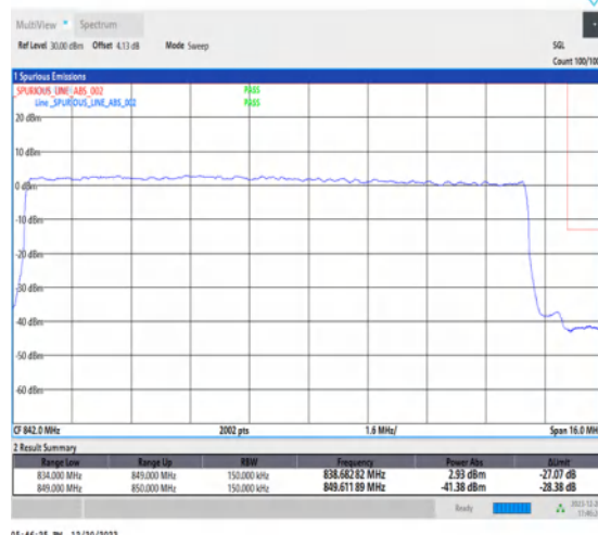
1-N515-15-H-3-DFT-PI2BPSK-Outer_Full-75@0-Ant1-1-seegraph-PASS-see graph
