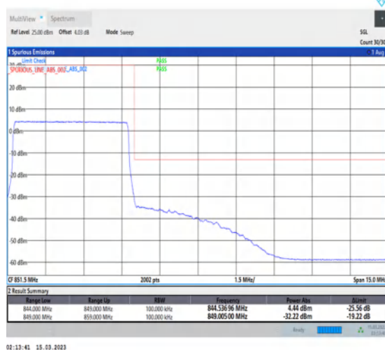
1-N5-PC3-15-5-H-6-CP-QPSK-Outer_Full-25@0-Ant1-1-seegraph-PASS-see graph
