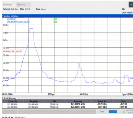
1-N515-5-L-1-DFT-PI2BPSK-Edge_1RB_Left-1@0-Ant1-1-seegraph-PASS-see graph
