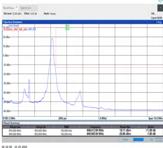
1-N5-PC3-15-5-H-5-CP-QPSK-Edge_1RB_Right-1@24-Ant1-1-seegraph-PASS-see graph
