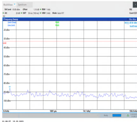
1-N5-PC3-15-20-L-1-DFT-PI2BPSK- Inner_1RB_Left-1@1-0.009-0.15-Ant1-0.02--87.81-- 33-PASS
