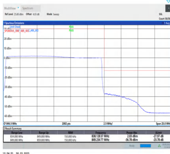
1-N5-PC3-15-15-H-6-CP-QPSK-Outer_Full-79@0-Ant1-1-seegraph-PASS-see graph
