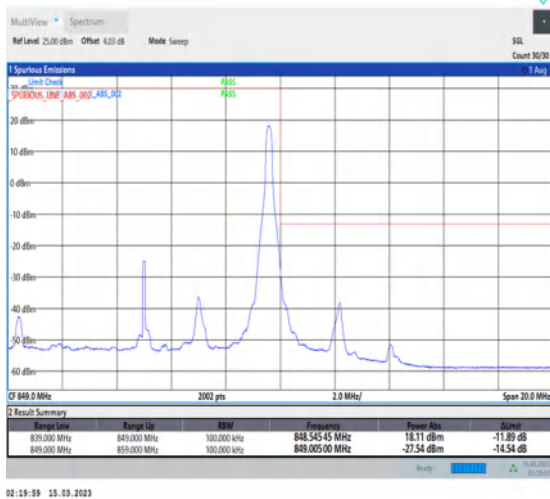
1-N5-PC3-15-10-H-5-CP-QPSK-Edge_1RB_Right-1@51-Ant1-1-seegraph-PASS-see graph
