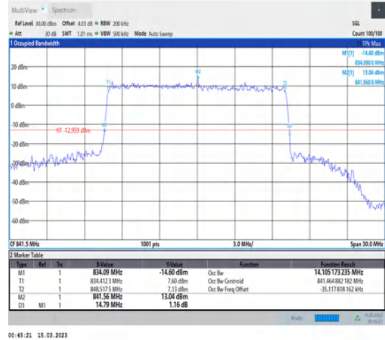
1-N5-PC3-15-15-H-6-CP-QPSK-Outer_Full-79@0-Ant1-14.105-14.790-≤15-PASS
