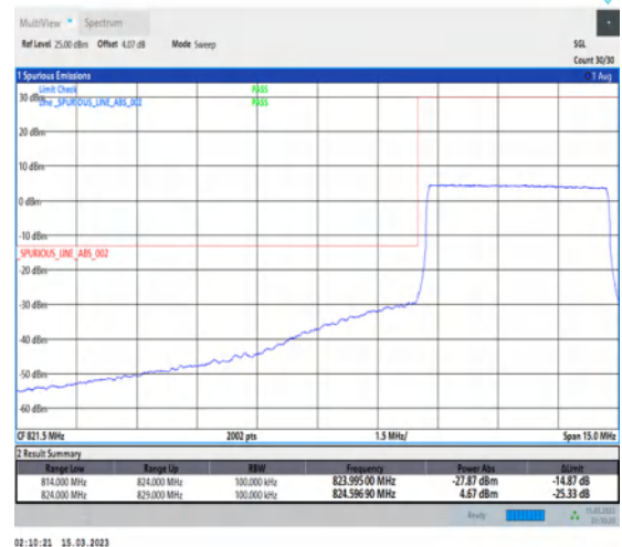
1-N5-PC3-15-5-L-6-CP-QPSK-Outer_Full-25@0-Ant1-1-seegraph-PASS-see graph
