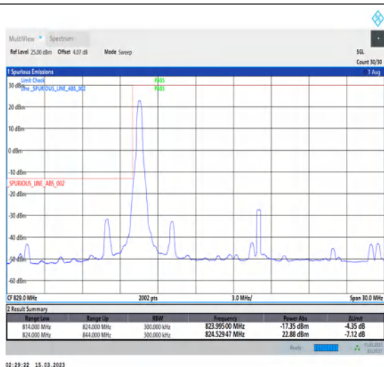
1-N5-PC3-15-20-L-1-DFT-PI2BPSK-Edge_1RB_Left-1@0-Ant1-1-seegraph-PASS-see graph
