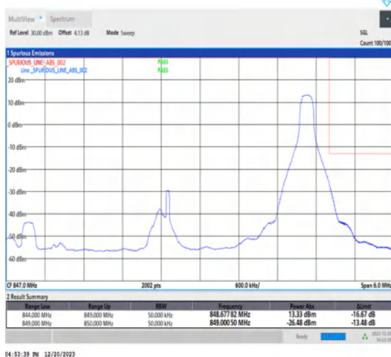
1-N515-5-H-5-CP-QPSK-Edge_1RB_Right-1@24-Ant1-1-seegraph-PASS-see graph
