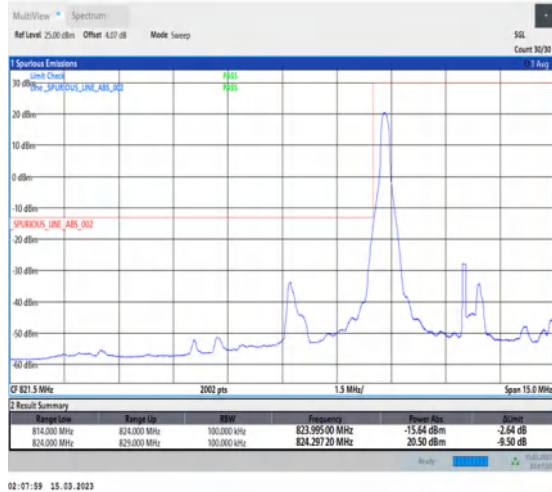
1-N5-PC3-15-5-L-1-DFT-PI2BPSK-Edge_1RB_Left-1@0-Ant1-1-seegraph-PASS-see graph
