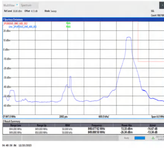
1-N515-5-H-2-DFT-PI2BPSK-Edge_1RB_Right-1@24-Ant1-1-seegraph-PASS-see graph
