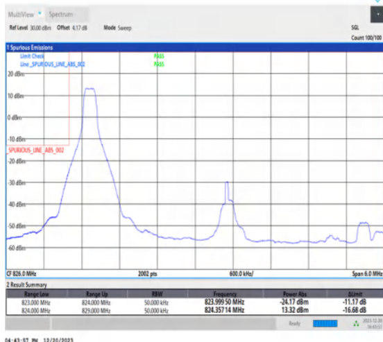
1-N515-5-L-4-CP-QPSK-Edge_1RB_Left-1@0-Ant1-1-seegraph-PASS-see graph
