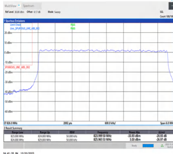
1-N515-5-L-3-DFT-PI2BPSK-Outer_Full-25@0-Ant1-1-seegraph-PASS-see graph
