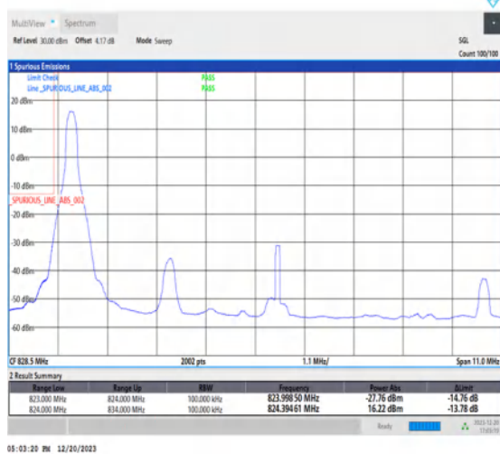
1-N515-10-L-4-CP-QPSK-Edge_1RB_Left-1@0-Ant1-1-seegraph-PASS-see graph
