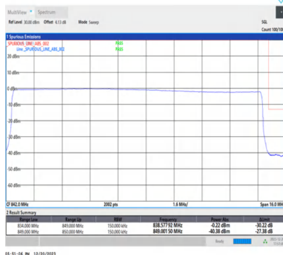
1-N515-15-H-6-CP-QPSK-Outer_Full-79@0-Ant1-1-seegraph-PASS-see graph
