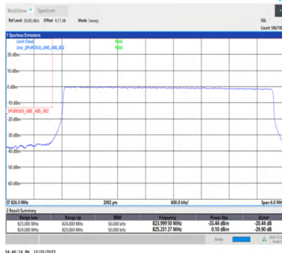
1-N515-5-L-6-CP-QPSK-Outer_Full-25@0-Ant1-1-seegraph-PASS-see graph
