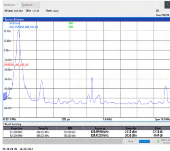
1-N515-15-L-1-DFT-PI2BPSK-Edge_1RB_Left-1@0-Ant1-1-seegraph-PASS-see graph
