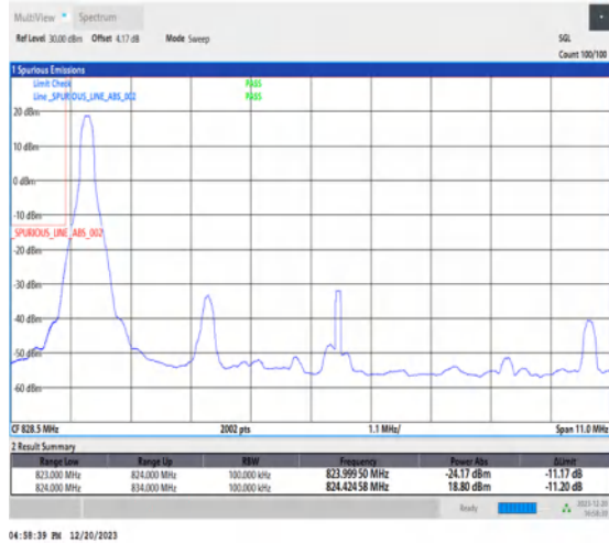
1-N515-10-L-1-DFT-PI2BPSK-Edge_1RB_Left-1@0-Ant1-1-seegraph-PASS-see graph
