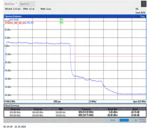
1-N5-PC3-15-10-H-3-DFT-PI2BPSK-Outer_Full-50@0-Ant1-1-seegraph-PASS-see graph
