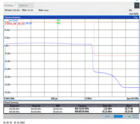
1-N5-PC3-15-20-H-6-CP-QPSK-Outer_Full-106@0-Ant1-1-seegraph-PASS-see graph
