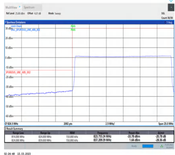
1-N5-PC3-15-15-L-6-CP-QPSK-Outer_Full-79@0-Ant1-1-seegraph-PASS-see graph
