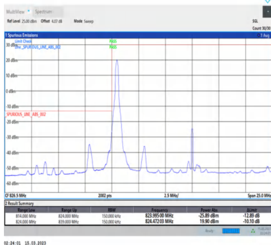
1-N5-PC3-15-15-L-4-CP-QPSK-Edge_1RB_Left-1@0-Ant1-1-seegraph-PASS-see graph
