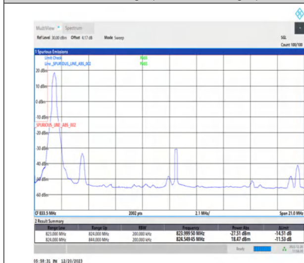
1-N515-20-L-4-CP-QPSK-Edge_1RB_Left-1@0-Ant1-1-seegraph-PASS-see graph
