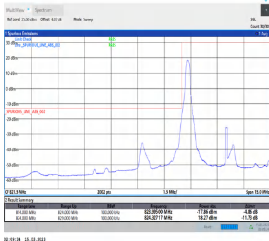
1-N5-PC3-15-5-L-4-CP-QPSK-Edge_1RB_Left-1@0-Ant1-1-seegraph-PASS-see graph
