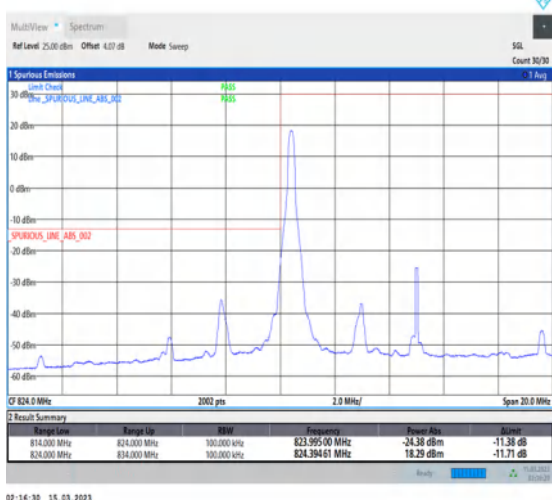
1-N5-PC3-15-10-L-4-CP-QPSK-Edge_1RB_Left-1@0-Ant1-1-seegraph-PASS-see graph
