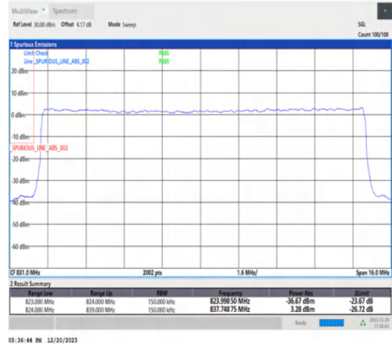
1-N515-15-L-3-DFT-PI2BPSK-Outer_Full-75@0-Ant1-1-seegraph-PASS-see graph
