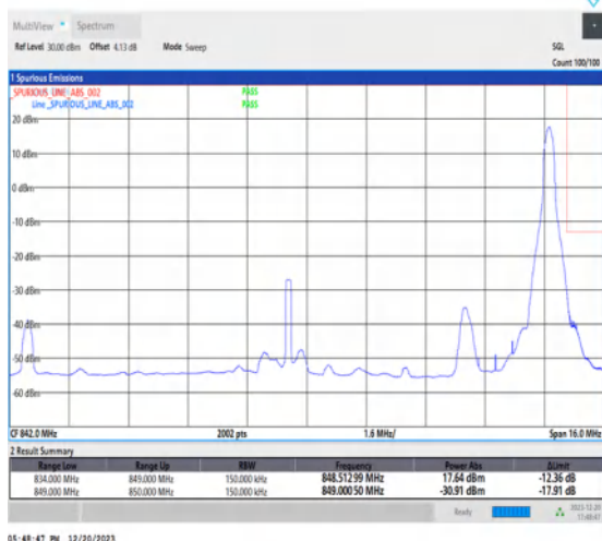
1-N515-15-H-5-CP-QPSK-Edge_1RB_Right-1@78-Ant1-1-seegraph-PASS-see graph
