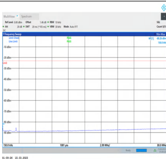
1-N5-PC3-15-20-M-1-DFT-PI2BPSK- Inner_1RB_Left-1@1-0.15-30-Ant1-0.15--85.26--23- PASS
