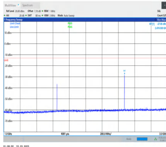
1-N5-PC3-15-20-L-1-DFT-PI2BPSK-Inner_1RB_Left- 1@1-1000-3000-Ant1-2474.50--27.85--13-PASS
