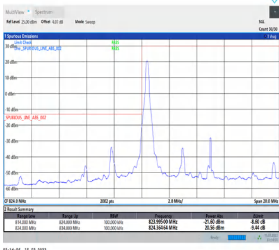
1-N5-PC3-15-10-L-1-DFT-PI2BPSK-Edge_1RB_Left-1@0-Ant1-1-seegraph-PASS-see graph
