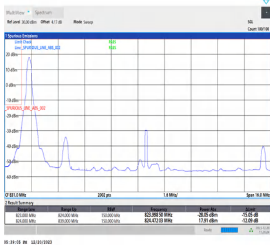
1-N515-15-L-4-CP-QPSK-Edge_1RB_Left-1@0-Ant1-1-seegraph-PASS-see graph
