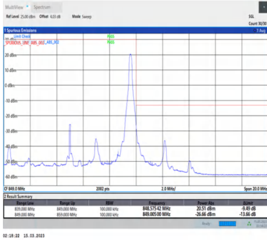
1-N5-PC3-15-10-H-2-DFT-PI2BPSK-Edge_1RB_Right-1@51-Ant1-1-seegraph-PASS-see graph
