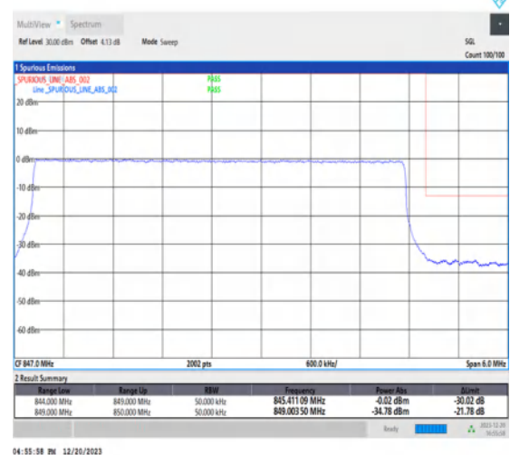
1-N515-5-H-6-CP-QPSK-Outer_Full-25@0-Ant1-1-seegraph-PASS-see graph
