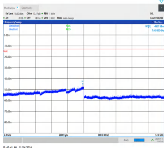
1-N5-15-20-H-1-DFT-PI2BPSK-Inner_1RB_Left- 1@1-3000-12000-Ant1-7489.65--45.97--13-PASS
