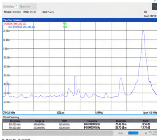
1-N515-15-H-2-DFT-PI2BPSK-Edge_1RB_Right-1@78-Ant1-1-seegraph-PASS-see graph
