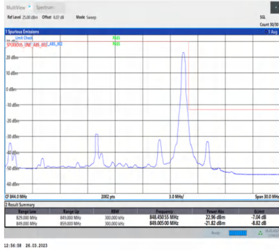
1-N5-PC3-15-20-H-2-DFT-PI2BPSK-Edge_1RB_Right-1@105-Ant1-1-seegraph-PASS-see graph
