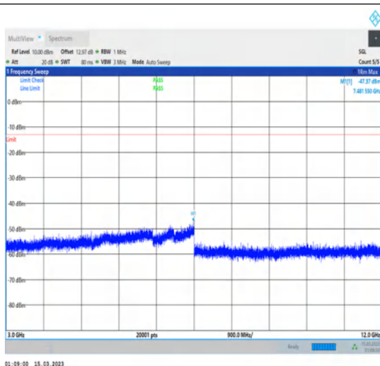
1-N5-PC3-15-20-L-1-DFT-PI2BPSK- Inner_1RB_Left-1@1-3000-12000-Ant1-7481.55-- 47.37--13-PASS
