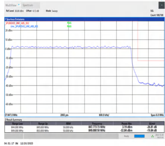
1-N515-5-H-3-DFT-PI2BPSK-Outer_Full-25@0-Ant1-1-seegraph-PASS-see graph
