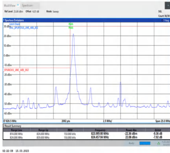
1-N5-PC3-15-15-L-1-DFT-PI2BPSK-Edge_1RB_Left-1@0-Ant1-1-seegraph-PASS-see graph
