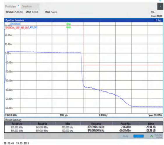
1-N5-PC3-15-10-H-6-CP-QPSK-Outer_Full-52@0-Ant1-1-seegraph-PASS-see graph
