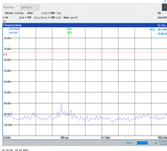
1-N5-PC3-15-20-H-1-DFT-PI2BPSK- Inner_1RB_Left-1@1-0.009-0.15-Ant1-0.06--84.10-- 33-PASS
