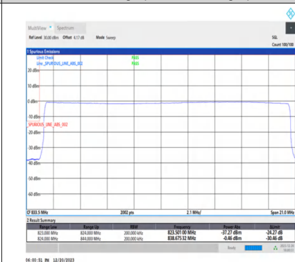
1-N515-20-L-6-CP-QPSK-Outer_Full-106@0-Ant1-1-seegraph-PASS-see graph
