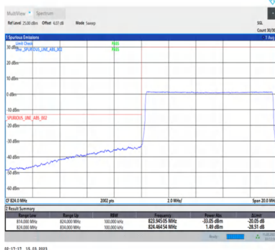
1-N5-PC3-15-10-L-6-CP-QPSK-Outer_Full-52@0-Ant1-1-seegraph-PASS-see graph
