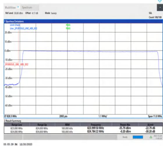
1-N515-10-L-6-CP-QPSK-Outer_Full-52@0-Ant1-1-seegraph-PASS-see graph
