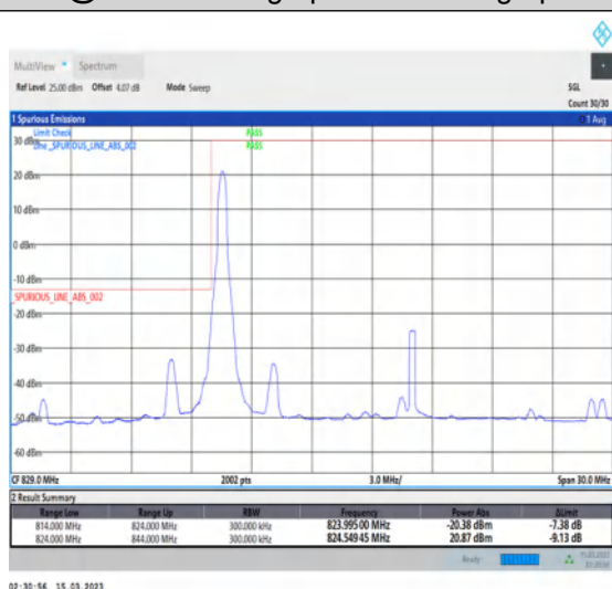
1-N5-PC3-15-20-L-4-CP-QPSK-Edge_1RB_Left-1@0-Ant1-1-seegraph-PASS-see graph
