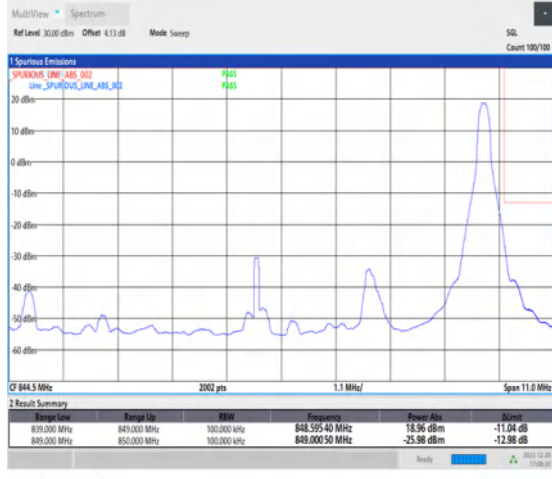
1-N515-10-H-2-DFT-PI2BPSK-Edge_1RB_Right-1@51-Ant1-1-seegraph-PASS-see graph
