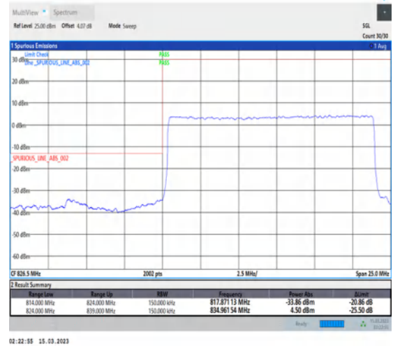
1-N5-PC3-15-15-L-3-DFT-PI2BPSK-Outer_Full-75@0-Ant1-1-seegraph-PASS-see graph
