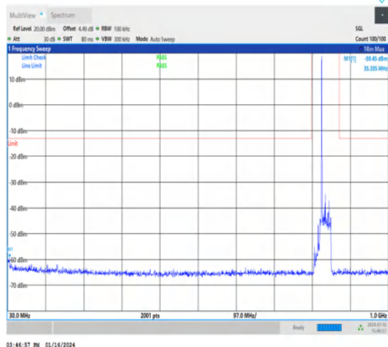
1-N5-15-20-H-1-DFT-PI2BPSK-Inner_1RB_Left- 1@1-30-1000-Ant1-32.91--59.45--13-PASS
