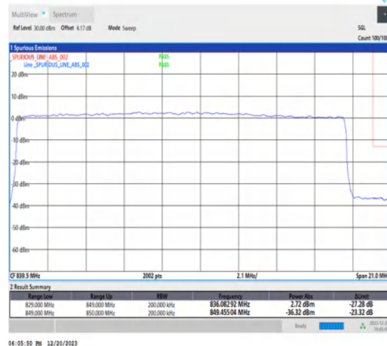
1-N515-20-H-3-DFT-PI2BPSK-Outer_Full-100@0-Ant1-1-seegraph-PASS-see graph
