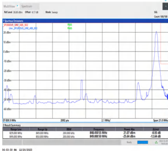
1-N515-20-H-2-DFT-PI2BPSK-Edge_1RB_Right-1@105-Ant1-1-seegraph-PASS-see graph
