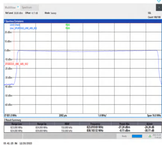
1-N515-15-L-6-CP-QPSK-Outer_Full-79@0-Ant1-1-seegraph-PASS-see graph
