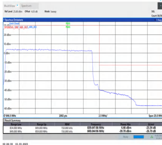
1-N5-PC3-15-15-H-3-DFT-PI2BPSK-Outer_Full-75@0-Ant1-1-seegraph-PASS-see graph
