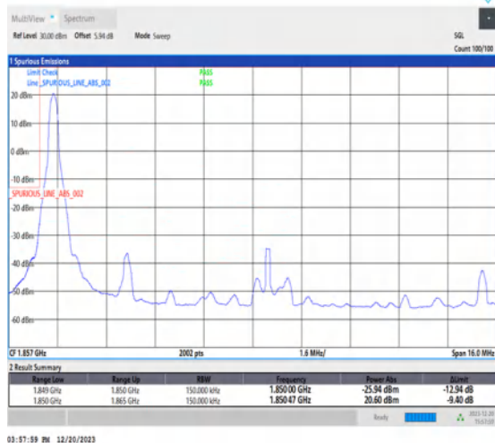
1-N2-15-15-L-1-DFT-PI2BPSK-Edge_1RB_Left-1@0-Ant1-1-seegraph-PASS-see graph
