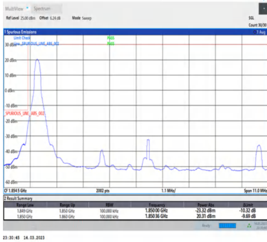
1-N2-PC3-15-10-L-1-DFT-PI2BPSK-Edge_1RB_Left-1@0-Ant1-1-seegraph-PASS-see graph
