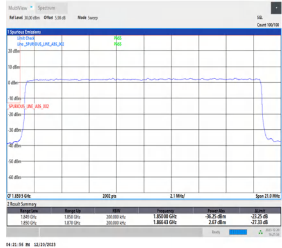
1-N2-15-20-L-3-DFT-PI2BPSK-Outer_Full-100@0-Ant1-1-seegraph-PASS-see graph
