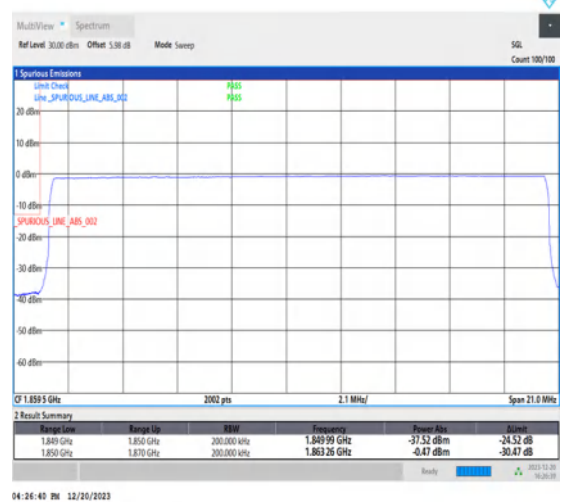
1-N2-15-20-L-6-CP-QPSK-Outer_Full-106@0-Ant1-1-seegraph-PASS-see graph
