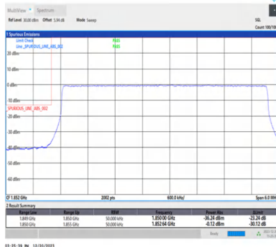
1-N2-15-5-L-6-CP-QPSK-Outer_Full-25@0-Ant1-1-seegraph-PASS-see graph
