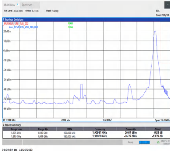
1-N2-15-15-H-2-DFT-PI2BPSK-Edge_1RB_Right-1@78-Ant1-1-seegraph-PASS-see graph
