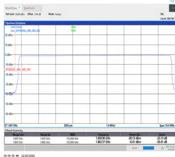
1-N2-15-15-L-6-CP-QPSK-Outer_Full-79@0-Ant1-1-seegraph-PASS-see graph
