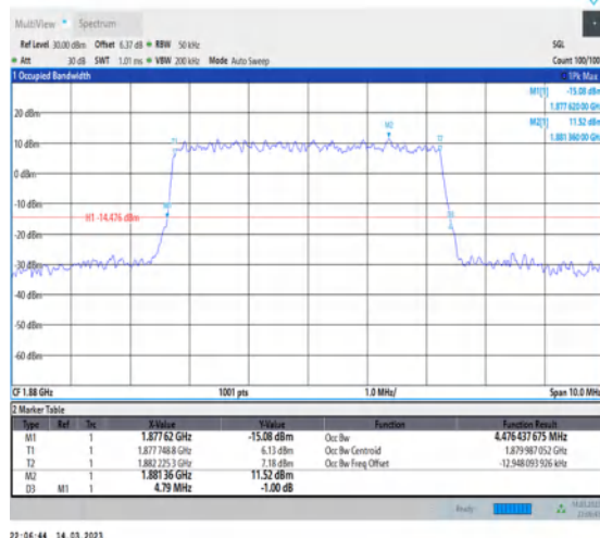
1-N2-PC3-15-5-M-3-DFT-16QAM-Outer_Full-25@0-Ant1-4.476-4.790-≤5-PASS
