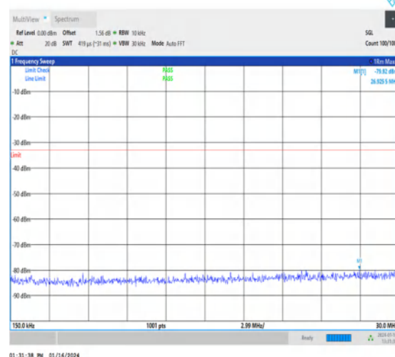
1-N2-15-20-M-1-DFT-PI2BPSK-Inner_1RB_Left-1@1-0.15-30-Ant1-29.97--79.92--33-PASS
