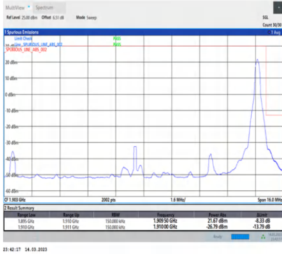
1-N2-PC3-15-15-H-2-DFT-PI2BPSK-Edge_1RB_Right-1@78-Ant1-1-seegraph-PASS-see graph
