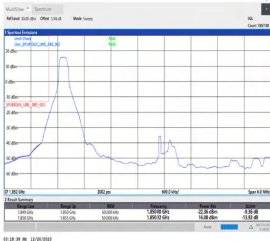
1-N2-15-5-L-1-DFT-PI2BPSK-Edge_1RB_Left-1@0-Ant1-1-seegraph-PASS-see graph
