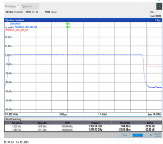
1-N2-PC3-15-10-H-6-CP-QPSK-Outer_Full-52@0-Ant1-1-seegraph-PASS-see graph
