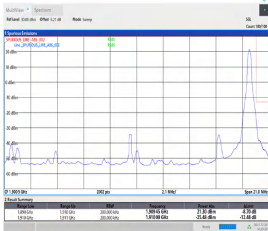
1-N2-15-20-H-2-DFT-PI2BPSK-Edge_1RB_Right-1@105-Ant1-1-seegraph-PASS-see graph
