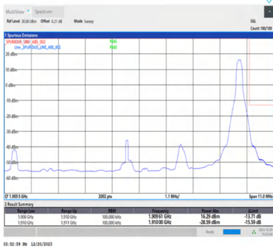
1-N2-15-10-H-5-CP-QPSK-Edge_1RB_Right-1@51-Ant1-1-seegraph-PASS-see graph
