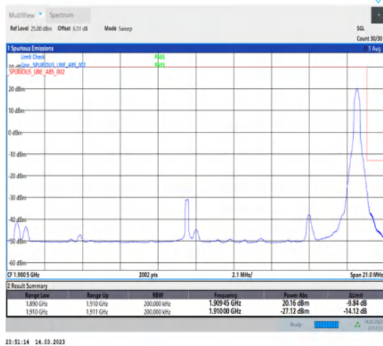
1-N2-PC3-15-20-H-5-CP-QPSK-Edge_1RB_Right-1@105-Ant1-1-seegraph-PASS-see graph
