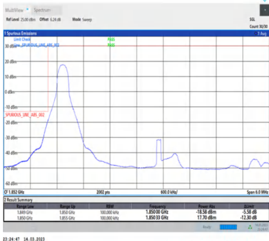
1-N2-PC3-15-5-L-4-CP-QPSK-Edge_1RB_Left-1@0-Ant1-1-seegraph-PASS-see graph
