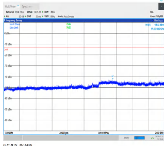
1-N2-15-20-H-1-DFT-PI2BPSK-Inner_1RB_Left-1@1-12000-20000-Ant1-16940.40--43.02--13-PASS
