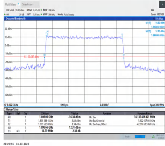
1-N2-PC3-15-15-H-6-CP-QPSK-Outer_Full-79@0-Ant1-14.137-14.790-≤15-PASS
