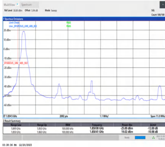
1-N2-15-10-L-1-DFT-PI2BPSK-Edge_1RB_Left-1@0-Ant1-1-seegraph-PASS-see graph
