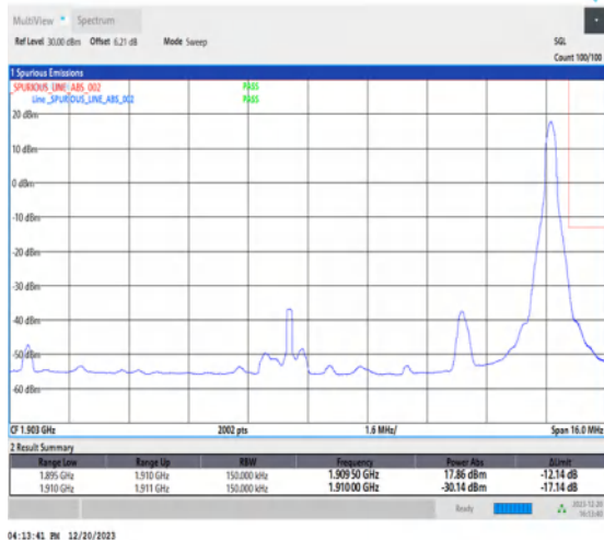
1-N2-15-15-H-5-CP-QPSK-Edge_1RB_Right-1@78-Ant1-1-seegraph-PASS-see graph
