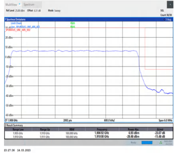
1-N2-PC3-15-5-H-3-DFT-PI2BPSK-Outer_Full-25@0-Ant1-1-seegraph-PASS-see graph
