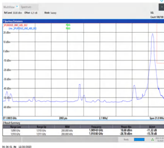
1-N2-15-20-H-5-CP-QPSK-Edge_1RB_Right-1@105-Ant1-1-seegraph-PASS-see graph
