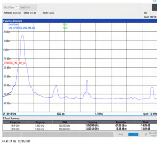
1-N2-15-10-L-4-CP-QPSK-Edge_1RB_Left-1@0-Ant1-1-seegraph-PASS-see graph
