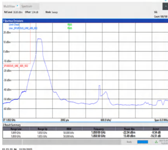
1-N2-15-5-L-4-CP-QPSK-Edge_1RB_Left-1@0-Ant1-1-seegraph-PASS-see graph
