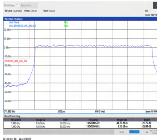
1-N2-15-5-L-3-DFT-PI2BPSK-Outer_Full-25@0-Ant1-1-seegraph-PASS-see graph
