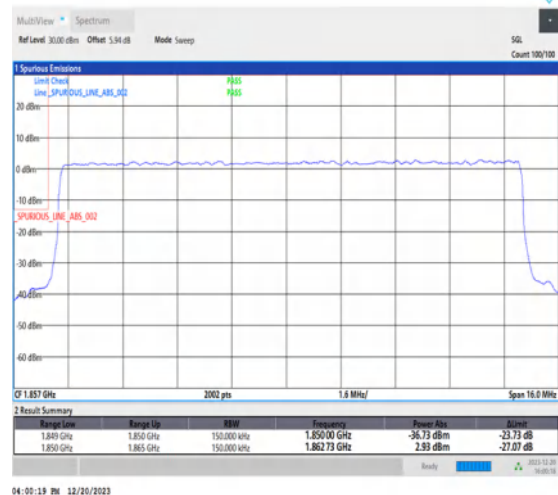
1-N2-15-15-L-3-DFT-PI2BPSK-Outer_Full-75@0-Ant1-1-seegraph-PASS-see graph
