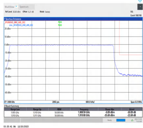
1-N2-15-5-H-6-CP-QPSK-Outer_Full-25@0-Ant1-1-seegraph-PASS-see graph
