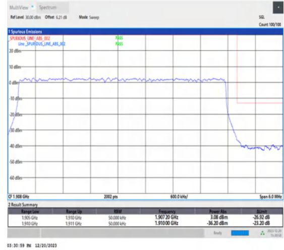
1-N2-15-5-H-3-DFT-PI2BPSK-Outer_Full-25@0-Ant1-1-seegraph-PASS-see graph
