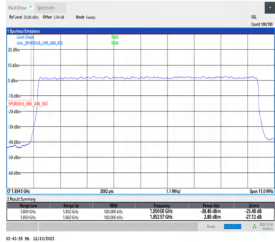
1-N2-15-10-L-3-DFT-PI2BPSK-Outer_Full-50@0-Ant1-1-seegraph-PASS-see graph
