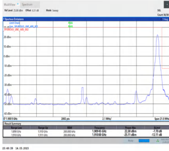
1-N2-PC3-15-20-H-2-DFT-PI2BPSK-Edge_1RB_Right-1@105-Ant1-1-seegraph-PASS-see graph
