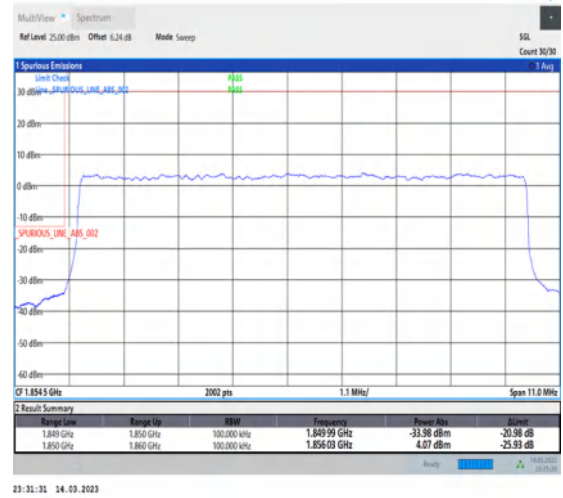
1-N2-PC3-15-10-L-3-DFT-PI2BPSK-Outer_Full-50@0-Ant1-1-seegraph-PASS-see graph
