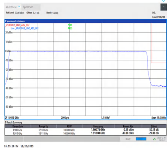
1-N2-15-10-H-6-CP-QPSK-Outer_Full-52@0-Ant1-1-seegraph-PASS-see graph
