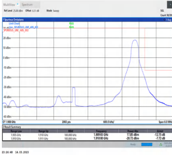
1-N2-PC3-15-5-H-2-DFT-PI2BPSK-Edge_1RB_Right-1@24-Ant1-1-seegraph-PASS-see graph
