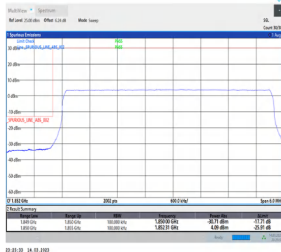
1-N2-PC3-15-5-L-6-CP-QPSK-Outer_Full-25@0-Ant1-1-seegraph-PASS-see graph
