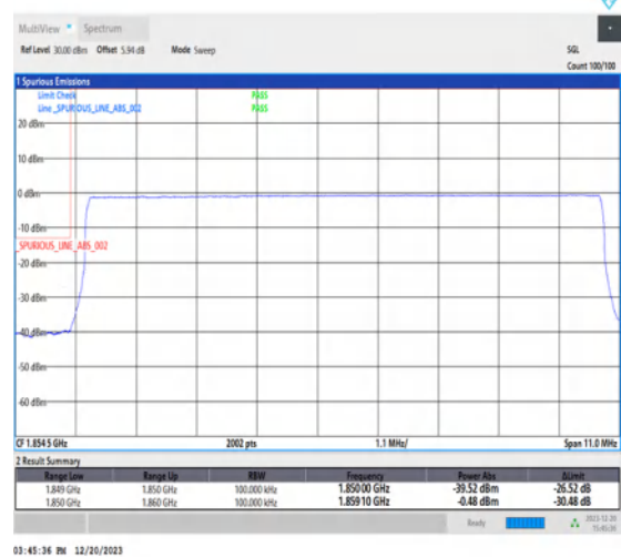
1-N2-15-10-L-6-CP-QPSK-Outer_Full-52@0-Ant1-1-seegraph-PASS-see graph
