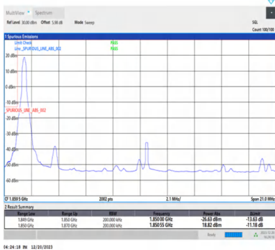
1-N2-15-20-L-4-CP-QPSK-Edge_1RB_Left-1@0-Ant1-1-seegraph-PASS-see graph
