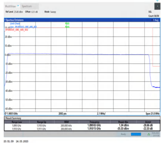
1-N2-PC3-15-20-H-6-CP-QPSK-Outer_Full-106@0-Ant1-1-seegraph-PASS-see graph
