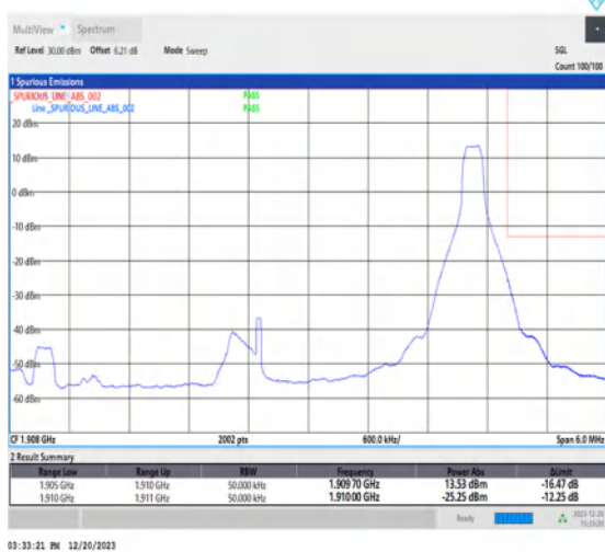
1-N2-15-5-H-5-CP-QPSK-Edge_1RB_Right-1@24-Ant1-1-seegraph-PASS-see graph
