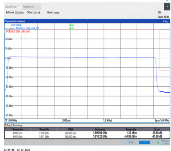
1-N2-PC3-15-15-H-6-CP-QPSK-Outer_Full-79@0-Ant1-1-seegraph-PASS-see graph
