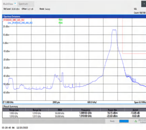
1-N2-15-5-H-2-DFT-PI2BPSK-Edge_1RB_Right-1@24-Ant1-1-seegraph-PASS-see graph
