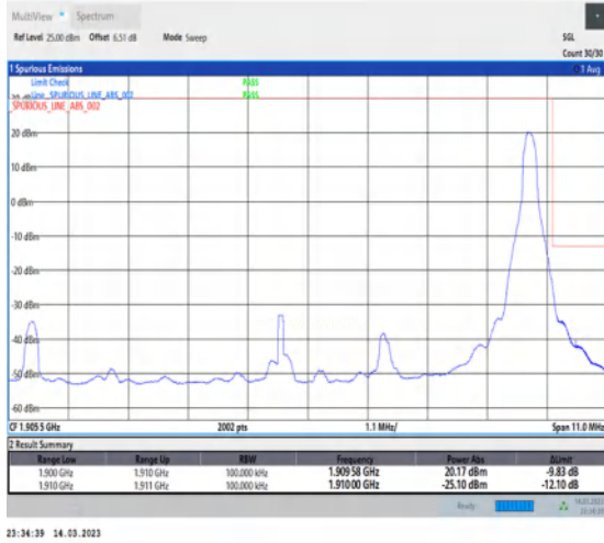
1-N2-PC3-15-10-H-2-DFT-PI2BPSK-Edge_1RB_Right-1@51-Ant1-1-seegraph-PASS-see graph
