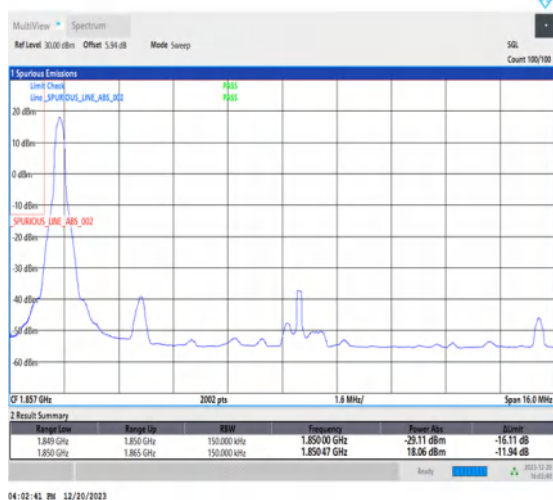
1-N2-15-15-L-4-CP-QPSK-Edge_1RB_Left-1@0-Ant1-1-seegraph-PASS-see graph
