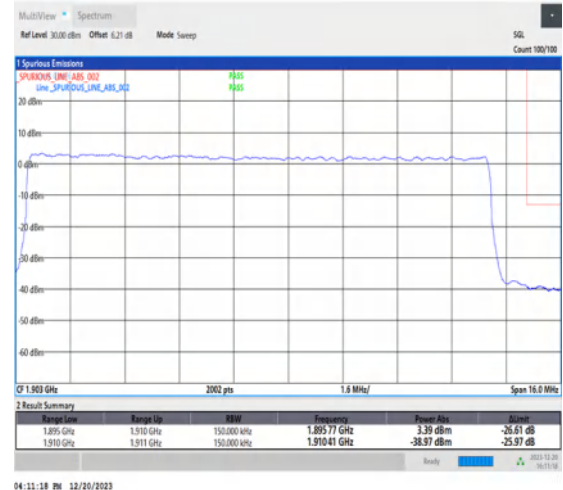
1-N2-15-15-H-3-DFT-PI2BPSK-Outer_Full-75@0-Ant1-1-seegraph-PASS-see graph
