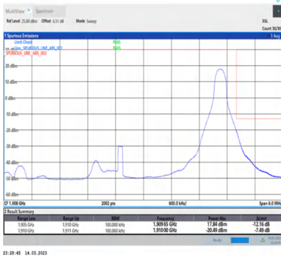
1-N2-PC3-15-5-H-5-CP-QPSK-Edge_1RB_Right-1@24-Ant1-1-seegraph-PASS-see graph
