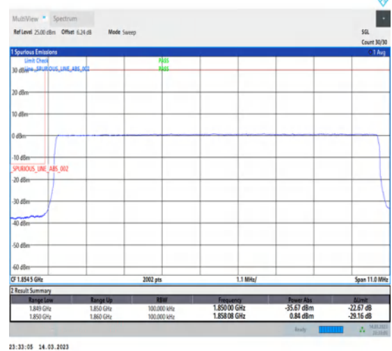
1-N2-PC3-15-10-L-6-CP-QPSK-Outer_Full-52@0-Ant1-1-seegraph-PASS-see graph
