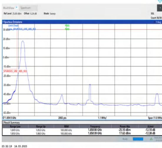
1-N2-PC3-15-10-L-4-CP-QPSK-Edge_1RB_Left-1@0-Ant1-1-seegraph-PASS-see graph
