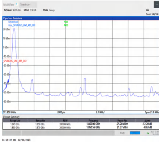
1-N2-15-20-L-1-DFT-PI2BPSK-Edge_1RB_Left-1@0-Ant1-1-seegraph-PASS-see graph
