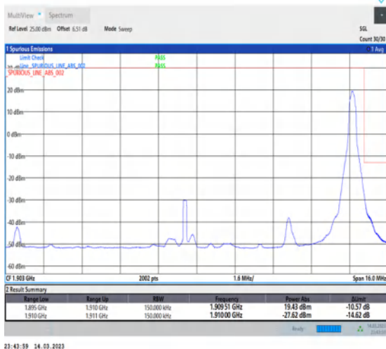
1-N2-PC3-15-15-H-5-CP-QPSK-Edge_1RB_Right-1@78-Ant1-1-seegraph-PASS-see graph
