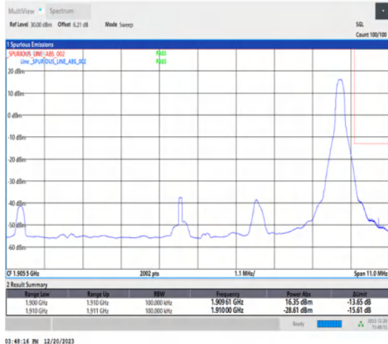
1-N2-15-10-H-2-DFT-PI2BPSK-Edge_1RB_Right-1@51-Ant1-1-seegraph-PASS-see graph
