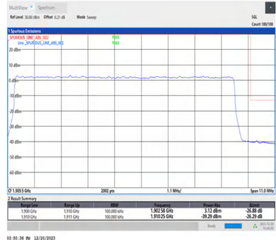
1-N2-15-10-H-3-DFT-PI2BPSK-Outer_Full-50@0-Ant1-1-seegraph-PASS-see graph
