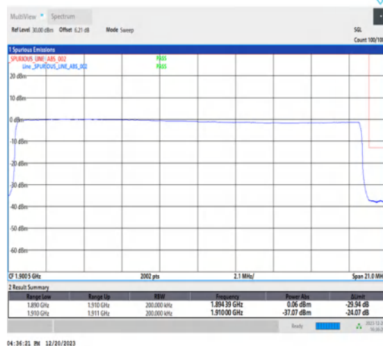
1-N2-15-20-H-6-CP-QPSK-Outer_Full-106@0-Ant1-1-seegraph-PASS-see graph
