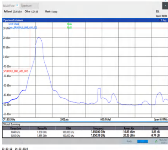
1-N2-PC3-15-5-L-1-DFT-PI2BPSK-Edge_1RB_Left-1@0-Ant1-1-seegraph-PASS-see graph
