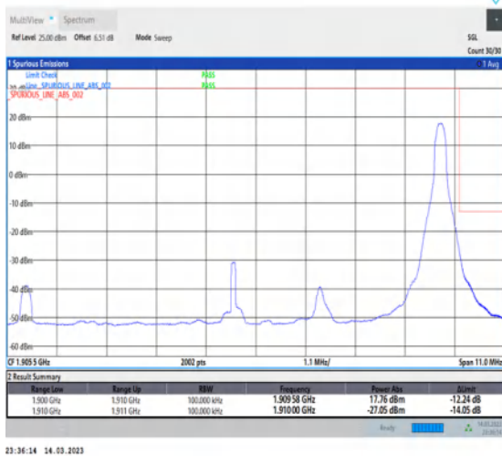
1-N2-PC3-15-10-H-5-CP-QPSK-Edge_1RB_Right-1@51-Ant1-1-seegraph-PASS-see graph
