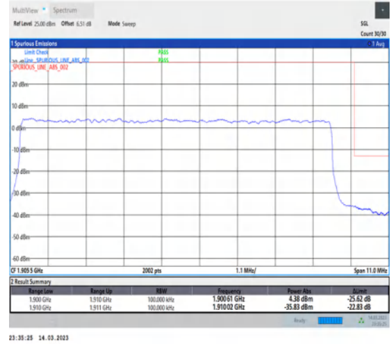
1-N2-PC3-15-10-H-3-DFT-PI2BPSK-Outer_Full-50@0-Ant1-1-seegraph-PASS-see graph
