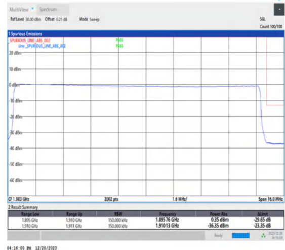
1-N2-15-15-H-6-CP-QPSK-Outer_Full-79@0-Ant1-1-seegraph-PASS-see graph
