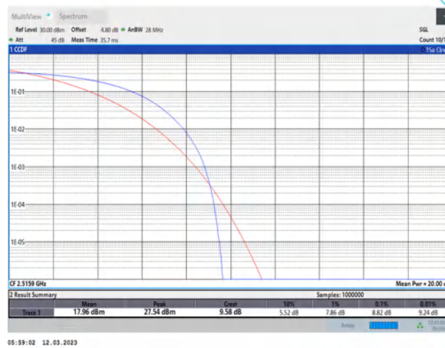
41-41-20MHz-20MHz-QPSK-QPSK-40521-40719-100RB#0-100RB#0
