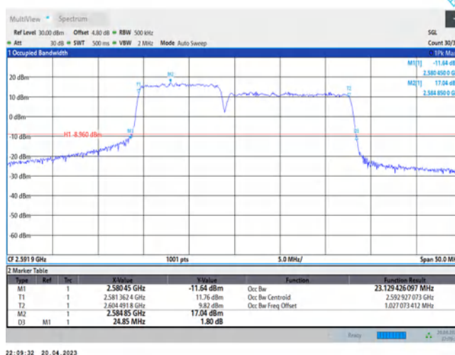
41-41-10MHz-15MHz-QPSK-QPSK-40549-40669-50RB#0-75RB#0
