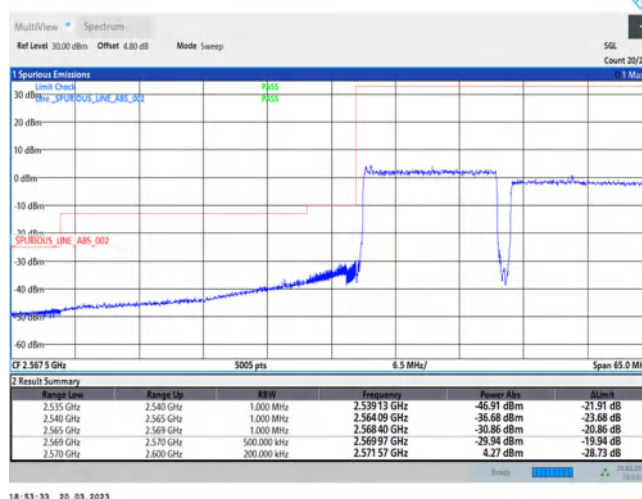
38-38-15MHz-15MHz-QPSK-QPSK-37825-37975-75RB#0-75RB#0
