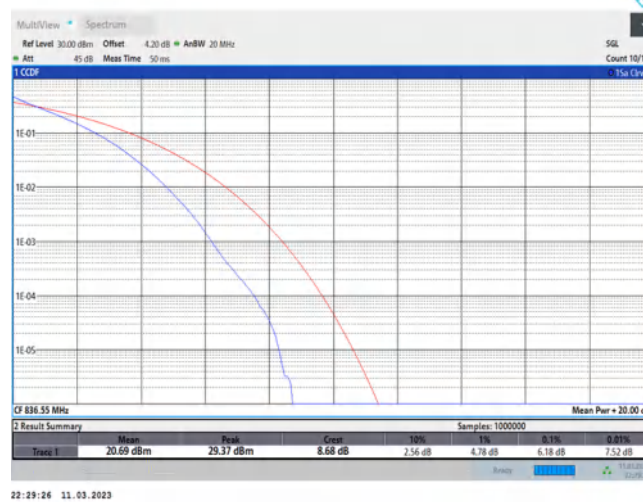
5-5-10MHz-10MHz-QPSK-QPSK-20476-20575-50RB#0-50RB#0
