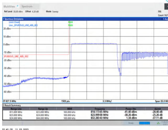
5-5-10MHz-10MHz-QPSK-QPSK-20450-20549-50RB#0-50RB#0
