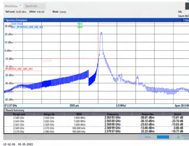
Band38-5MHz-QPSK-37775-25RB#0
