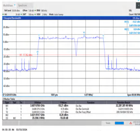
NTNV_CA_n48B_PC3_30+30_20+15_M+M_Ant0_TID7_1_#1
