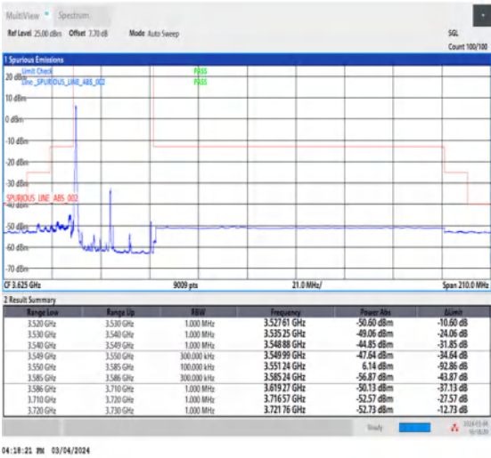
NTNV_CA_n48B_PC3_30+30_15+20_L+L_TID1_1_#1
