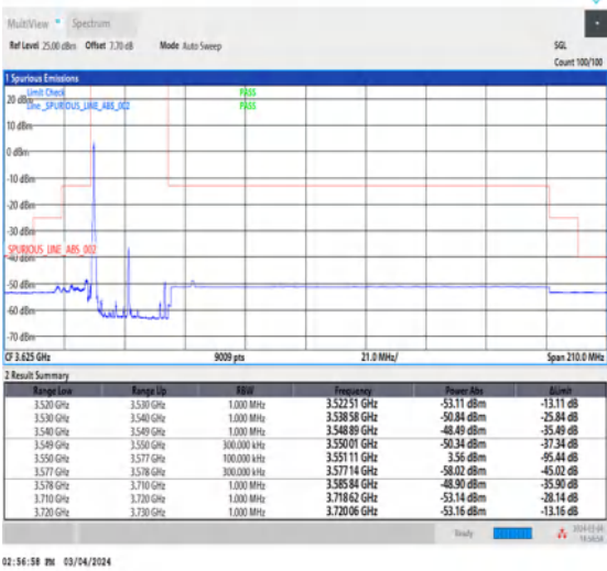
NTNV_CA_n48B_PC3_30+30_15+15_L+L_TID1_1_#1
