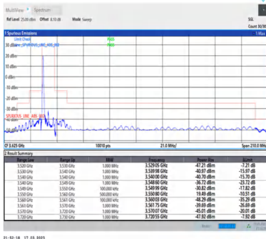
1-N48-PC3-30-10-L-4-CP-QPSK-Edge_1RB_Left-1@0-Ant0-1--PASS-see graph
