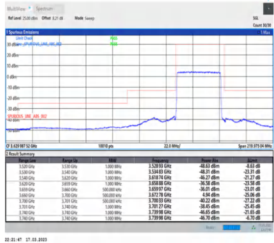
1-N48-PC3-30-40-H-3-DFT-PI2BPSK-Outer_Full-100@0-Ant0-1--PASS-see graph
