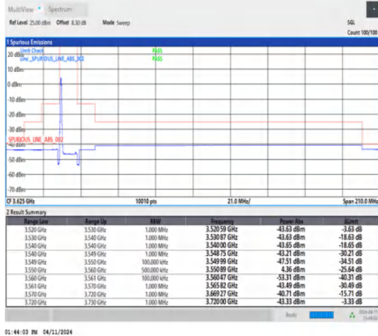
1-N48-30-10-L-1-DFT-PI2BPSK-Edge_1RB_Left-1@0-Ant0-1--PASS-see graph
