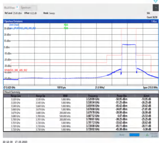
1-N48-PC3-30-20-H-6-CP-QPSK-Outer_Full-51@0-Ant0-1--PASS-see graph
