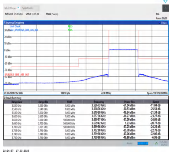
1-N48-PC3-30-40-H-6-CP-QPSK-Outer_Full-106@0-Ant0-1--PASS-see graph
