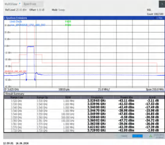
1-N48-30-10-L-3-DFT-PI2BPSK-Outer_Full-24@0-Ant0-1--PASS-see graph
