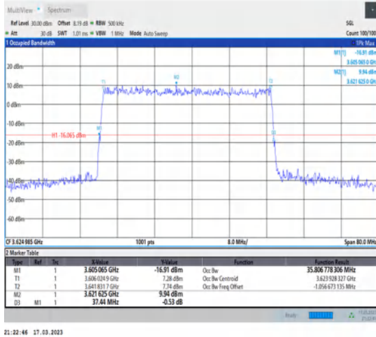
1-N48-PC3-30-40-M-5-DFT-256QAM-Outer_Full-100@0-Ant0-35.807-37.440-≤40-PASS
