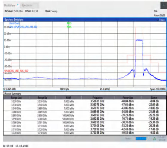
1-N48-PC3-30-10-H-3-DFT-PI2BPSK-Outer_Full-24@0-Ant0-1--PASS-see graph
