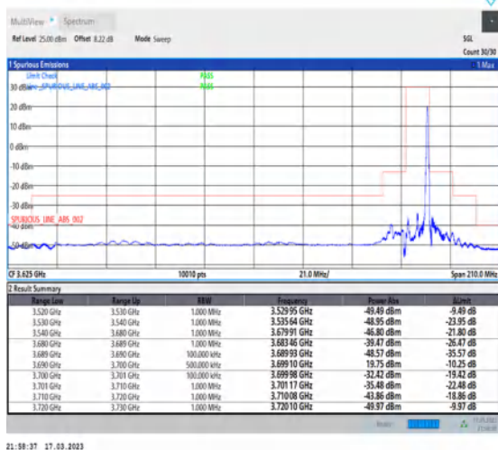
1-N48-PC3-30-10-H-5-CP-QPSK-Edge_1RB_Right-1@23-Ant0-1--PASS-see graph
