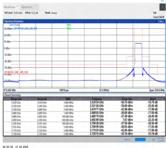
1-N48-PC3-30-10-H-6-CP-QPSK-Outer_Full-24@0-Ant0-1--PASS-see graph
