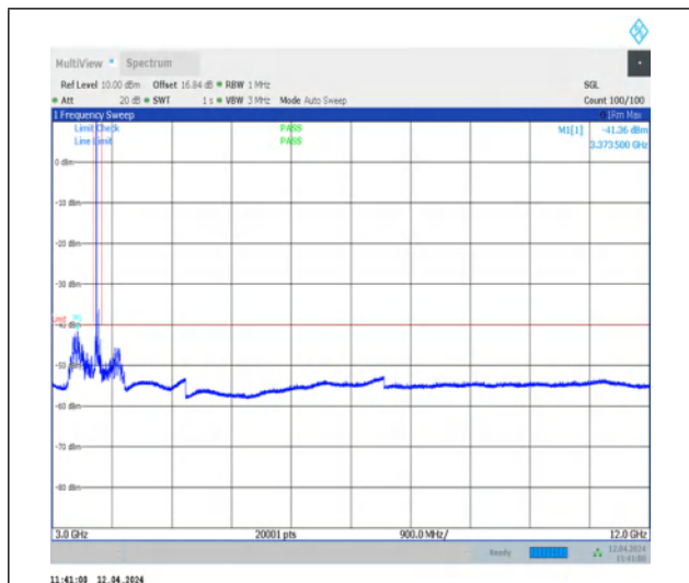
1-N48-30-40-H-1-DFT-QPSK-Edge_1RB_Left- 1@0-3000-12000-Ant0-3373.95--41.36--40-PASS
