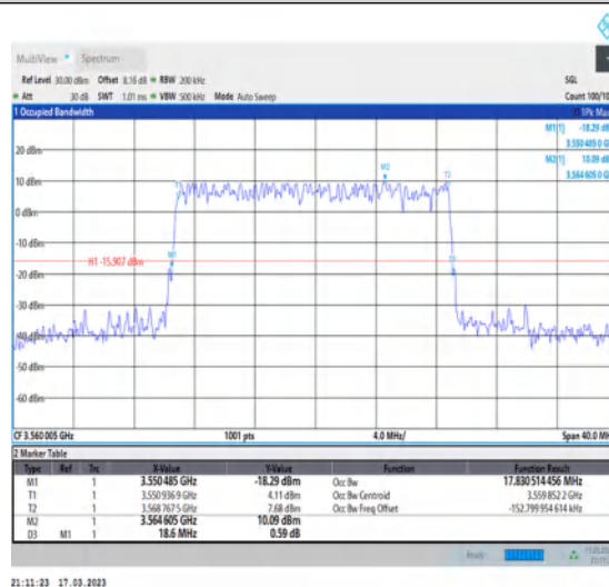
1-N48-PC3-30-20-L-4-DFT-64QAM-Outer_Full-50@0-Ant0-17.831-18.600-≤20-PASS
