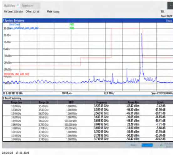
1-N48-PC3-30-40-H-2-DFT-PI2BPSK-Edge_1RB_Right-1@105-Ant0-1--PASS-see graph
