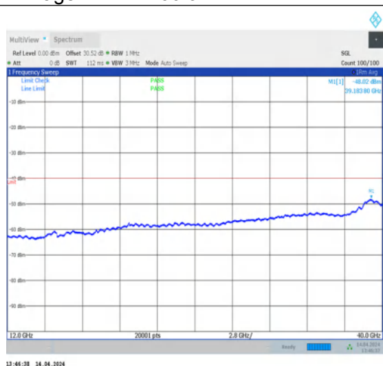
1-N48-PC3-30-40-H-1-DFT-PI2BPSK-Inner_1RB_Left- 1@1-12000-40000-Ant0-12000.00--48.00--40-PASS
