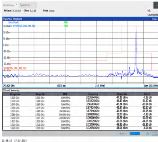
1-N48-PC3-30-20-H-2-DFT-PI2BPSK-Edge_1RB_Right-1@50-Ant0-1--PASS-see graph
