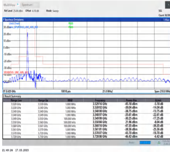
1-N48-PC3-30-10-L-1-DFT-PI2BPSK-Edge_1RB_Left-1@0-Ant0-1--PASS-see graph
