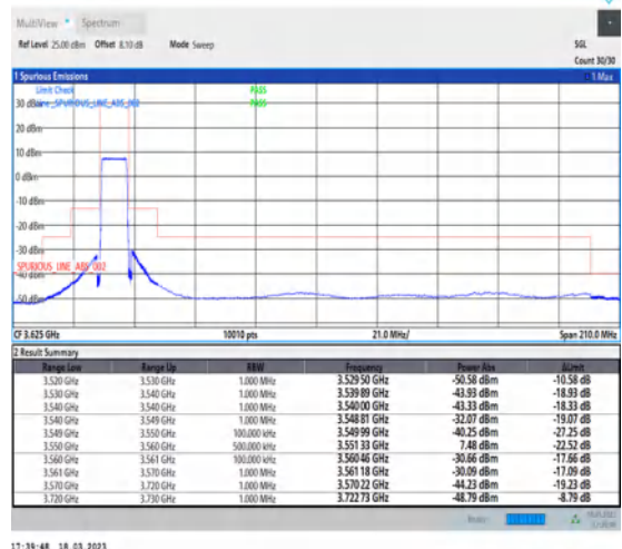
1-N48-PC3-30-10-L-6-CP-QPSK-Outer_Full-24@0-Ant0-1--PASS-see graph
