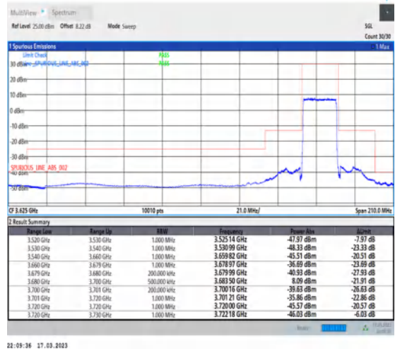
1-N48-PC3-30-20-H-3-DFT-PI2BPSK-Outer_Full-50@0-Ant0-1--PASS-see graph
