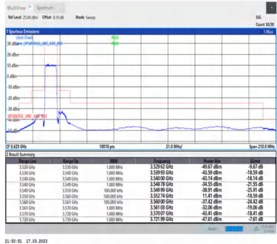
1-N48-PC3-30-10-L-3-DFT-PI2BPSK-Outer_Full-24@0-Ant0-1--PASS-see graph
