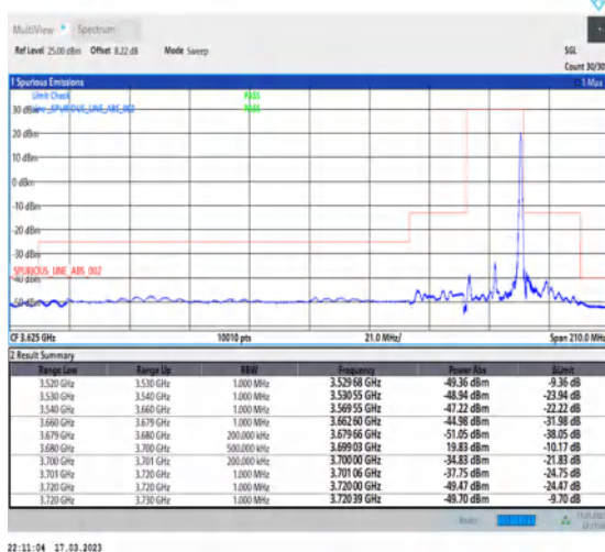
1-N48-PC3-30-20-H-5-CP-QPSK-Edge_1RB_Right-1@50-Ant0-1--PASS-see graph
