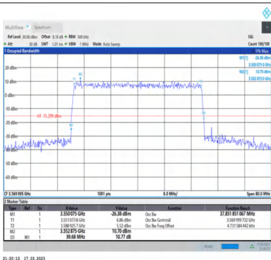
1-N48-PC3-30-40-L-6-CP-QPSK-Outer_Full-106@0-Ant0-37.852-39.680-≤40-PASS
