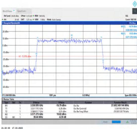
1-N48-PC3-30-40-L-8-CP-64QAM-Outer_Full-106@0-Ant0-37.692-39.440-≤40-PASS
