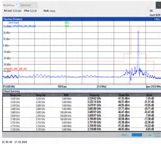
1-N48-PC3-30-10-H-2-DFT-PI2BPSK-Edge_1RB_Right-1@23-Ant0-1--PASS-see graph
