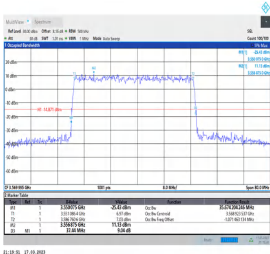
1-N48-PC3-30-40-L-4-DFT-64QAM-Outer_Full-100@0-Ant0-35.674-37.440-≤40-PASS
