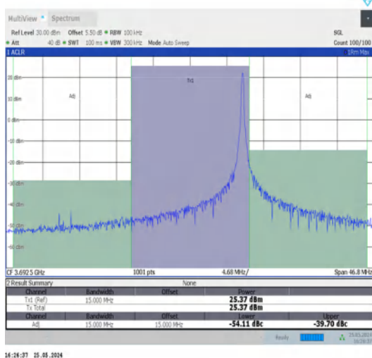
Band48-15MHz-QPSK-56665-1RB#74-PASS
