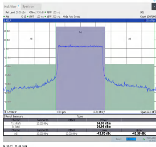
Band48-20MHz-QPSK-56640-100RB#0-PASS
