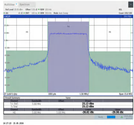
Band48-5MHz-QPSK-56715-25RB#0-PASS
