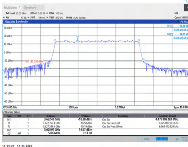
Band48-5MHz-QPSK-55990-25RB#0
