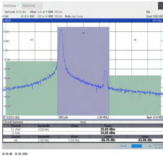
Band48-5MHz-QPSK-55265-1RB#0-PASS
