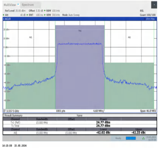
Band48-15MHz-QPSK-55315-75RB#0-PASS
