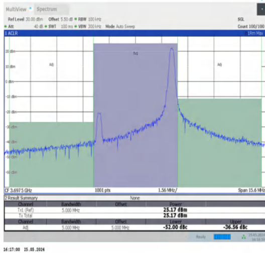
Band48-5MHz-QPSK-56715-1RB#24-PASS
