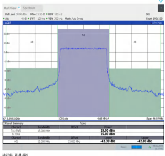
Band48-15MHz-QPSK-56665-75RB#0-PASS
