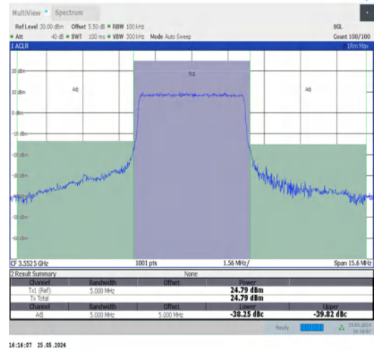
Band48-5MHz-QPSK-55265-25RB#0-PASS
