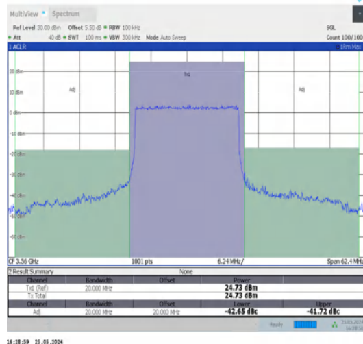
Band48-20MHz-QPSK-55340-100RB#0-PASS
