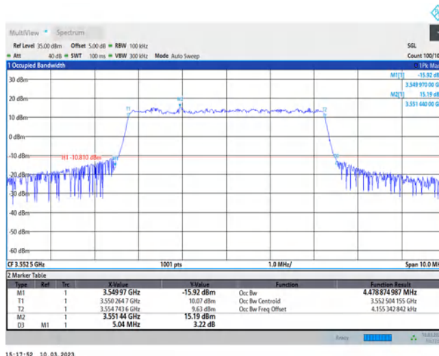
Band48-5MHz-QPSK-55990-25RB#0
