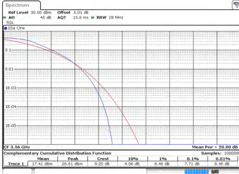
Band48-20MHz-QPSK-55340-100RB#0
