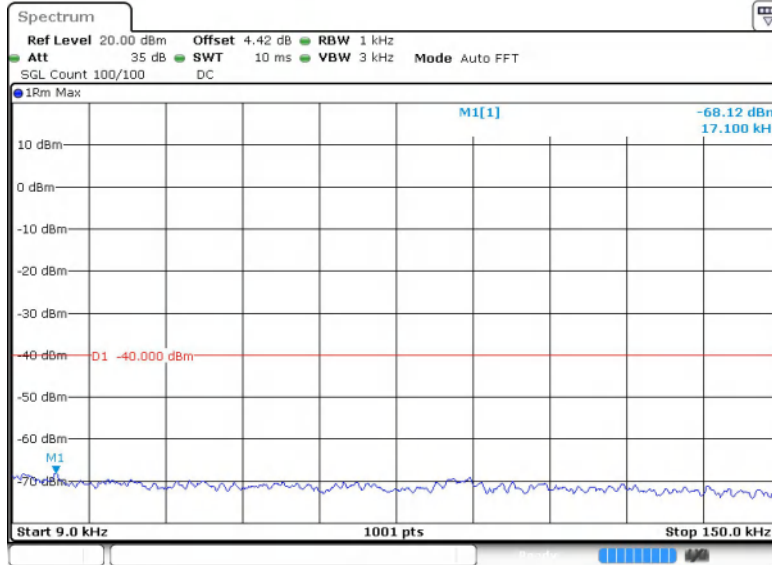
Band48-20MHz-QPSK-55340-1RB#0-Range1:0.009~0.15MHz
