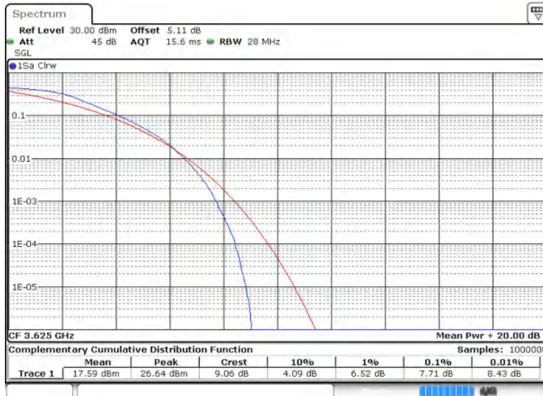
Band48-20MHz-QPSK-55990-100RB#0
