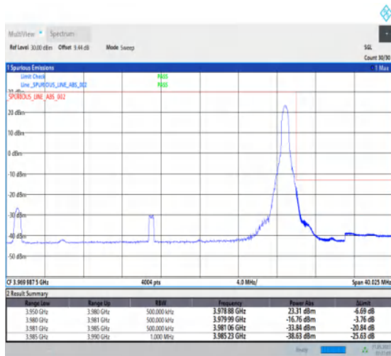
1-N77-3700-3980-PC1-30-30-H-2-DFT-PI2BPSK-Edge_1RB_Right-1@77-Ant1-1--PASS-see graph
