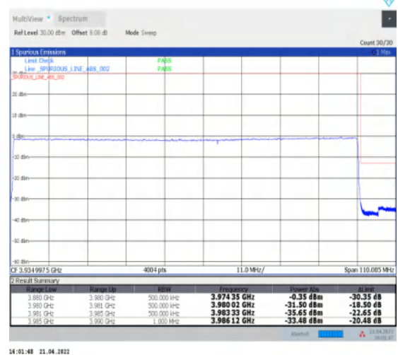
1-N77-3700-3980--30-100-H-6-CP-QPSK-Outer_F ull-273@0-Ant1-PASS-see graph
