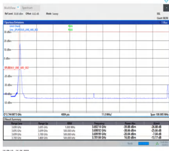
1-N77-3700-3980-PC1-30-100-L-4-CP-QPSK-Edge_1RB_Left-1@0-Ant1-1--PASS-see graph
