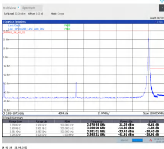
1-N77-3700-3980--30-100-H-5-CP-QPSK-Edge_1RB Right-1@272-Ant1-PASS-see graph
