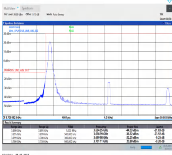
1-N77-3700-3980-PC1-30-30-L-4-CP-QPSK-Edge_1RB_Left-1@0-Ant1-1--PASS-see graph
