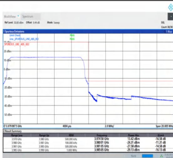
1-N77-3700-3980-PC1-30-10-H-3-DFT-PI2BPSK-Outer_Full-24@0-Ant1-1--PASS-see graph
