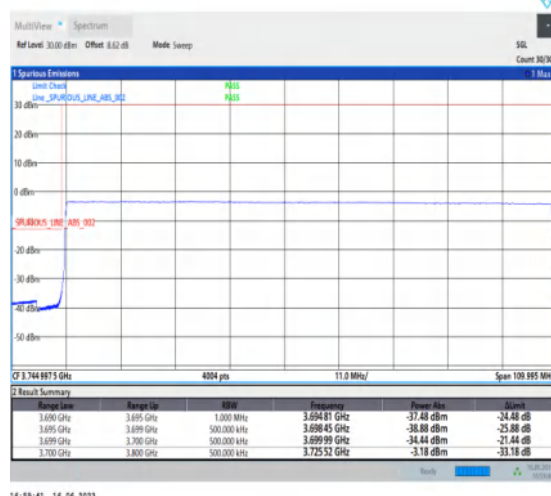
1-N77-3700-3980-PC1-30-100-L-6-CP-QPSK-Outer_Full-273@0-Ant1-1--PASS-see graph
