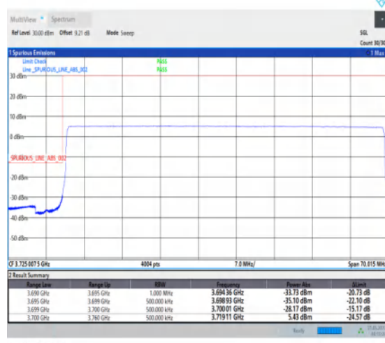
1-N77-3700-3980-PC1-30-60-L-6-CP-QPSK-Outer_Full-162@0-Ant1-1--PASS-see graph
