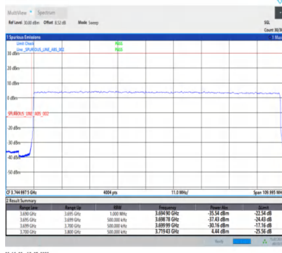
1-N77-3700-3980-PC1-30-100-L-3-DFT-PI2BPSK-Outer_Full-270@0-Ant1-1--PASS-see graph
