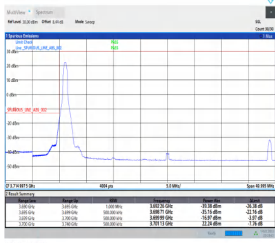
1-N77-3700-3980-PC1-30-40-L-1-DFT-PI2BPSK-Edg e_1RB_Left-1@0-Ant1-1--PASS-see graph
