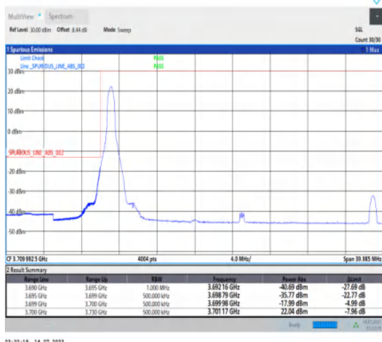
1-N77-3700-3980-PC1-30-30-L-1-DFT-PI2BPSK-Edge_1RB_Left-1@0-Ant1-1--PASS-see graph
