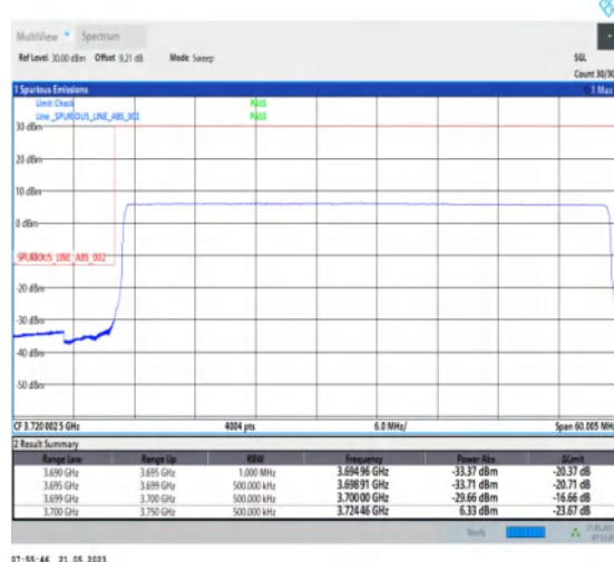
1-N77-3700-3980-PC1-30-50-L-6-CP-QPSK-Outer_ Full-133@0-Ant1-1--PASS-see graph
