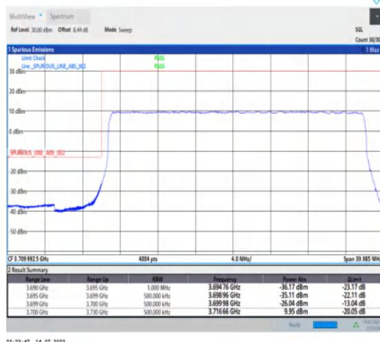
1-N77-3700-3980-PC1-30-30-L-3-DFT-PI2BPSK-Outer_Full-75@0-Ant1-1--PASS-see graph
