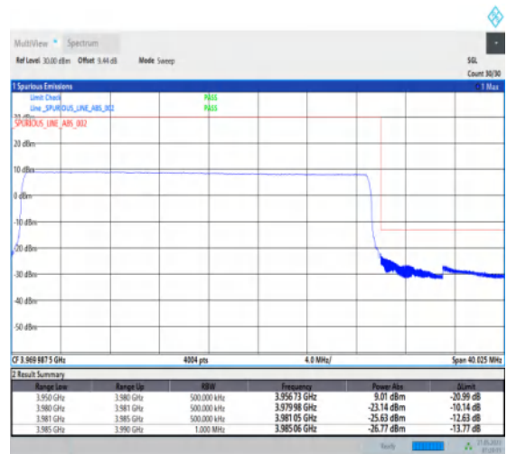
1-N77-3700-3980-PC1-30-30-H-3-DFT-PI2BPSK-Outer_Full-75@0-Ant1-1--PASS-see graph
