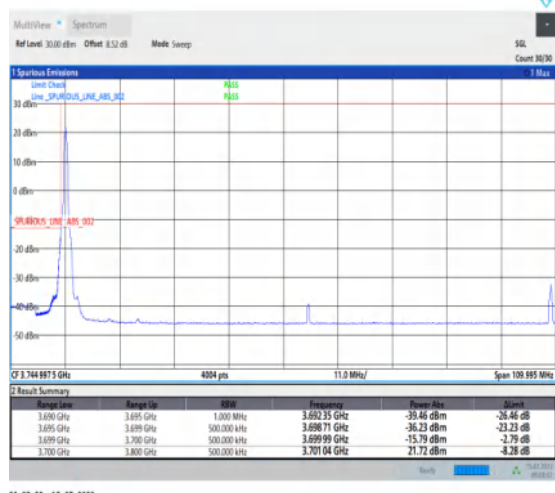
1-N77-3700-3980-PC1-30-100-L-1-DFT-PI2BPSK-Edge_1RB_Left-1@0-Ant1-1--PASS-see graph
