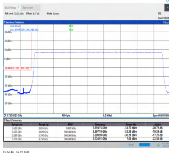
1-N77-3700-3980-PC1-30-50-L-3-DFT-PI2BPSK-O uter_Full-128@0-Ant1-1--PASS-see graph
