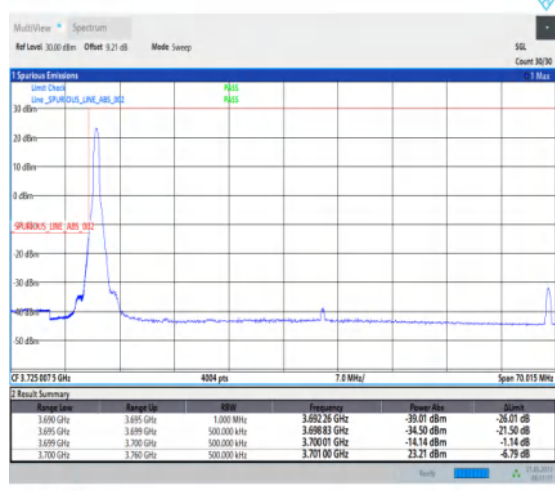
1-N77-3700-3980-PC1-30-60-L-4-CP-QPSK-Edge_1RB_Left-1@0-Ant1-1--PASS-see graph
