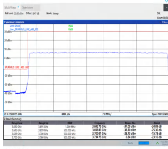
1-N77-3700-3980-PC1-30-60-L-3-DFT-PI2BPSK-Outer_Full-162@0-Ant1-1--PASS-see graph
