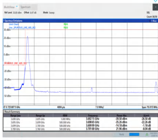
1-N77-3700-3980-PC1-30-60-L-1-DFT-PI2BPSK-Edg_e_1RB_Left-1@0-Ant1-1--PASS-see graph
