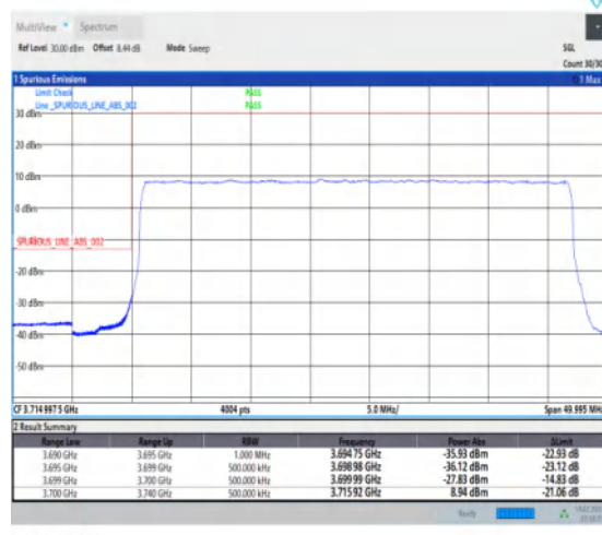
1-N77-3700-3980-PC1-30-40-L-3-DFT-PI2BPSK-O uter_Full-100@0-Ant1-1--PASS-see graph
