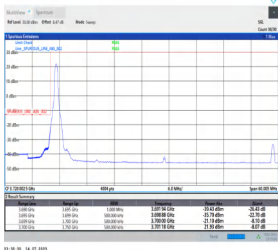
1-N77-3700-3980-PC1-30-50-L-1-DFT-PI2BPSK-Edg e_1RB_Left-1@0-Ant1-1--PASS-see graph
