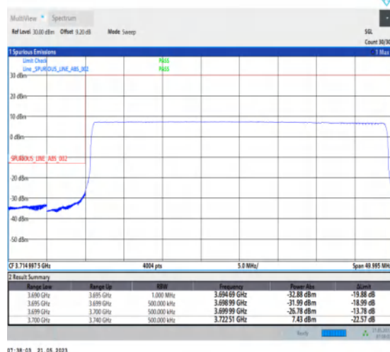
1-N77-3700-3980-PC1-30-40-L-6-CP-QPSK-Outer_ Full-106@0-Ant1-1--PASS-see graph
