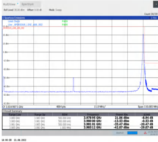
1-N77-3700-3980--30-100-H-2-DFT-PI2BPSK-Edge_1 RB_Right-1@272-Ant1-PASS-see graph
