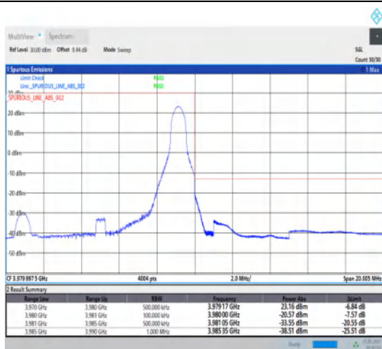
1-N77-3700-3980-PC1-30-10-H-2-DFT-PI2BPSK-Edge_1RB_Right-1@23-Ant1-1--PASS-see graph
