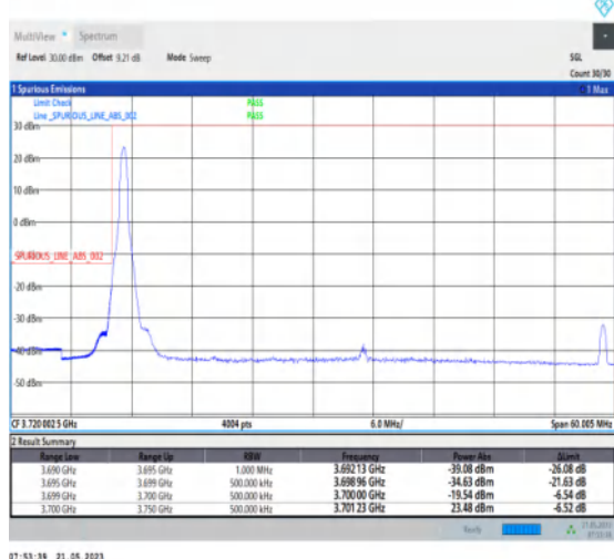
1-N77-3700-3980-PC1-30-50-L-4-CP-QPSK-Edge_1 RB_Left-1@0-Ant1-1--PASS-see graph
