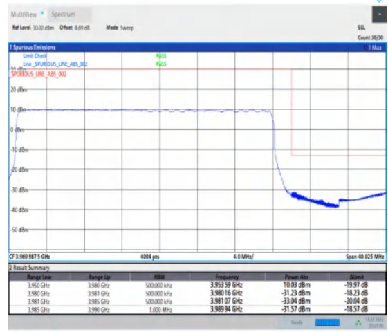
1-N77-3700-3980-PC1-30-30-H-3-DFT-PI2BPSK-Outer_Full-75@0-Ant1-1--PASS-see graph
