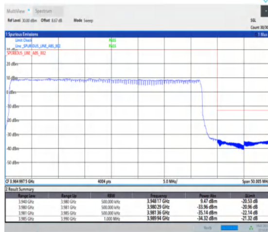
1-N77-3700-3980-PC1-30-40-H-3-DFT-PI2BPSK-Outer_Full-100@0-Ant1-1--PASS-see graph
