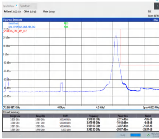
1-N77-3700-3980-PC1-30-30-H-2-DFT-PI2BPSK-Edge_1RB_Right-1@77-Ant1-1--PASS-see graph
