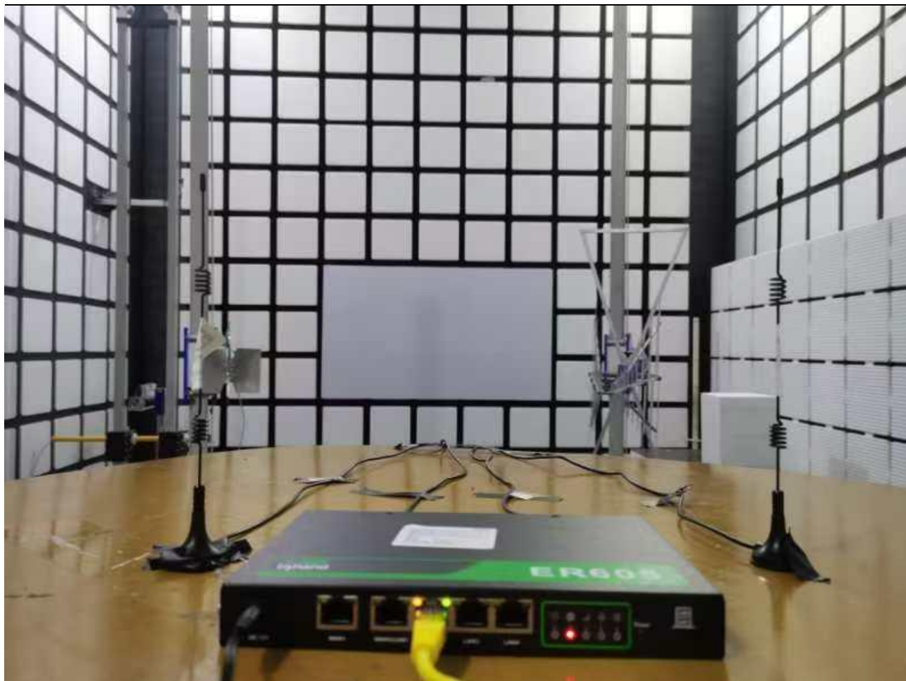
RF Radiated Test setup (RSE)
