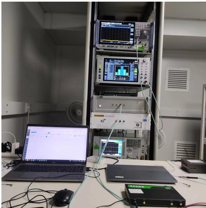
RF Conducted Test setup (WCDMA/LTE)
