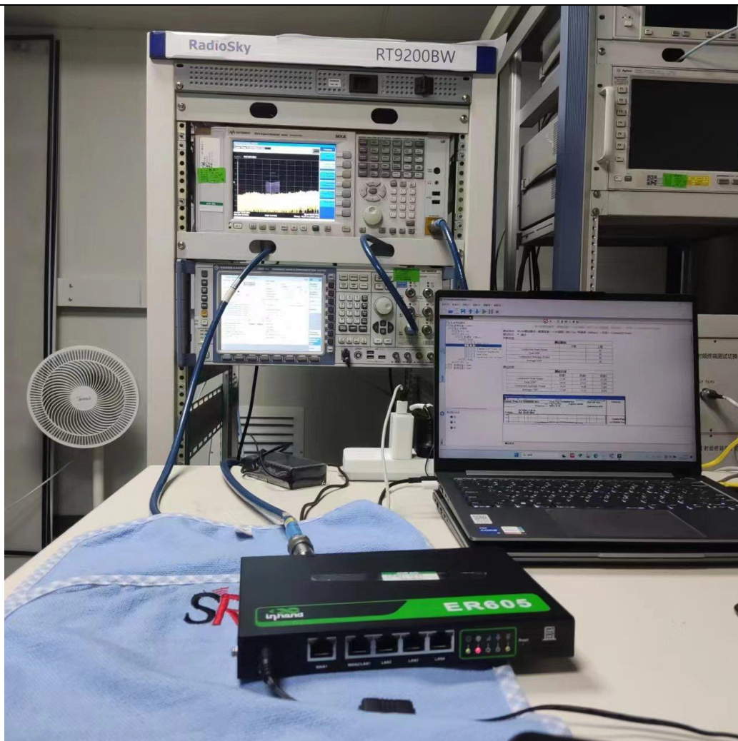
RF Conducted Test setup (WIFI)
