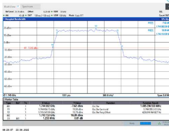
Band66-1.4MHz-QPSK-132322-6RB#0
