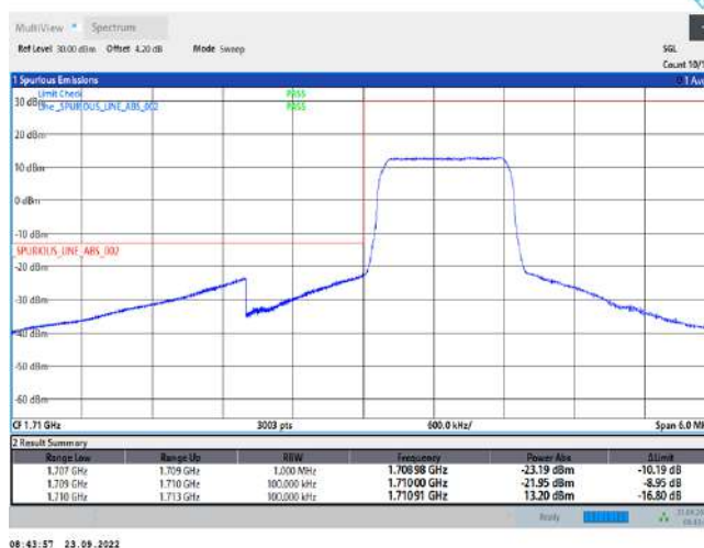
Band66-1.4MHz-QPSK-131979-6RB#0
