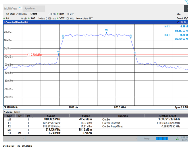
Band26-1.4MHz-QPSK-26740-6RB#0
