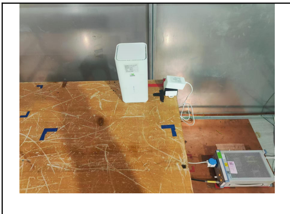
Power line conducted emission setup photo
