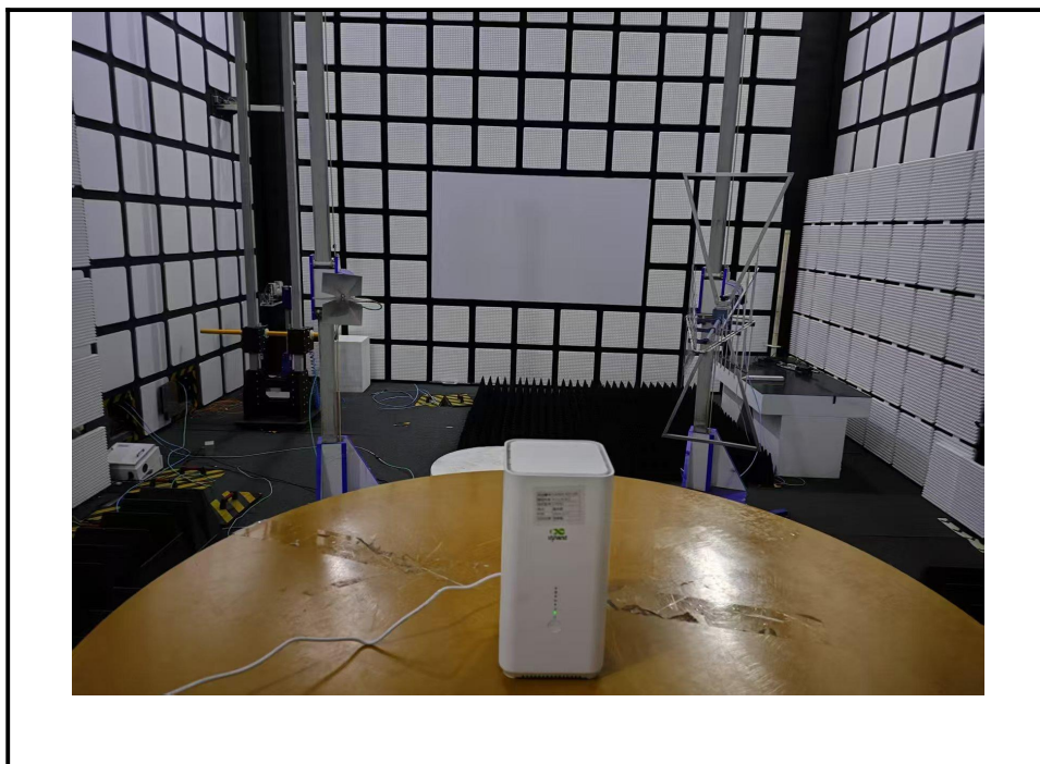
Radiated emission setup photo
