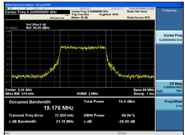
Mode:802.11ac VHT20 Frequency:5240MHz
