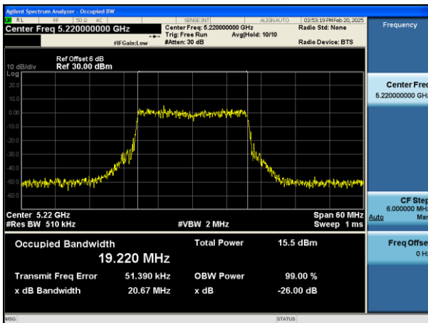
Mode:802.11ac VHT20 Frequency:5220MHz
