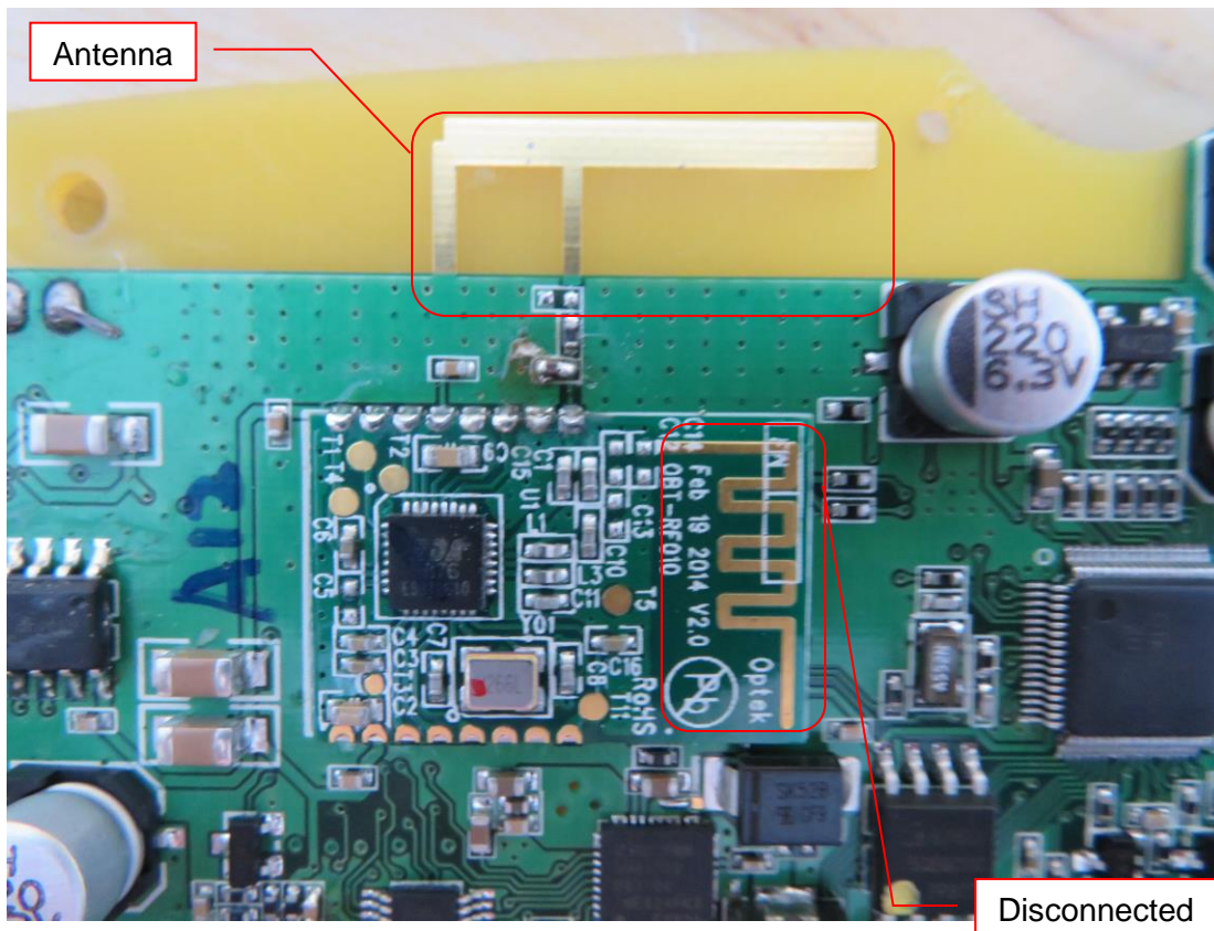
Details View of PCB
