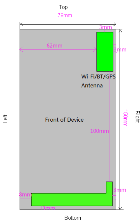
Mobile Hotspot Sides for SAR Testing
