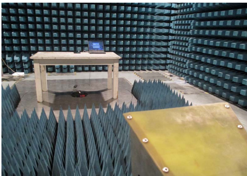
Radiated Emission of 1-6G
