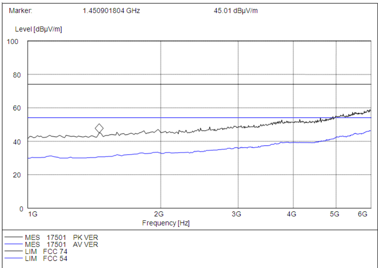
(Plot D: Test Antenna Vertical 1G – 6G)
