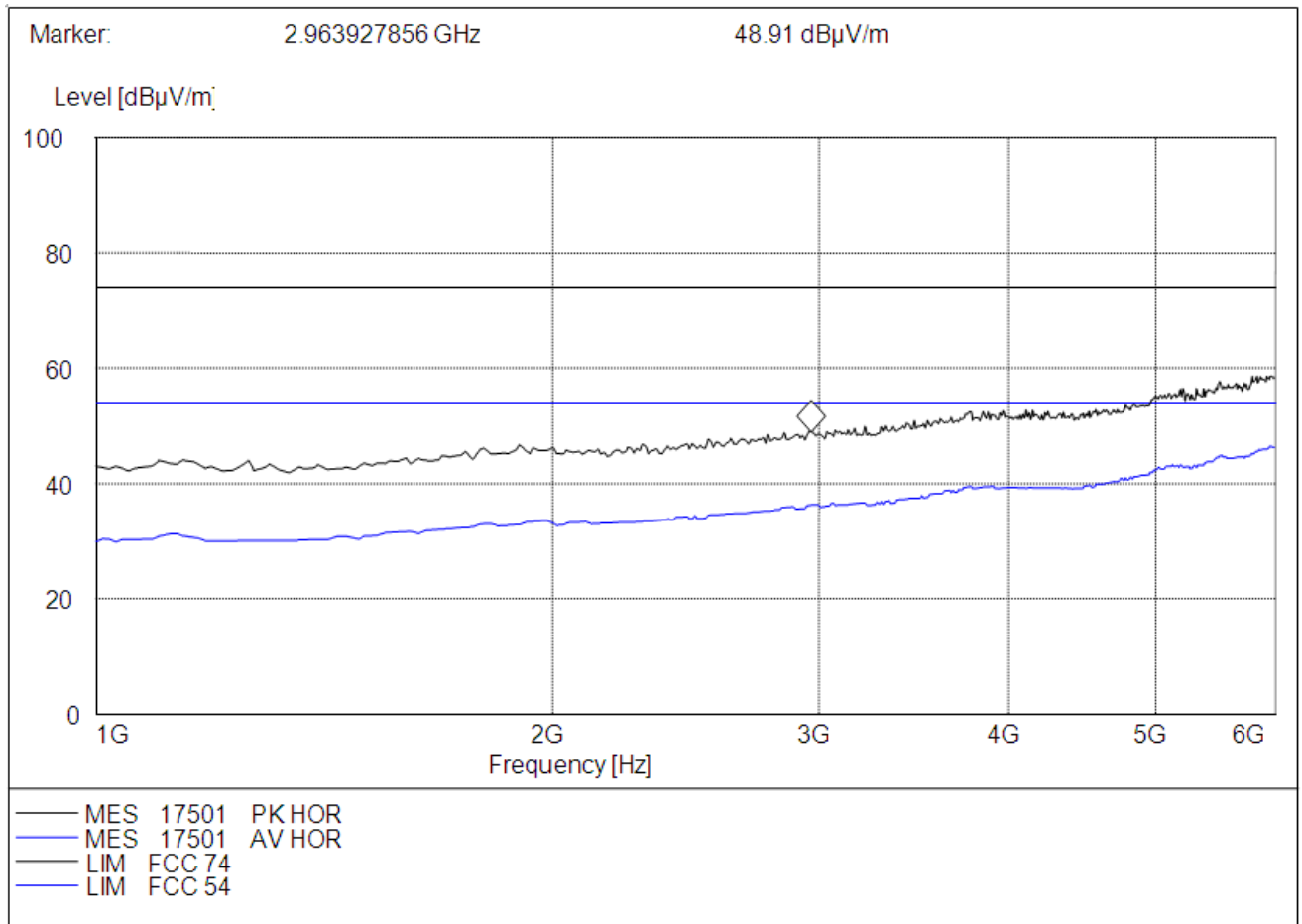
(Plot C: Test Antenna Horizontal 1G – 6G)
