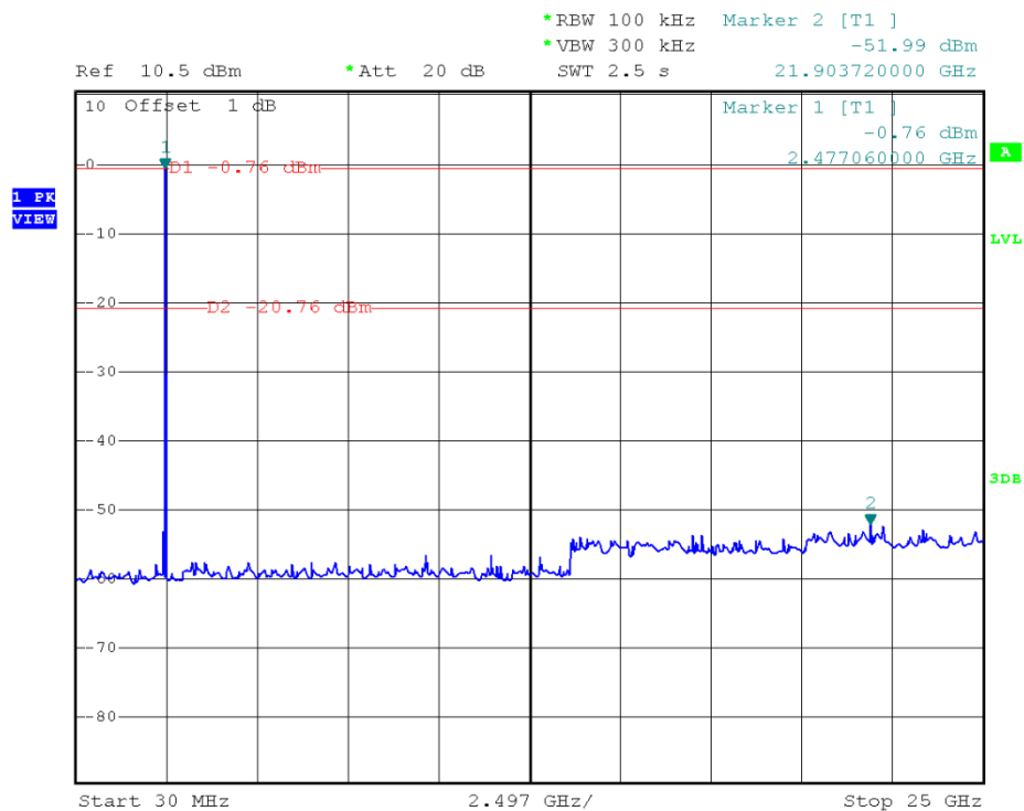
(Plot C: Channel = 78, 30MHz to 25GHz @ \pi/3 -DQPSK)
