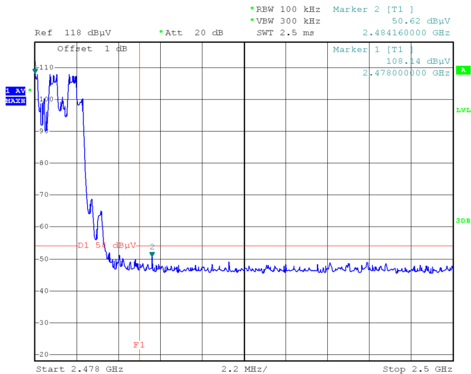
(Plot D2-1: Channel = 78 AVERAGE)
