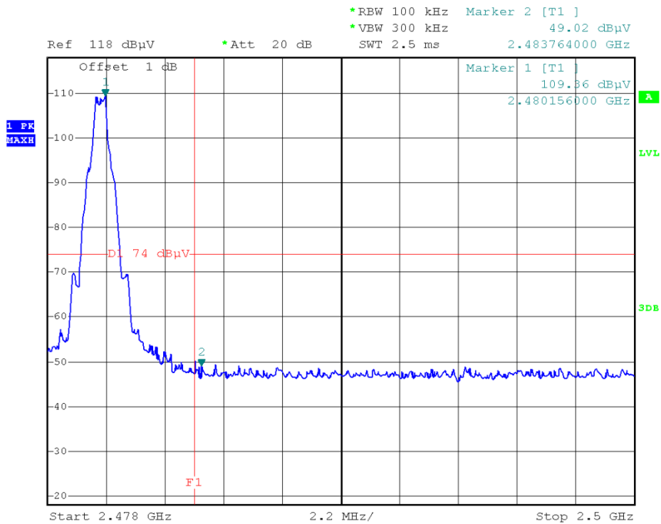
(Plot B1: Channel = 78 PEAK @ GFSK)
