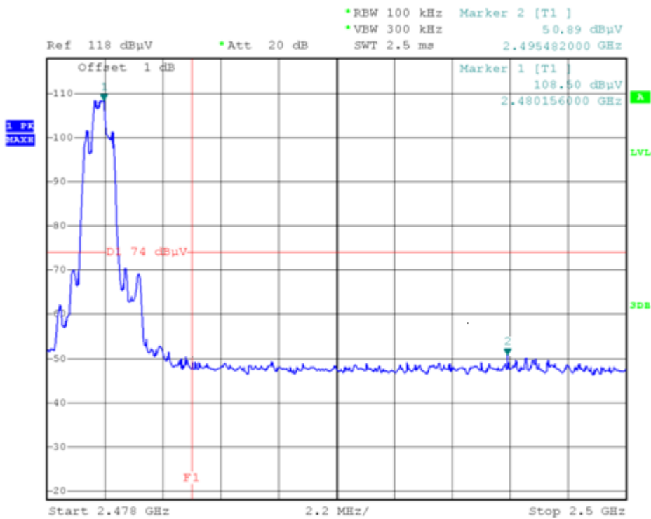
(Plot F1: Channel = 78 PEAK @ 8-DPSK Mode)
