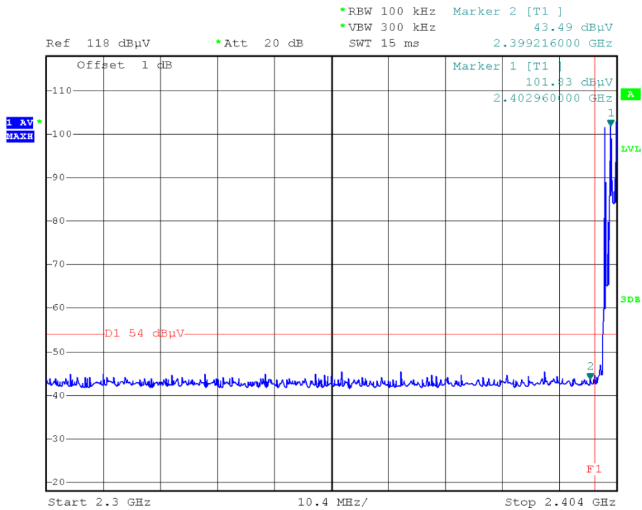
(Plot A2-1: Channel = 0 AVERAGE)
