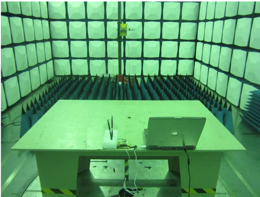
Radiated Emission – Rear View (Above 1G Distance 3m)
