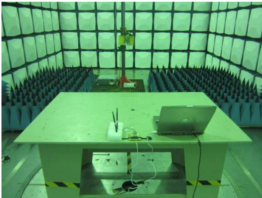
Radiated Emission – Rear View (Above 1G Distance 1.5m)
