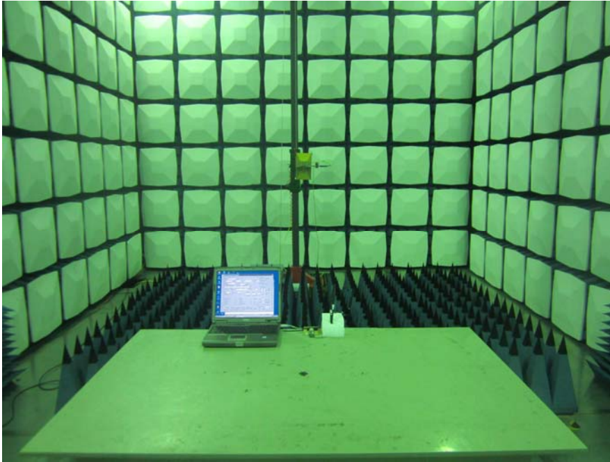
Radiated Emission – Front View (Above 1G Distance 3m)
