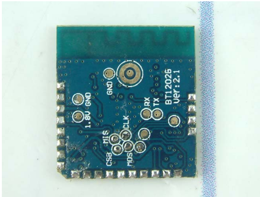
RF Module view side 2
