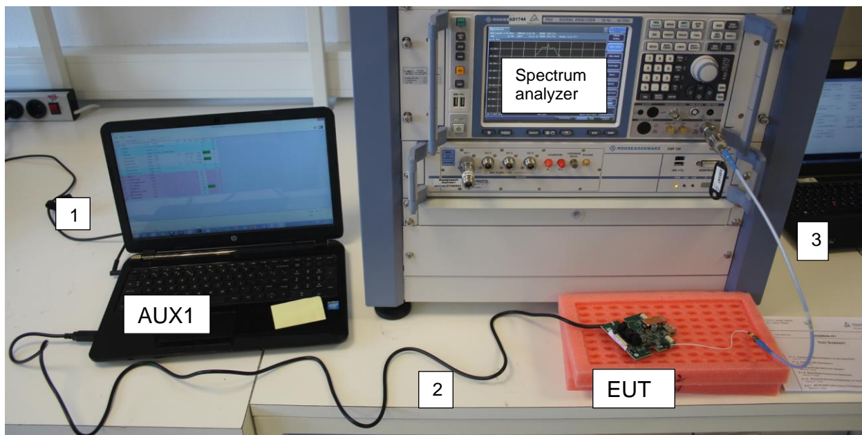
Figure 2b: Test Setup Photos – conducted tests and programming
