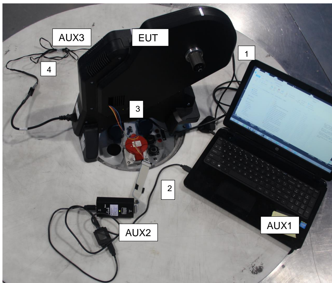
Figure 2: Test Setup Photos – radiated tests and programming
