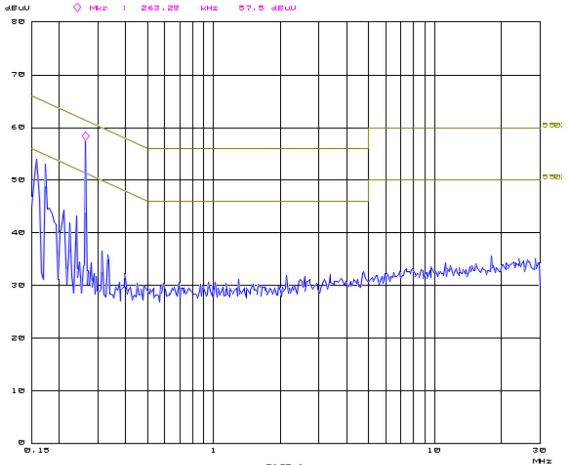
Plot of the AC Power-line Conducted emissions on N
