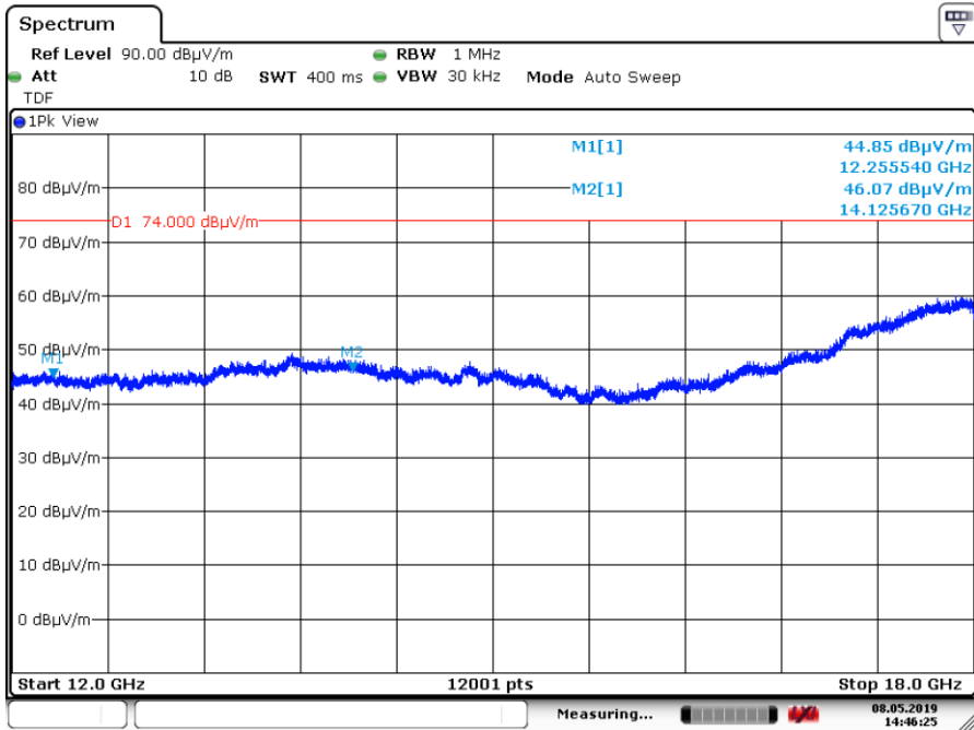
Plot of the emissions at 2403 MHz in the range 12 – 18 GHz, Antenna Vertical, Peak values shown (Reduced Video Bandwidth used)
