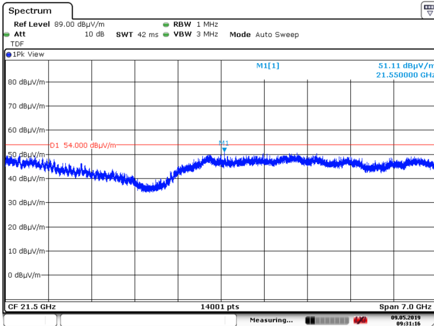
Plot of the emissions at 2403 MHz in the range 18 – 25 GHz, Antenna Horizontal, Peak values shown
