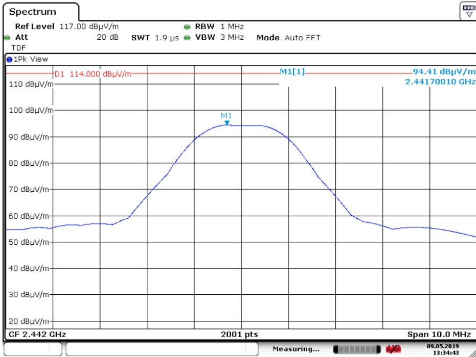
Plot of the emissions at 2442 MHz, Vertical polarization, Peak value of the fundamental
