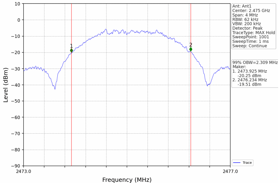
2.4g_HCH_2475MHz_Ant1_NTNV
