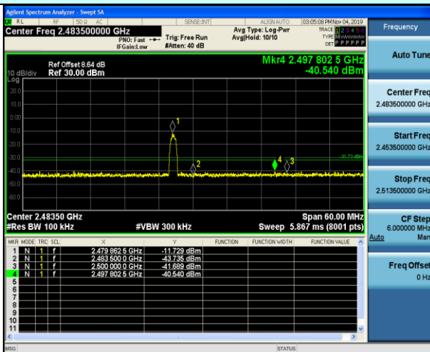
No-hopping mode
