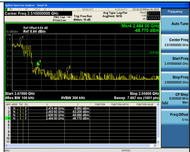
Hopping mode
