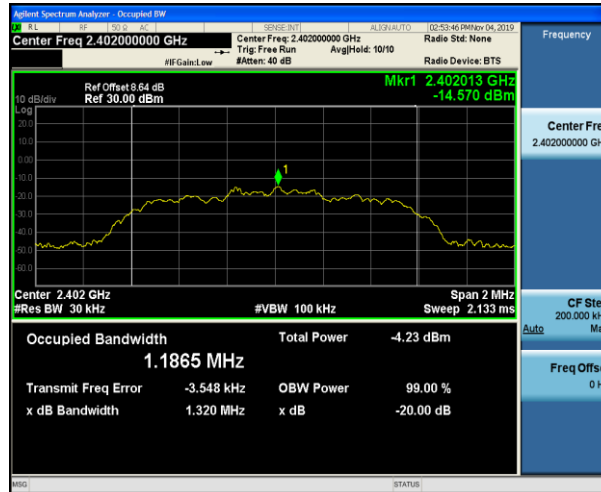
Lowest channel
