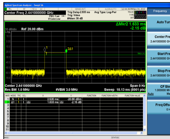
3DH3
