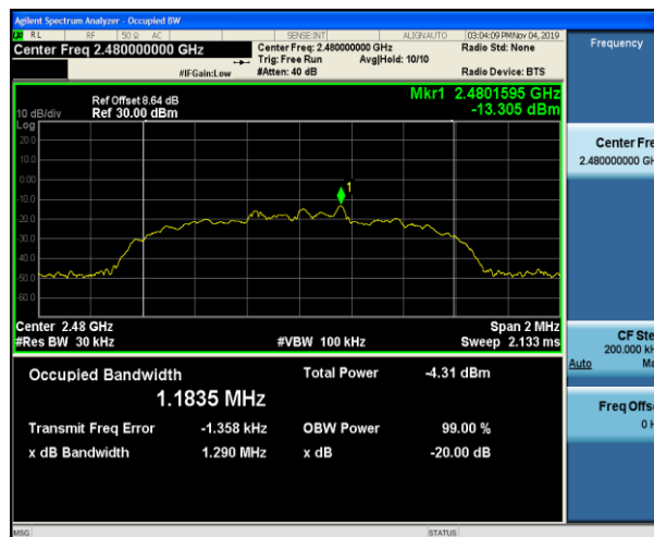
Highest channel
