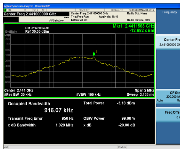
Middle channel
