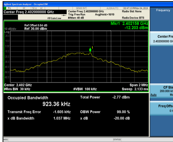
Lowest channel
