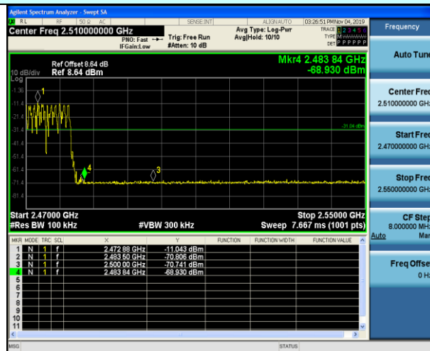
Hopping mode
