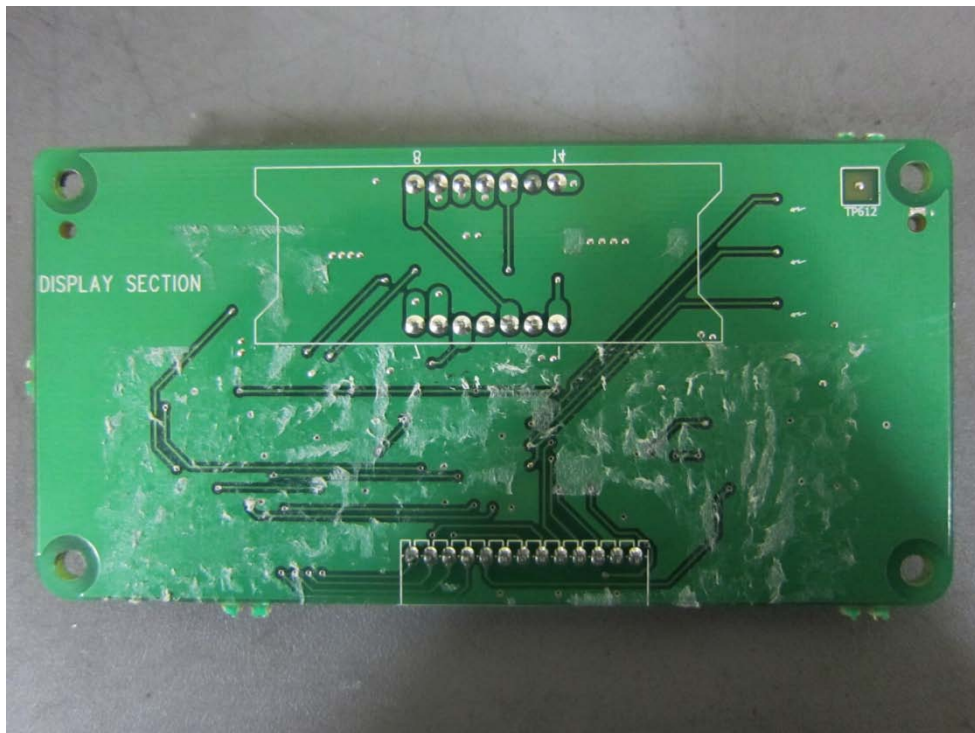
LED Board_Rear
