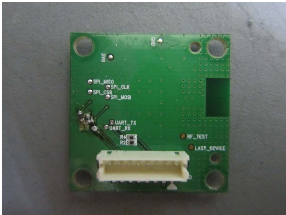
RF Board_Rear
