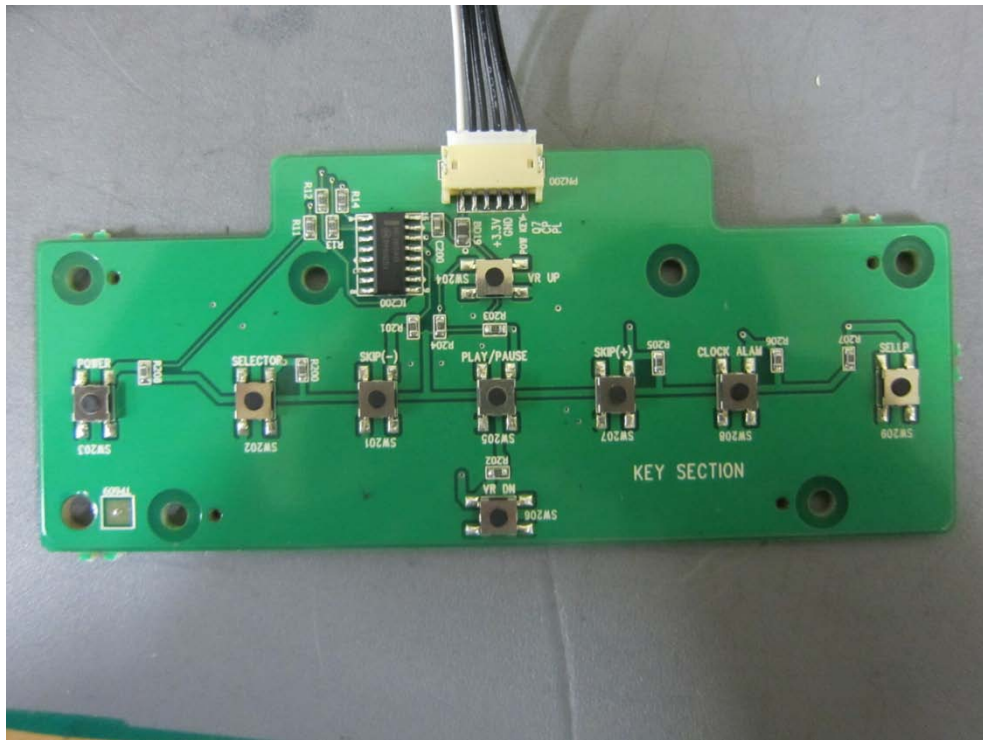
Key Board_Front
