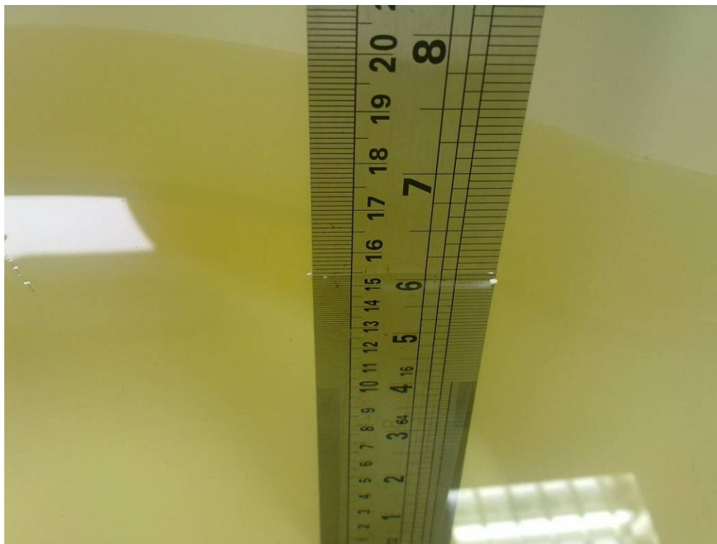
Liquid depth in the Flat Phantom (1900MHz)
