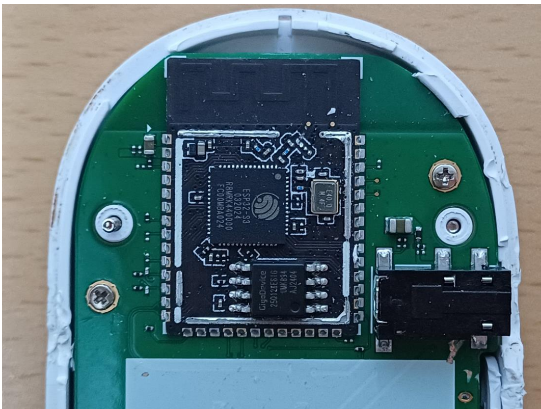
RF Module(Shelid can Remove) - Front
