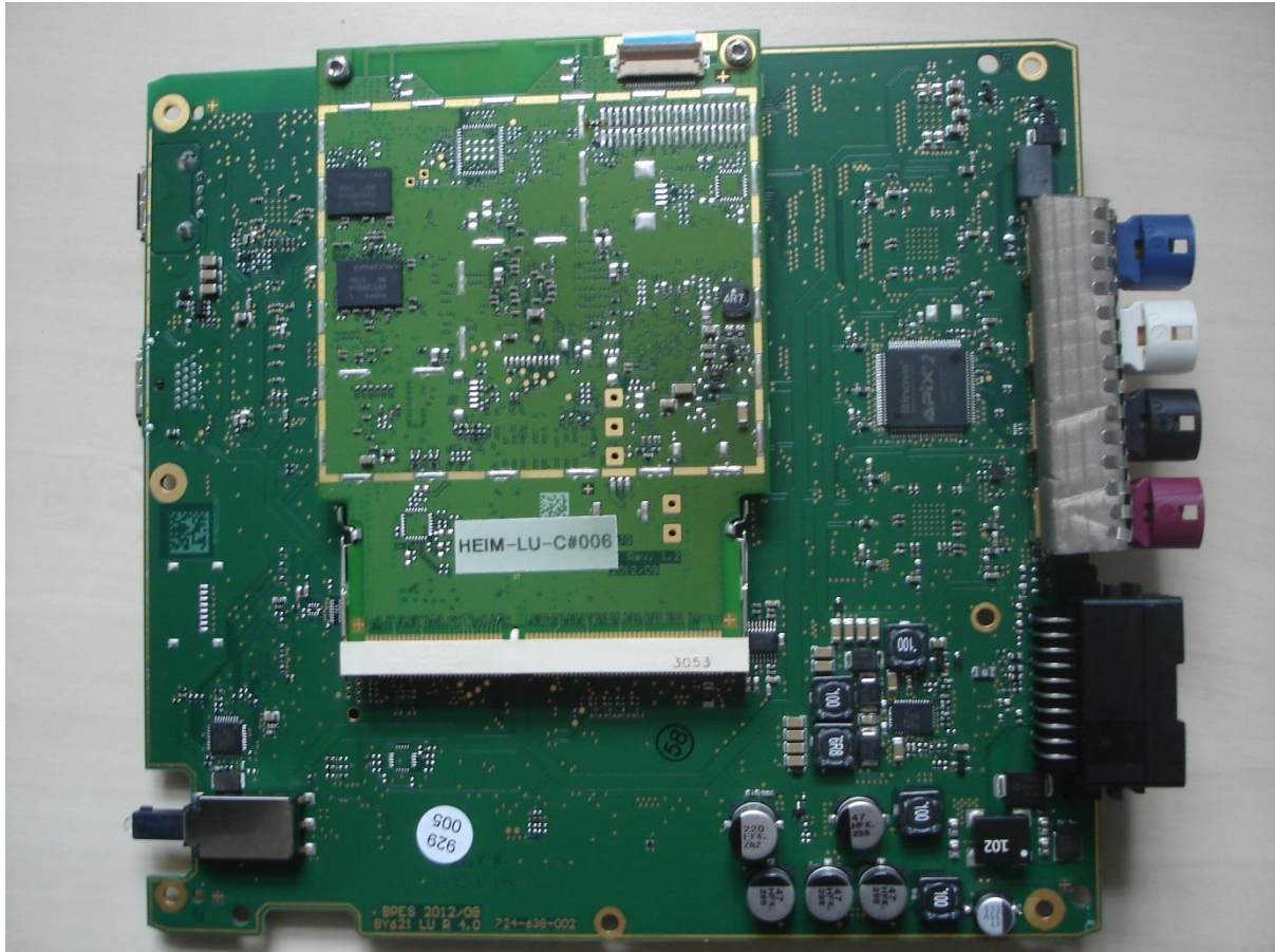
Ribbon cable between Heim board and loader PCB
