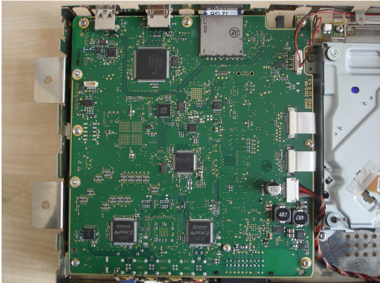
Loader PCB Top View
