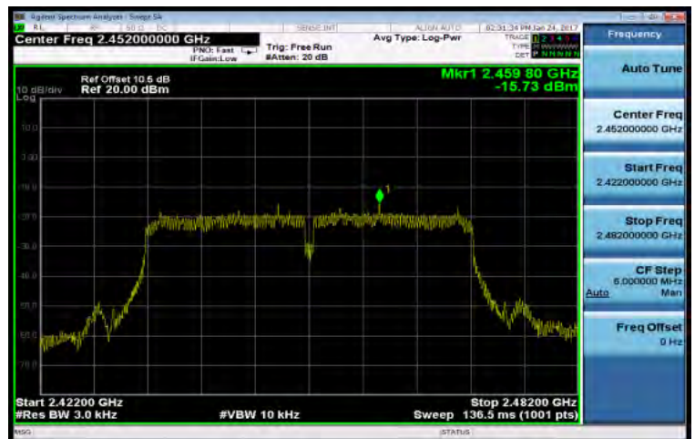
802.11n_40 CH-High
