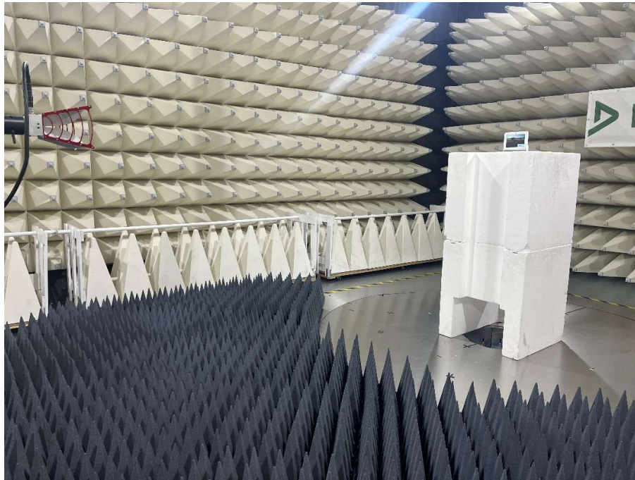
5. Radiated Emission Test Setup High range 1
