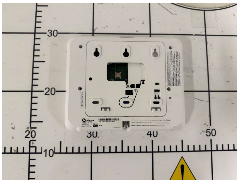
2. Bottom View of the DUT
