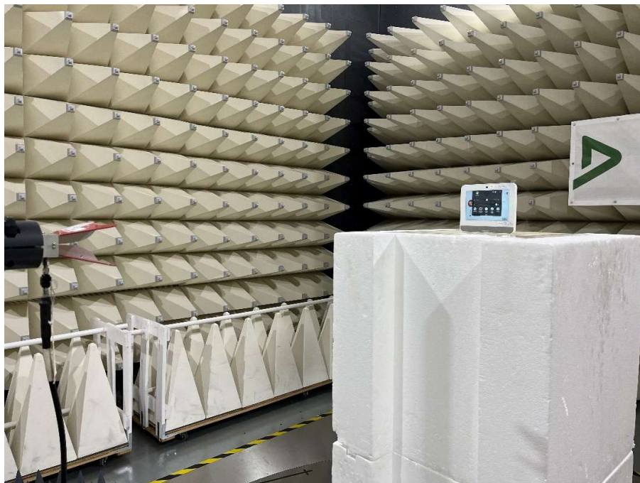
6. Radiated Emission Test Setup High range 2
