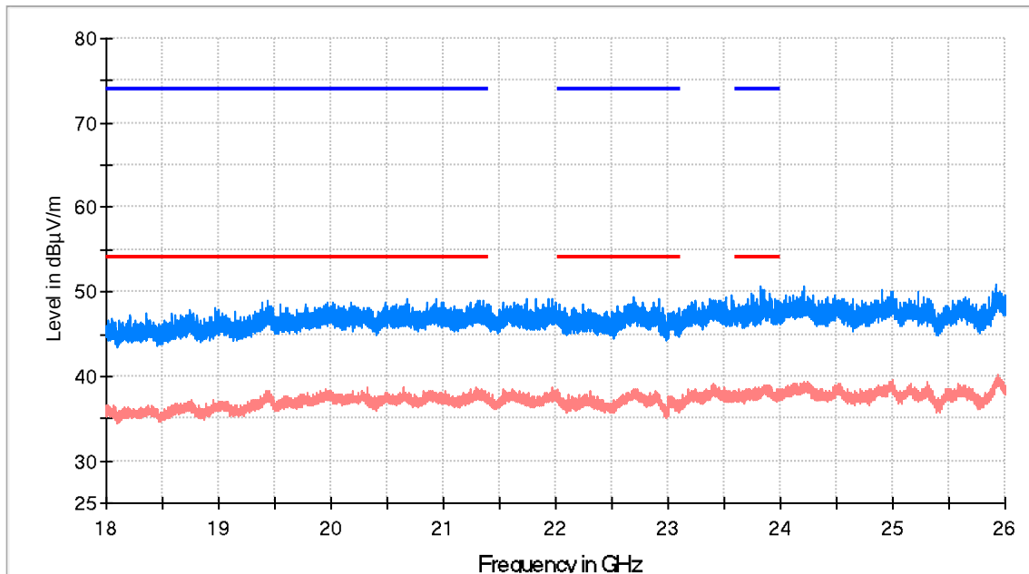
RF_FCC_15.247_E Field_18GHz_26GHz(SAC2)
