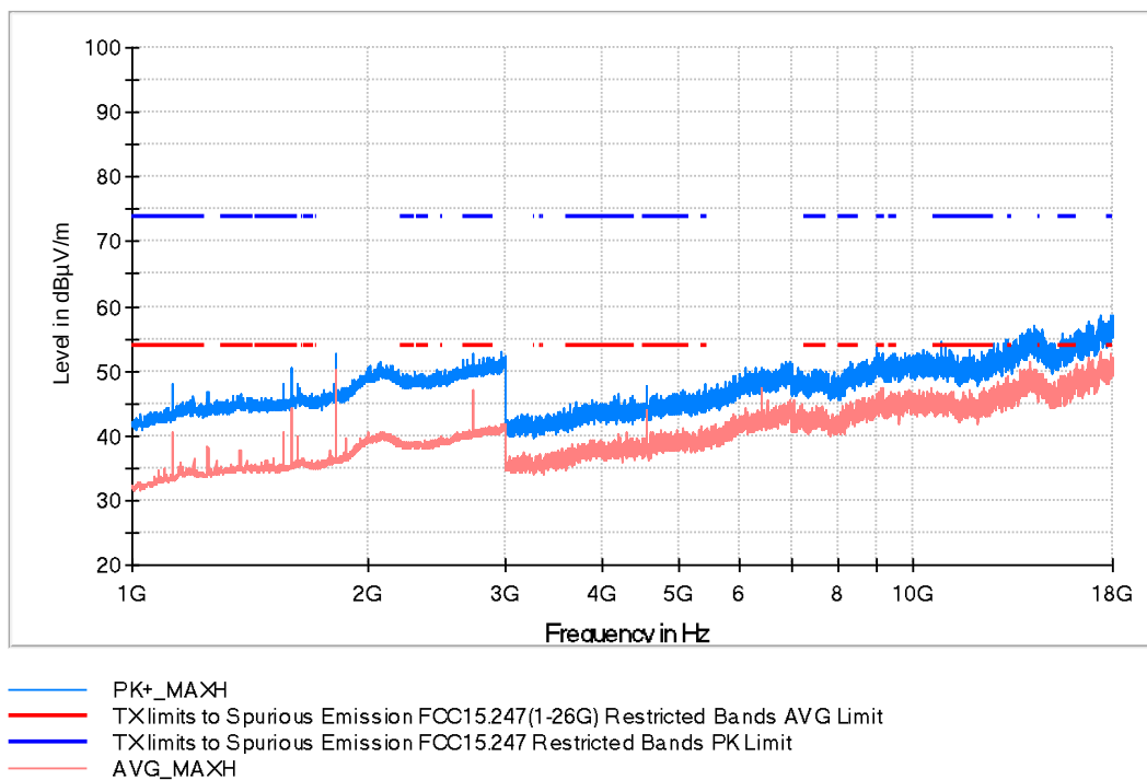
RF_FCC_15.247_E Field_1GHz_18GHz_HPFF(SAC2)
