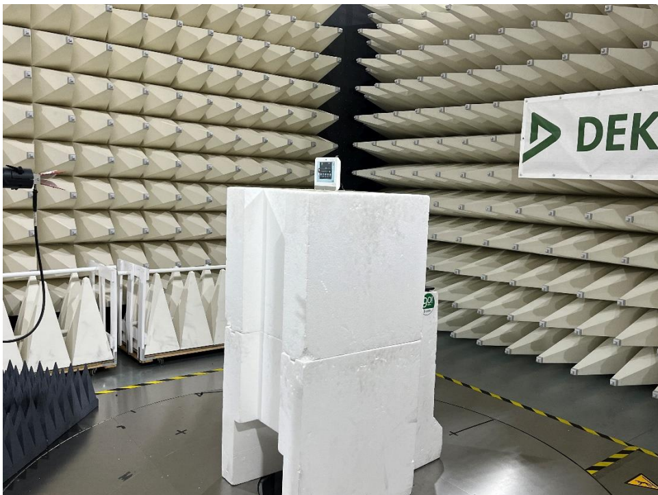
6. Radiated Emission Test Setup High range 2
