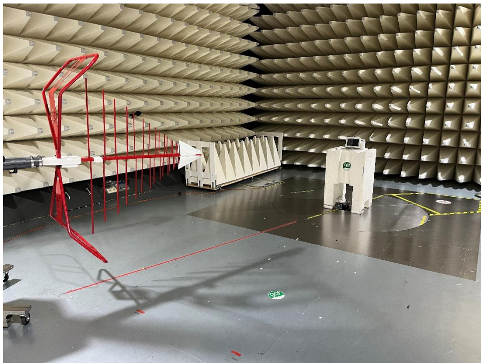
4. Radiated Emission Test Setup Low Range
