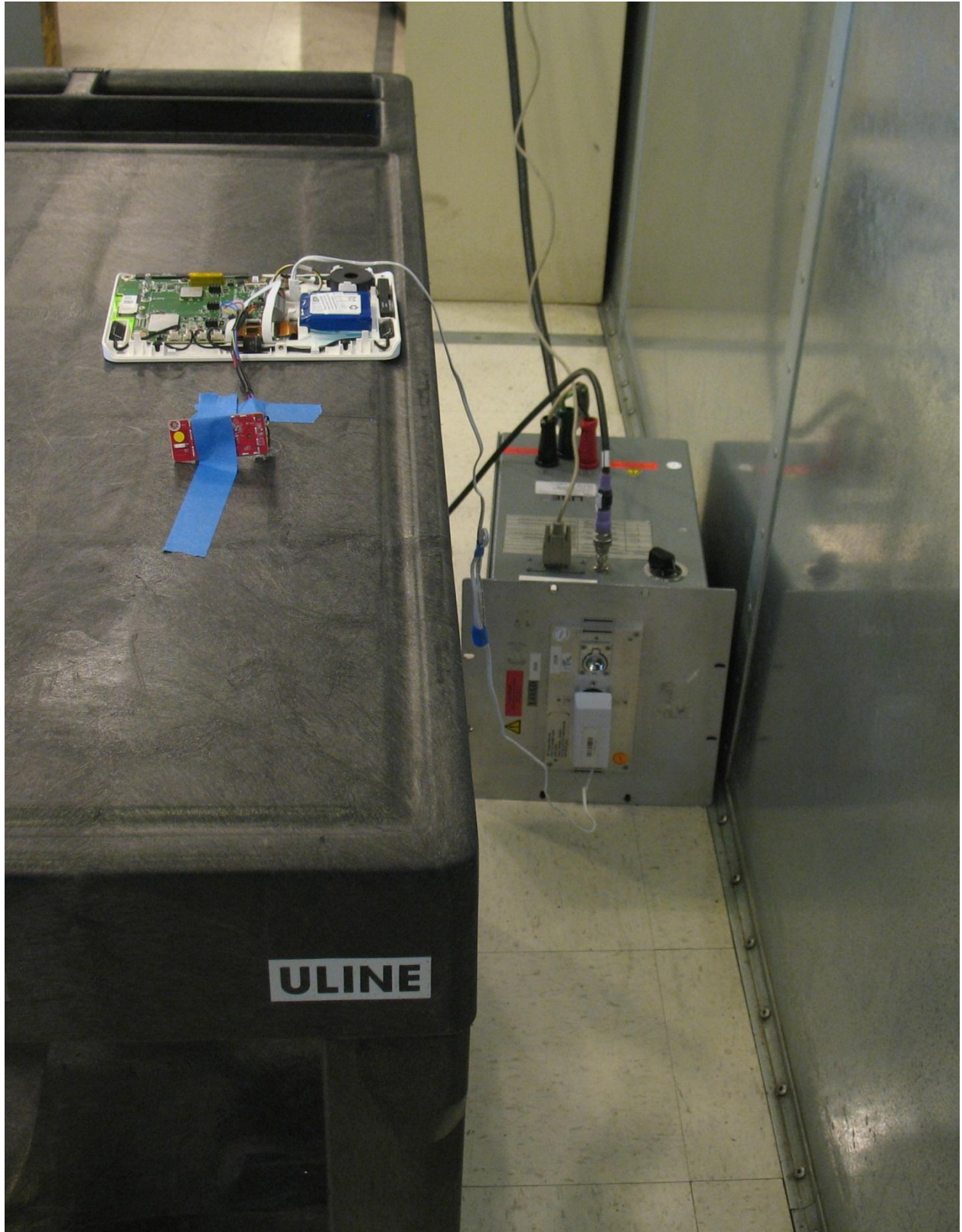
Conducted Emissions
