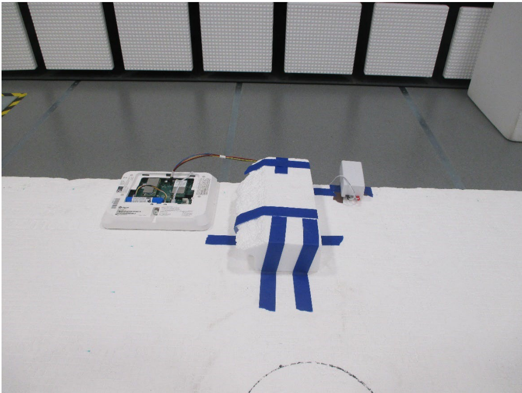
RADIATED SETUP BELOW 30MHz: BACK
