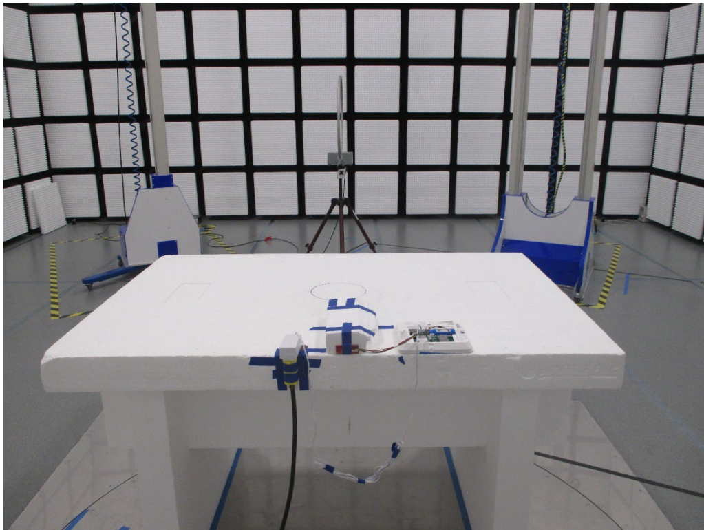
RADIATED SETUP BELOW 30MHz: 90 Deg
