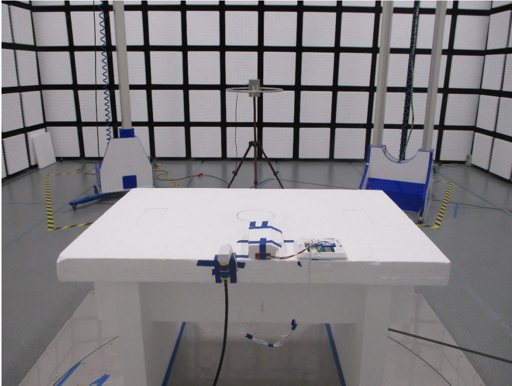
RADIATED SETUP BELOW 30MHz: FLAT
