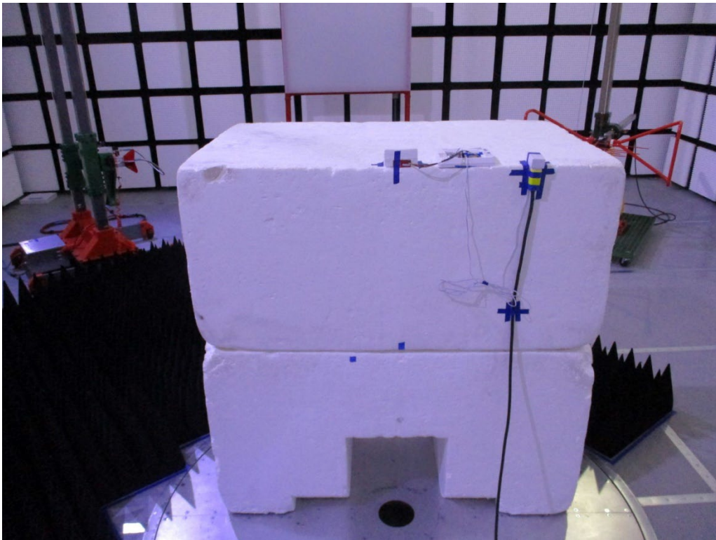
RADIATED SETUP ABOVE 1GHz: REAR
