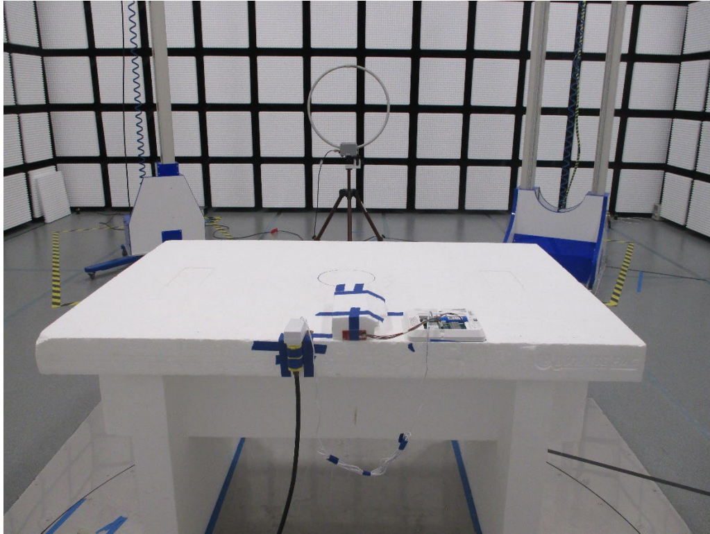
RADIATED SETUP BELOW 30MHz: 0 Deg
