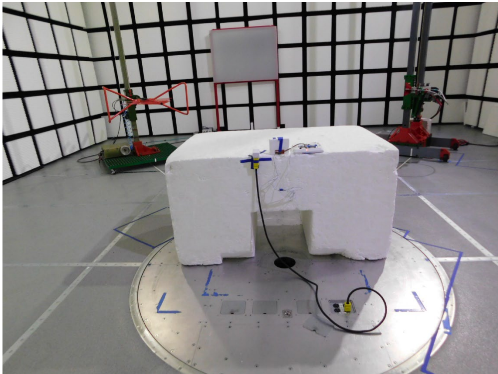
RADIATED SETUP BELOW 1GHz: REAR
