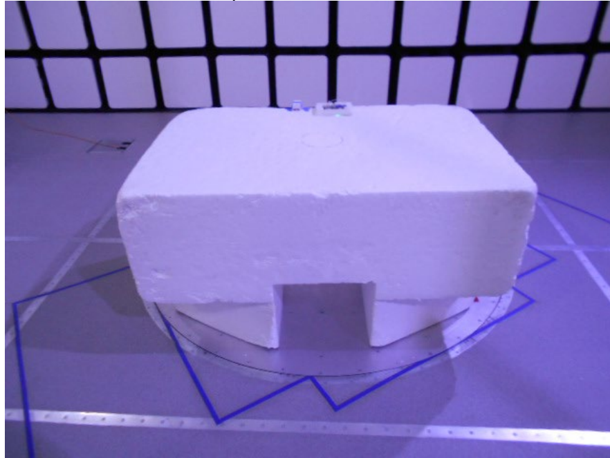
Radiated Emissions Setup 30-1000MHz
