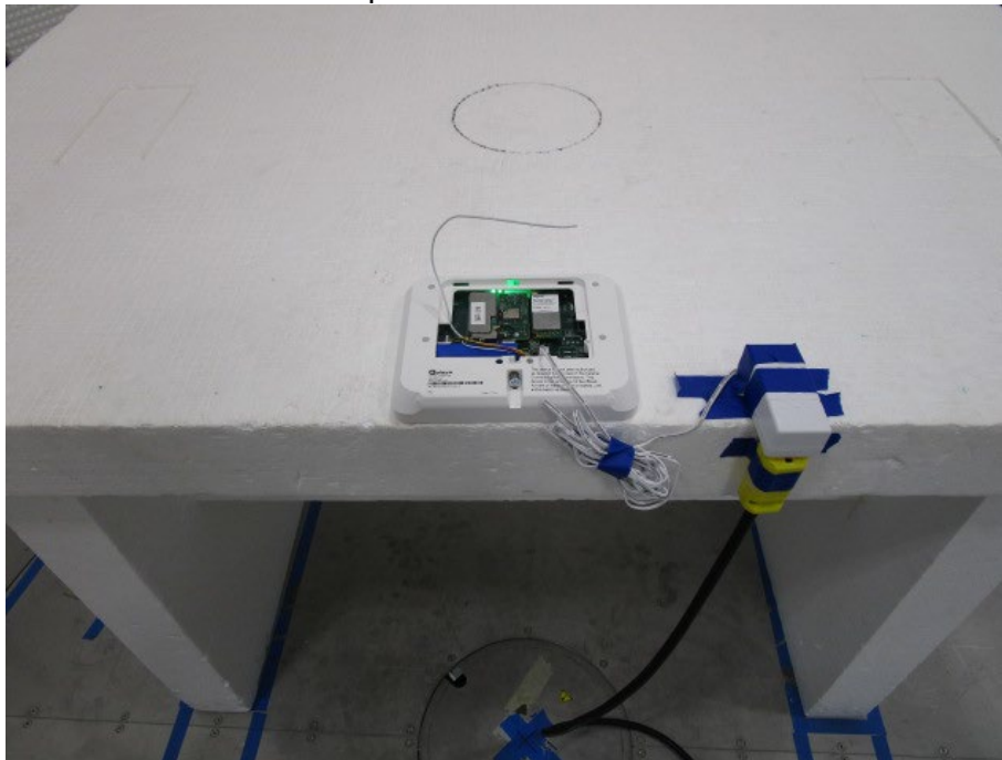
Radiated Emissions Setup X-Orientation
