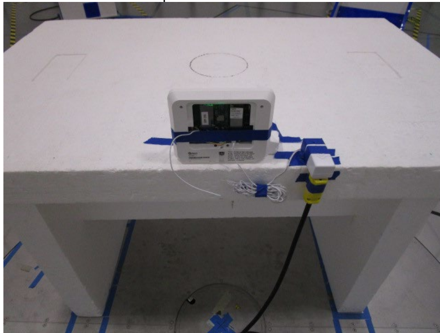
Radiated Emissions Setup Y-Orientation
