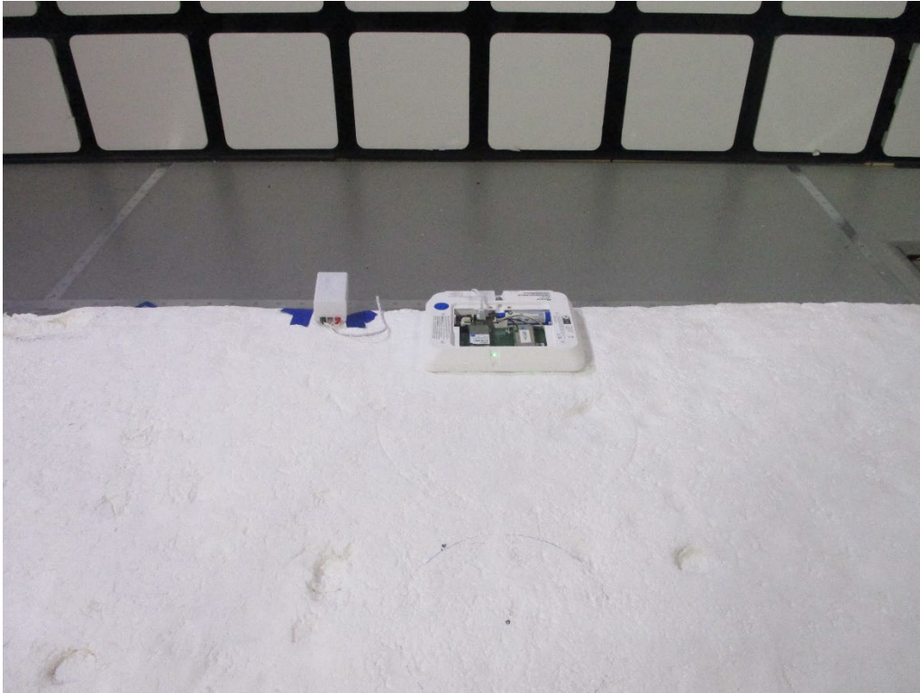
RADIATED SETUP BELOW 1GHz: FRONT
