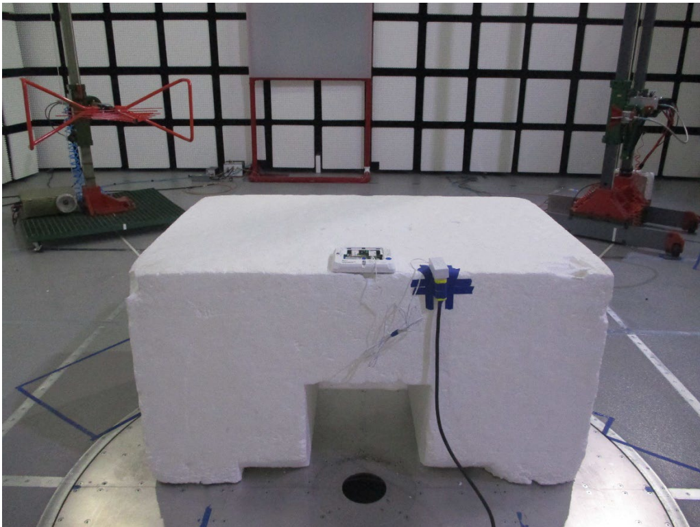
RADIATED SETUP BELOW 1GHz: REAR
