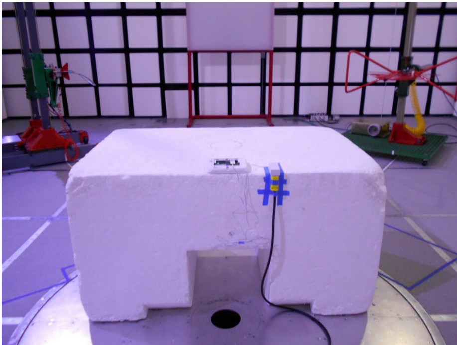
BL1G RADIATED SPURIOUS EMISSIONS BACK
