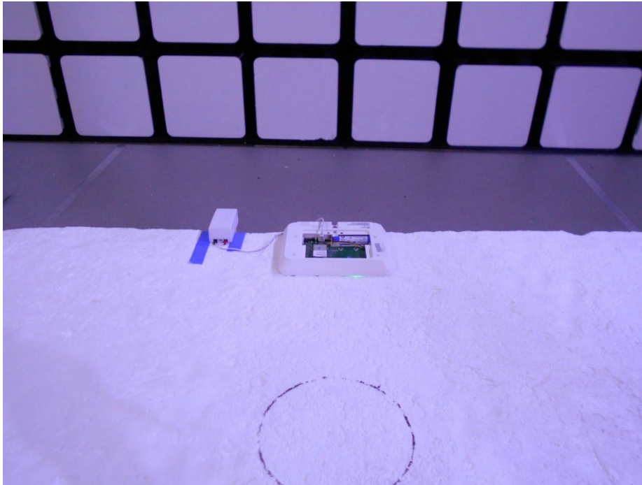
BL1G RADIATED SPURIOUS EMISSIONS FRONT
