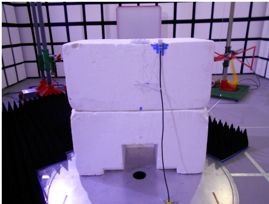
A1G RADIATED SPURIOUS EMISSIONS BACK
