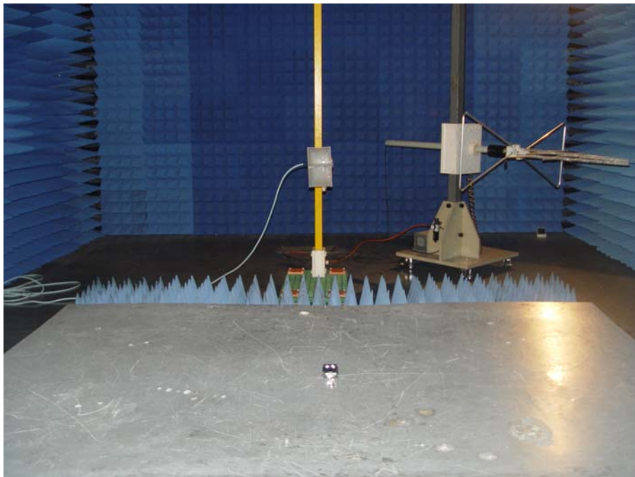
Radiated emissions test > 1GHz
