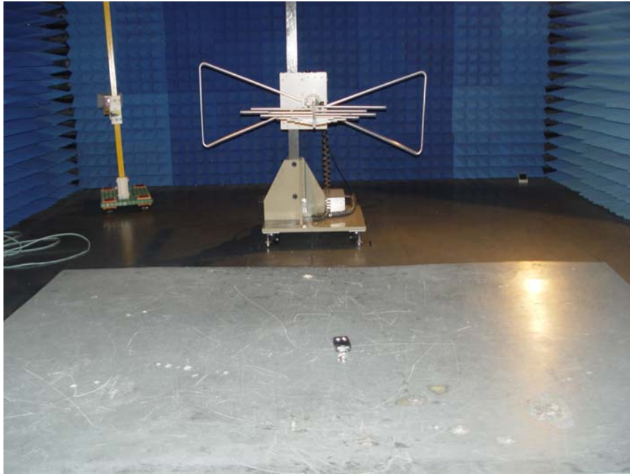
Radiated emissions test 30MHz- 1GHz
