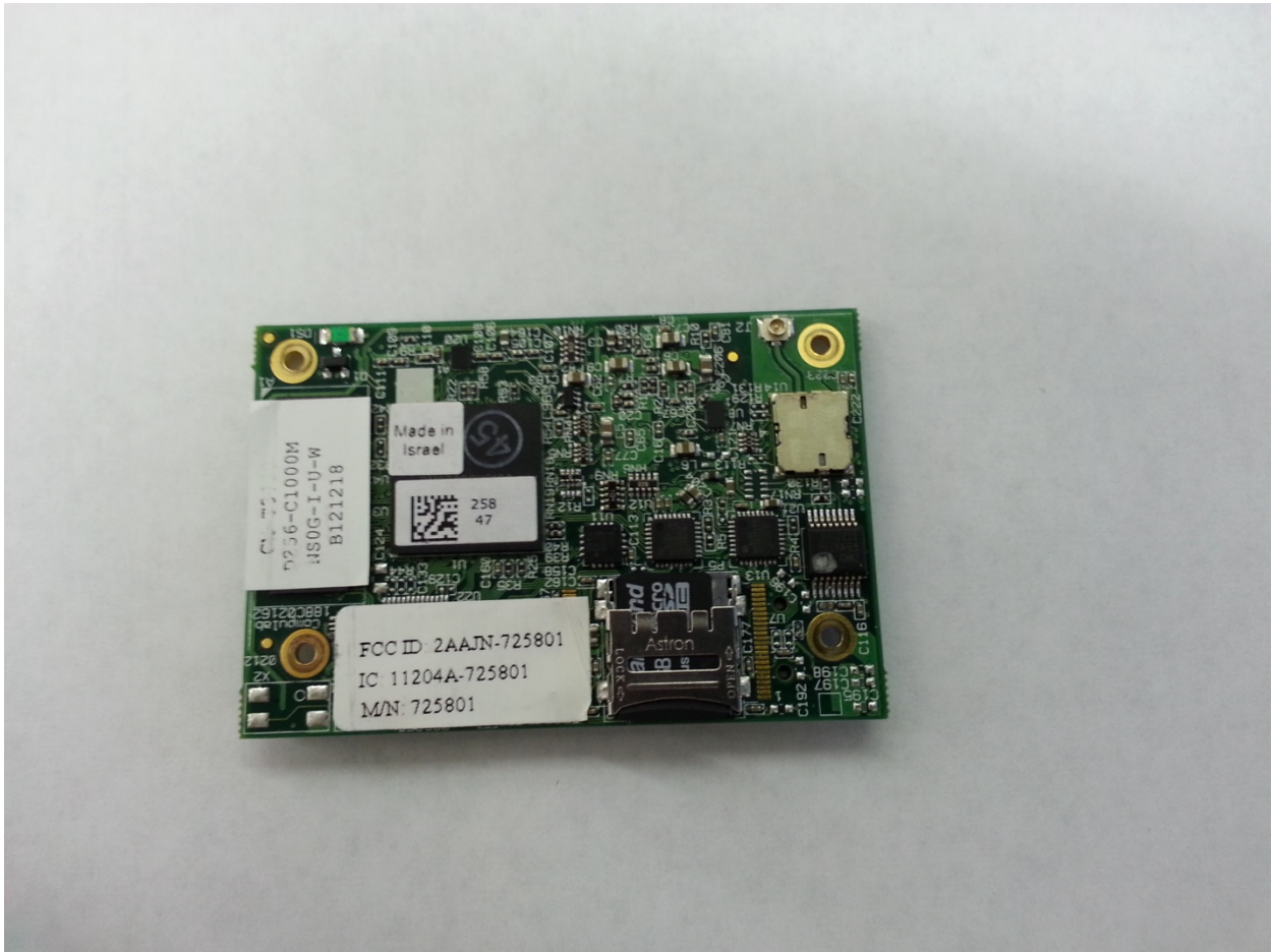
Daughter Board Frontside.
