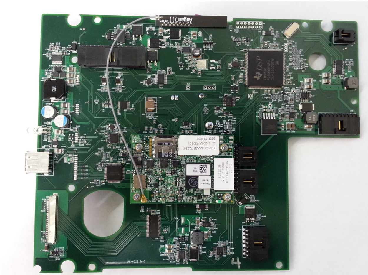
Base Board Frontside with Daughter board.
